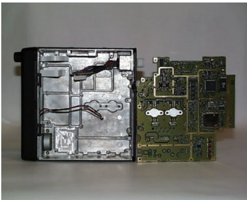
PC Board Bottom View
