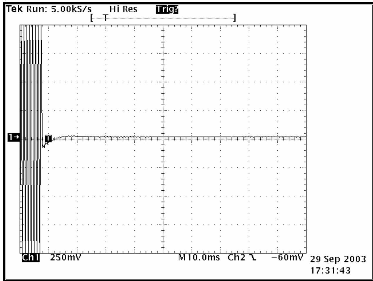
PLOT 13-3: TRANSIENT FREQUENCY BEHAVIOR – 160.15 MHZ; HIGH POWER; NARROW BAND; CARRIER ON TIME
