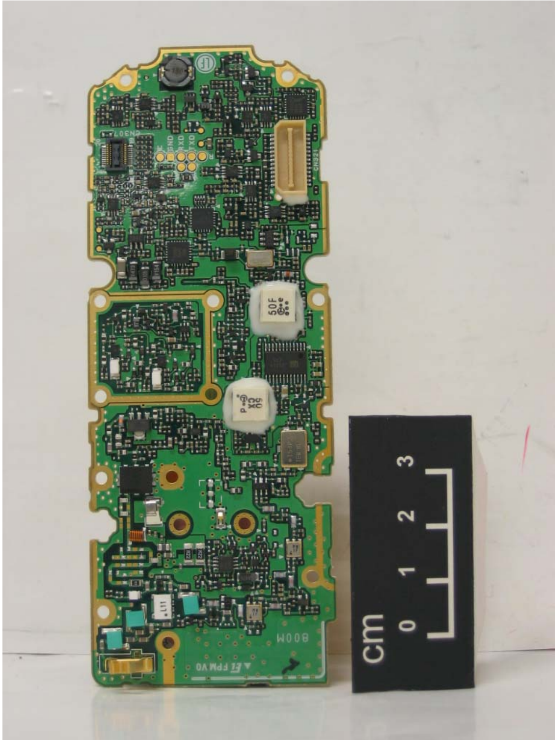
TXRX UNIT
