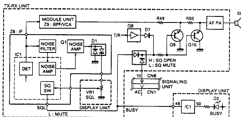
Fig. 3 Squelch circuit
