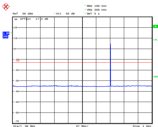
LTE Band 12 5MHz CH-High 30MHz~1GHz
