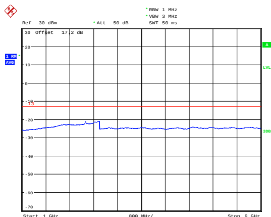
LTE Band 12 5MHz CH-Low 1GHz~9GHz
