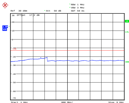
LTE Band 12 5MHz CH- Middle 1GHz~9GHz
