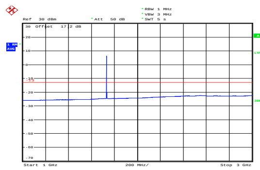
LTE Band 4 1.4MHz CH-Middle 1GHz~3GHz
