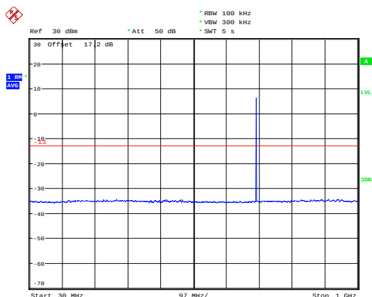
LTE Band 12 5MHz CH-Low 30MHz~1GHz
