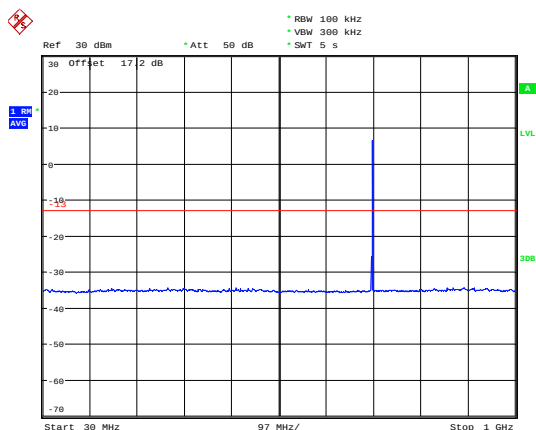
LTE Band 12 5MHz CH- Middle 30MHz~1GHz
