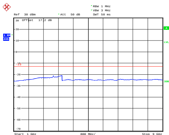
LTE Band 12 5MHz CH-High 1GHz~9GHz
