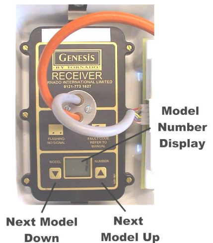
Dia. 14 – The Receiver in Position in the Boat
