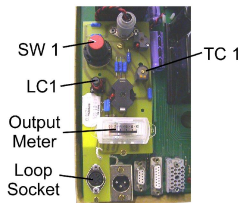
Dia. 15 Loop Output Board
