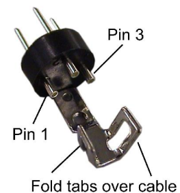
Dia. 10 – Inside the Loop Plug
