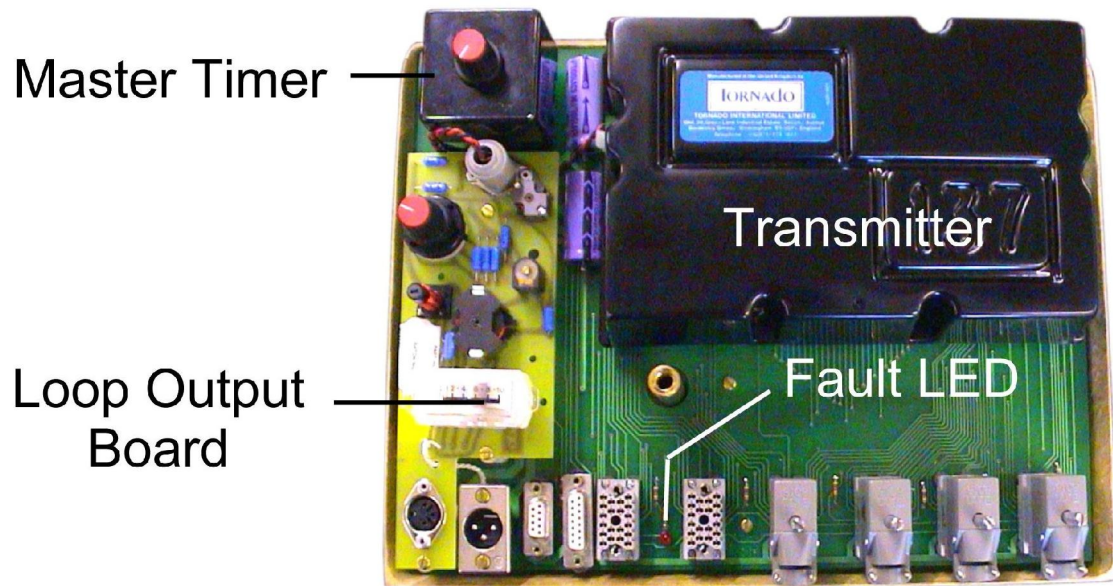
The Transmitter Mother Board The Transmitter The Loop Output Board The Master Timer
