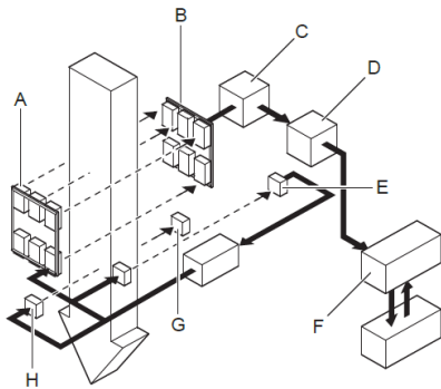
Fig. 2 A: Transmitters B: Receivers C: Amplifier D: A/D E: Reference detector F: Milk flow memory G: Blood sensor H: Transmitter
