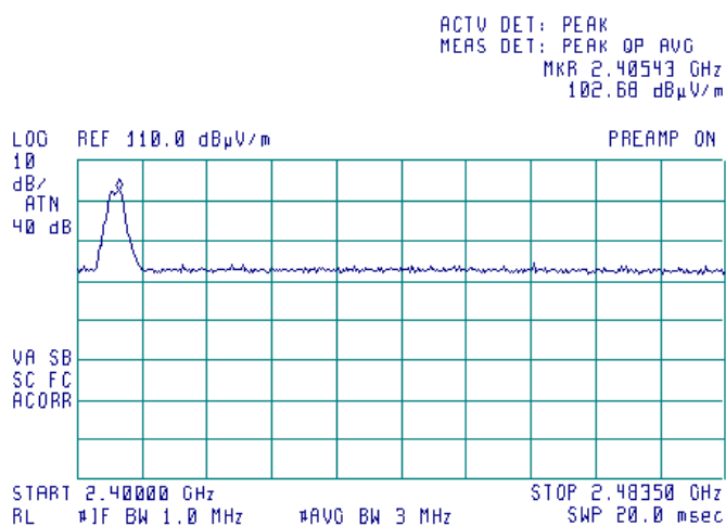
Plot 7.1.14 Radiated emission measurements from 2.4 to 2.4835 GHz
