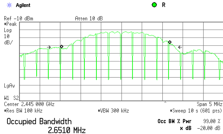
Plot 7.4.2 Occupied bandwidth test result at mid frequency
