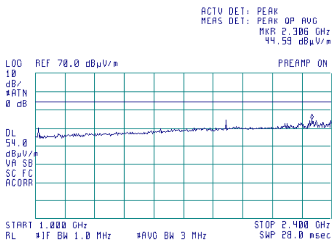
Plot 7.1.12 Radiated emission measurements from 1.0 to 2.4 GHz
