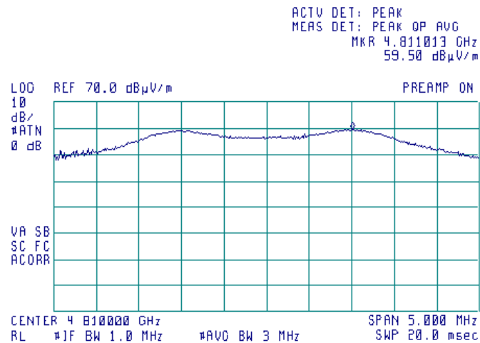
Plot 7.1.25 Radiated emission measurements at the second harmonic at low frequency
