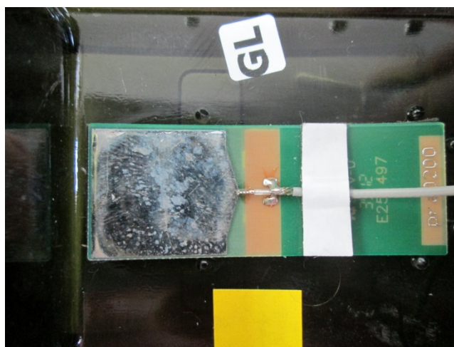
Photograph 7.3.1 Antenna assembly
