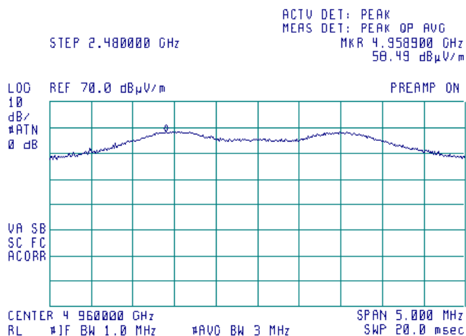
Plot 7.1.29 Radiated emission measurements at the second harmonic at high frequency
