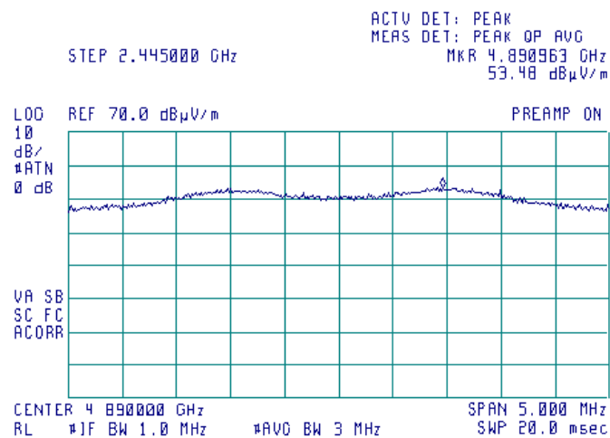
Plot 7.1.27 Radiated emission measurements at the second harmonic at mid frequency
