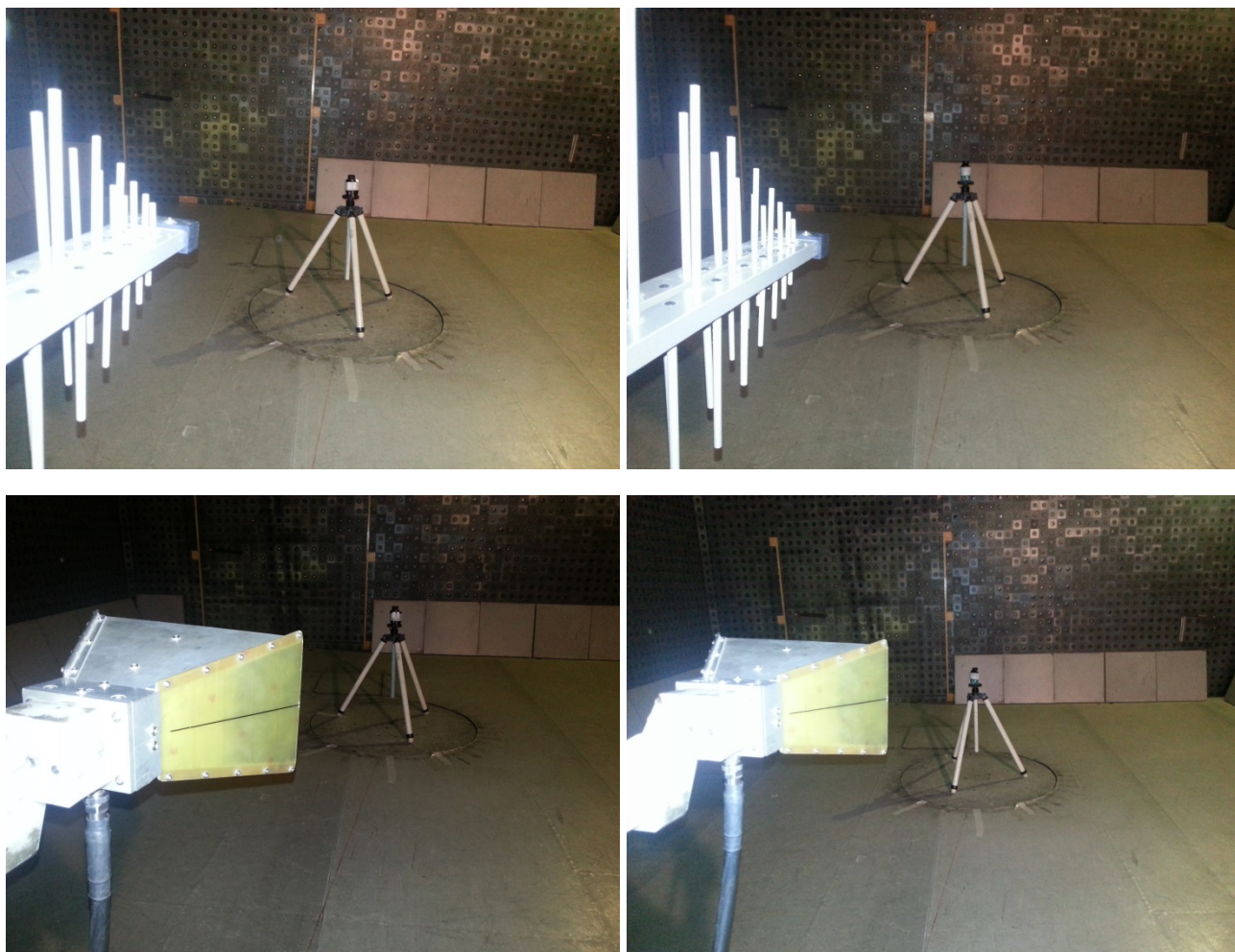
Photograph 8.1.1 Setup for radiated emission measurements
