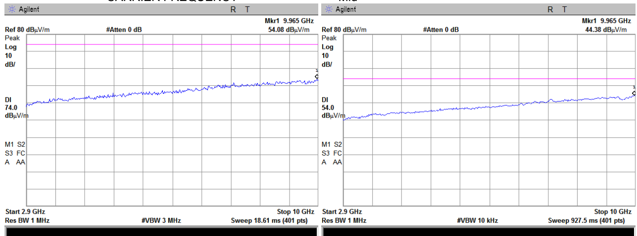
Plot 7.1.33 Radiated emission measurements from 2.9 to 10 GHz
