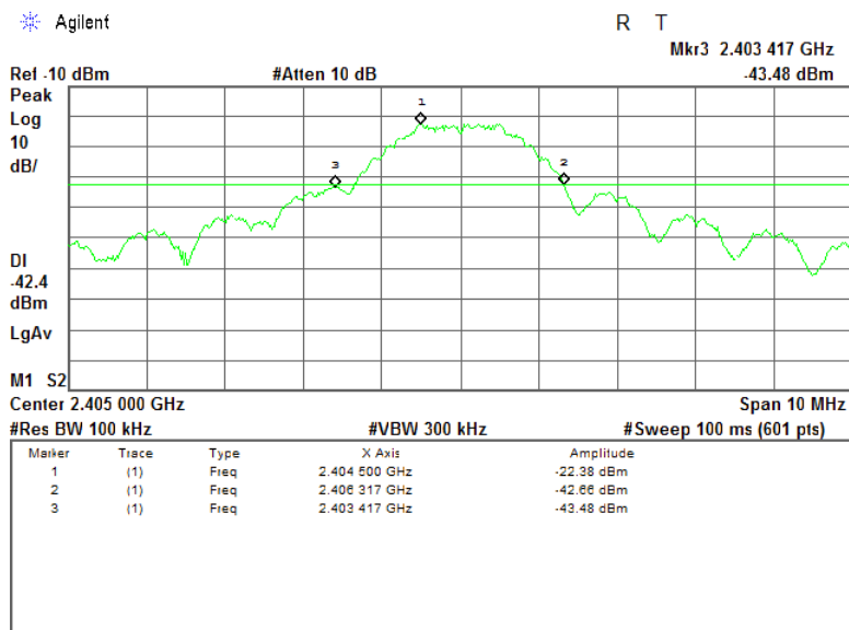
Plot 7.2.2 Low band edge frequency
