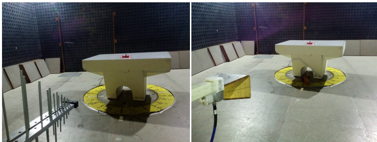
Photograph 8.1.1 Setup for radiated emission measurements
