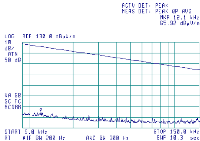
Plot 7.1.20 Radiated emission measurements from 9 to 150 kHz
