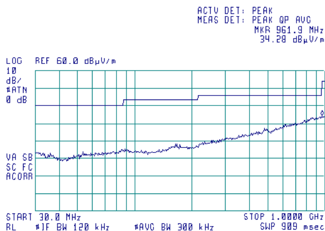
Plot 7.1.26 Radiated emission measurements from 30 to 1000 MHz
