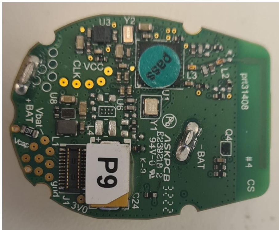
PCBA – Bottom side view
