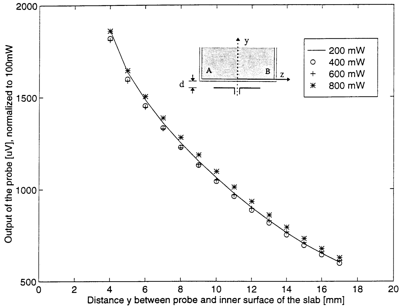
Fig. 2a. Test for square-law behavior at 840 MHz: Variation of the output voltage (proportional to |E_i|^2 ) for different radiated powers normalized to 0.1 W.
