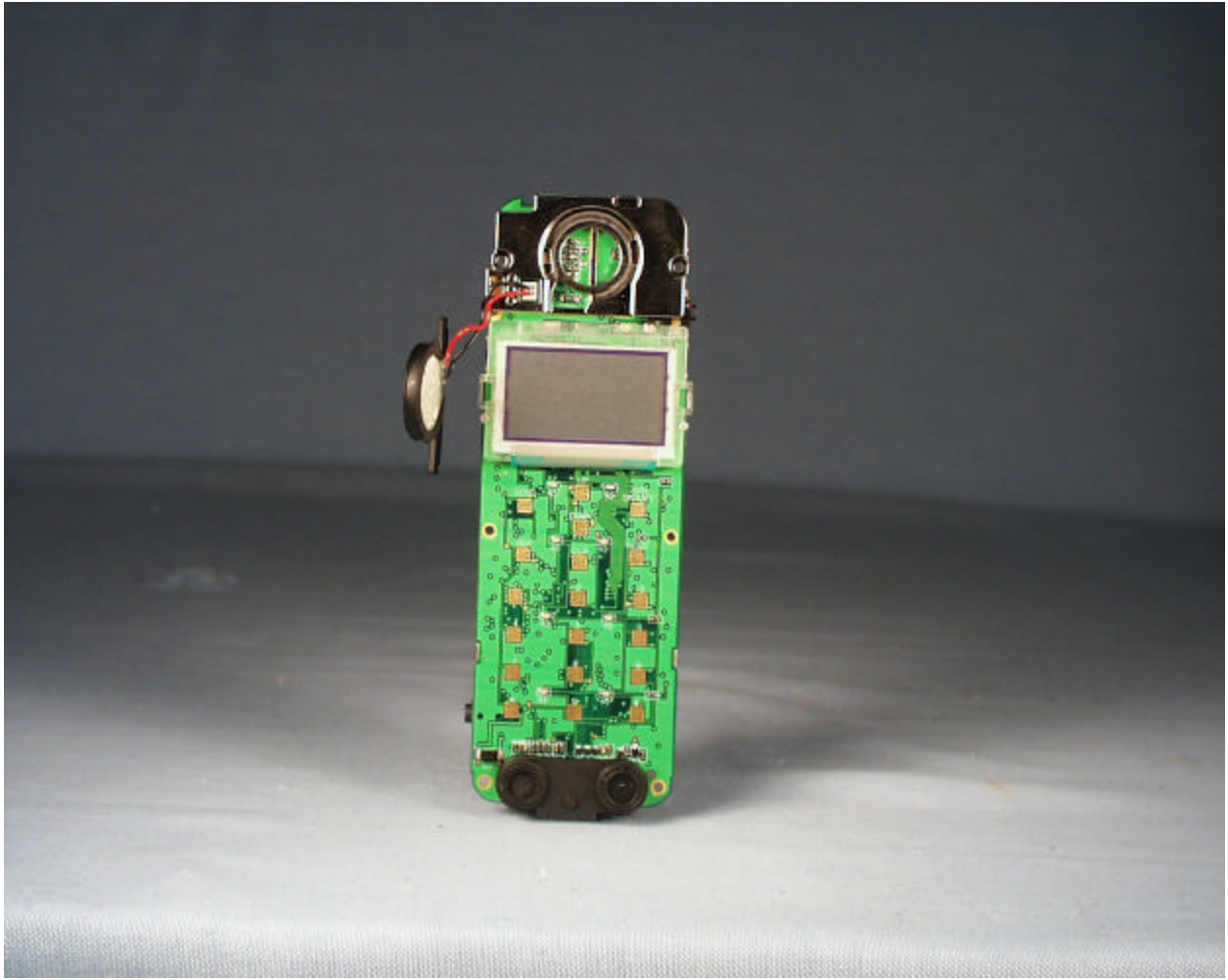
Solder Side
