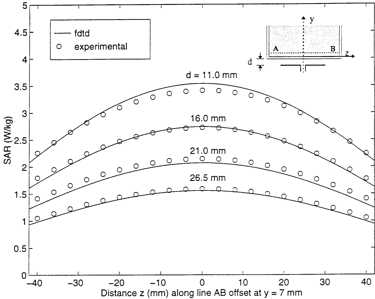
Figure 5b: Comparison of the calculated and measured SAR variations for a box phantom of dimensions 30 x 15 x 50 cm for a line AB parallel to the z axis at a distance y = 7 mm from the surface of the phantom material; 840 MHz; \lambda/2 dipole antenna; 0.5 W radiated power. Calibration factor for the Narda Model 8021 probe at 840 MHz = 0.49 (mW/kg)/ \mu V. Measured for the phantom material \epsilon_r = 41.1 , \sigma = 1.06 S/m.
