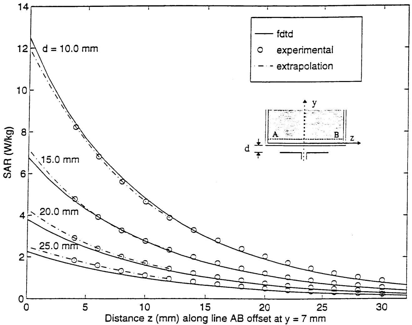
Fig. 5a. Comparison of the calculated and measured SAR variations for a box phantom of dimensions 30 \times 15 \times 50 cm; 1900 MHz; \lambda/2 dipole antenna; 0.5 W radiated power. Calibration factor for the Narda Model 8021 probe at 1900 MHz = 0.84 (mW/kg)/ \mu V. Measured for the phantom material \epsilon_r = 45.5 , \sigma = 1.31 S/m.
