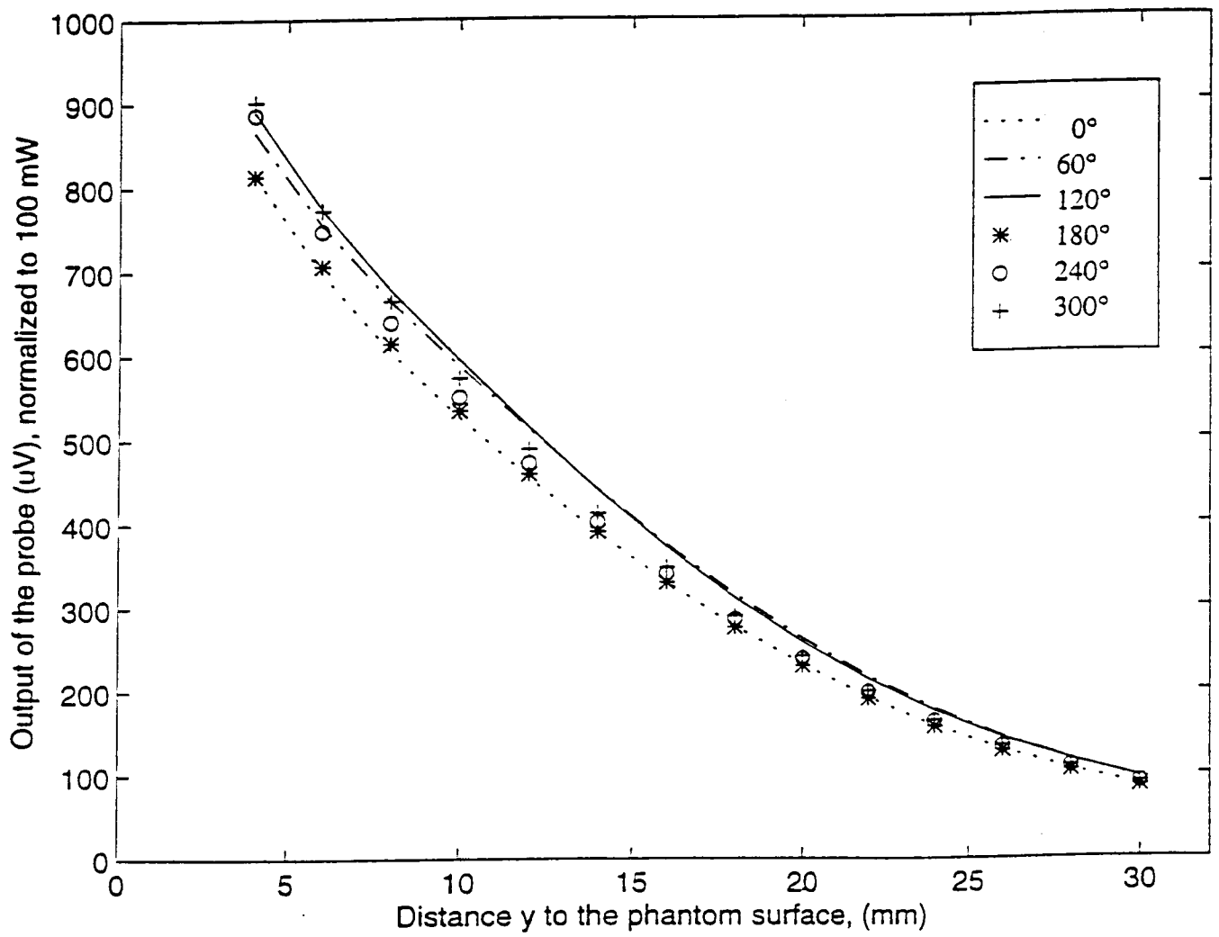
Fig. 3a. Test for isotropy: The model shown in Fig. 1 was used with nominal half wavelength dipole radiator of length 178 mm at 840 MHz.
