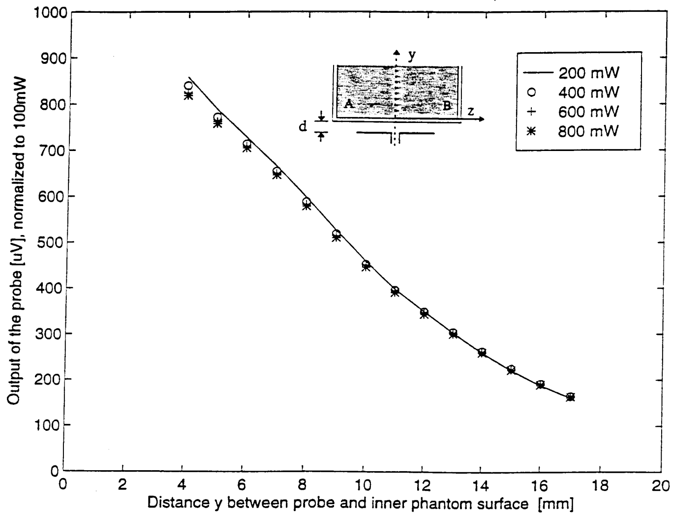
Fig. 2b. Test for square-law behavior at 1900 MHz: Variation of the output voltage (proportional to |E_i|^2 ) for different radiated powers normalized to 0.1 W.
