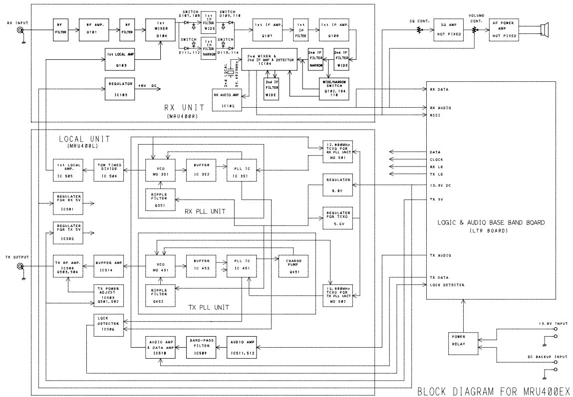
BLOCK DIAGRAM FOR MRU400EX
