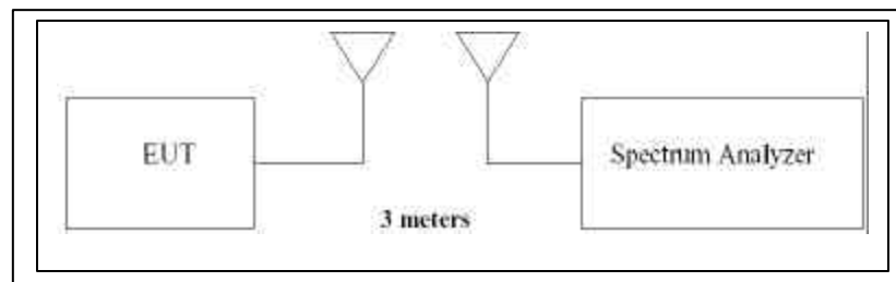
Figure A-1. Test Instrument & Measurement Setup
