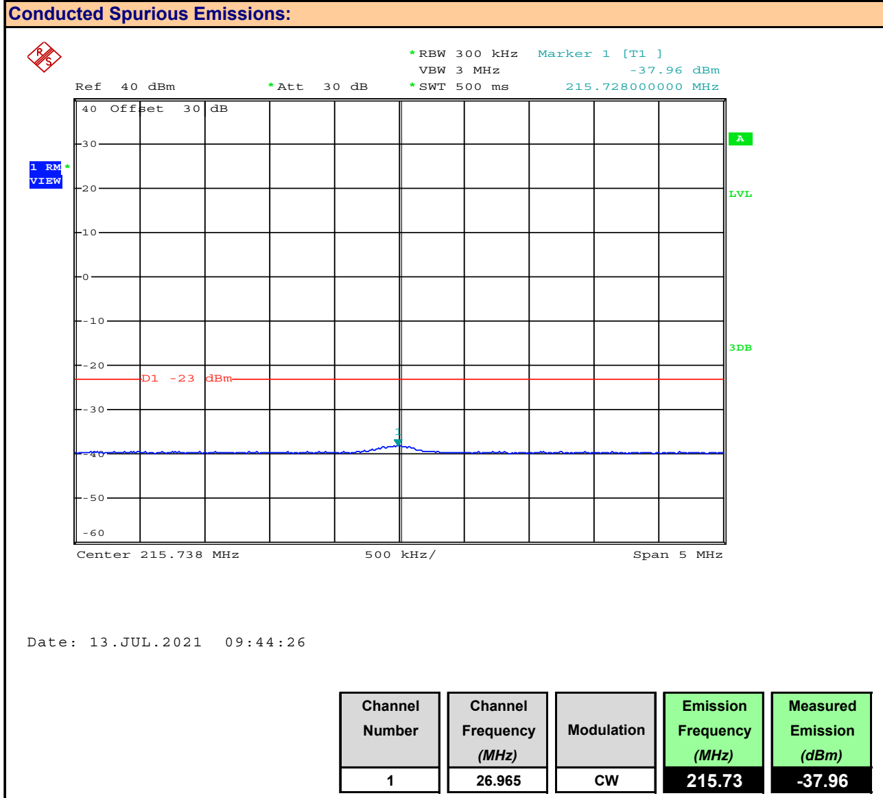
Plot 10.3 – Conducted Out of Band Emissions, Channel 1, 8 th Harmonic
