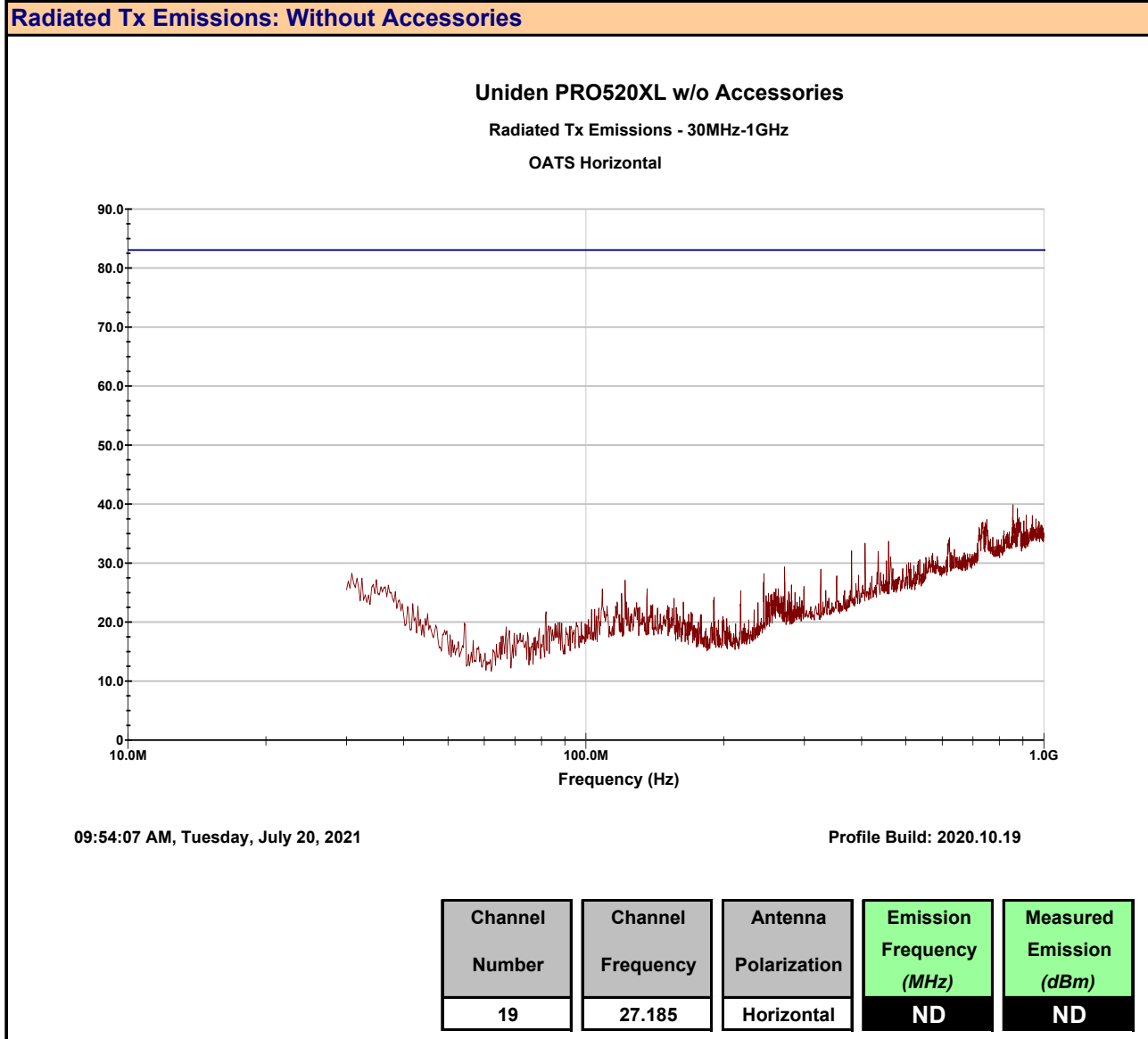
Plot 11.3 – Radiated Spurious Emissions, 30MHz – 1000MHz, Without Accessories Horizontal
