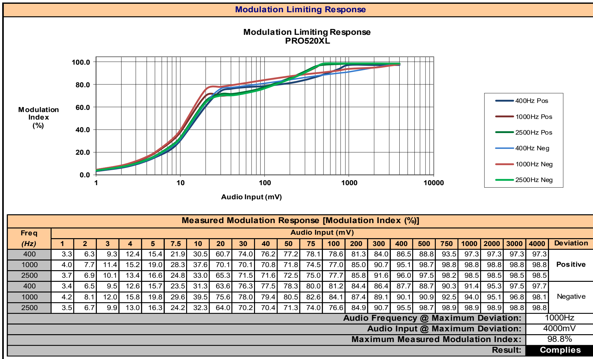
Plot 8.2 – Modulation Limiting Response
