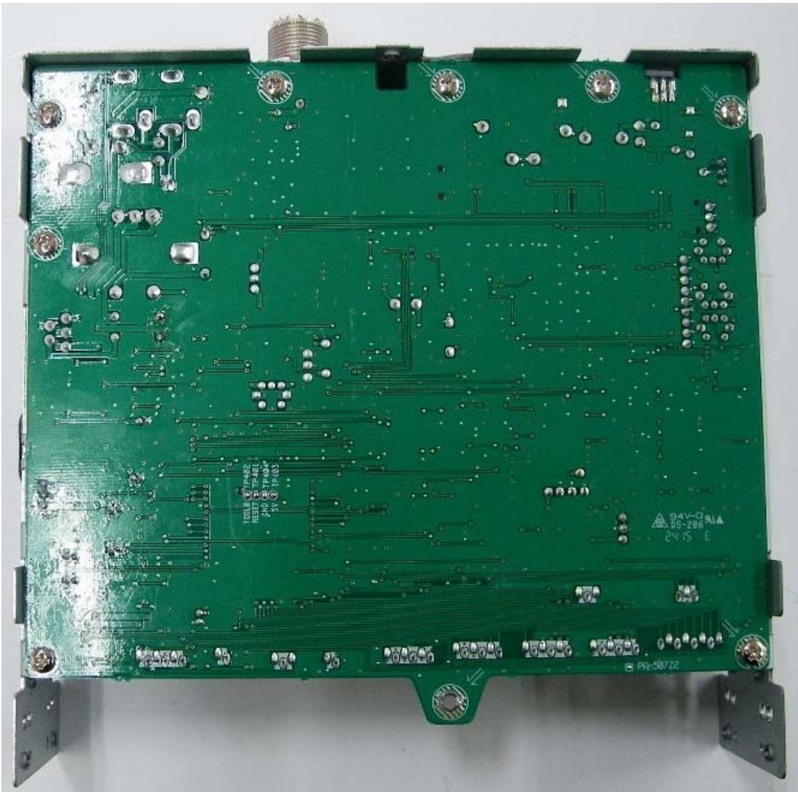
PC78LTD – Main Top View
