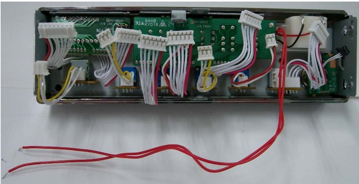
PC78LTD – Front Control Panel Inner View
