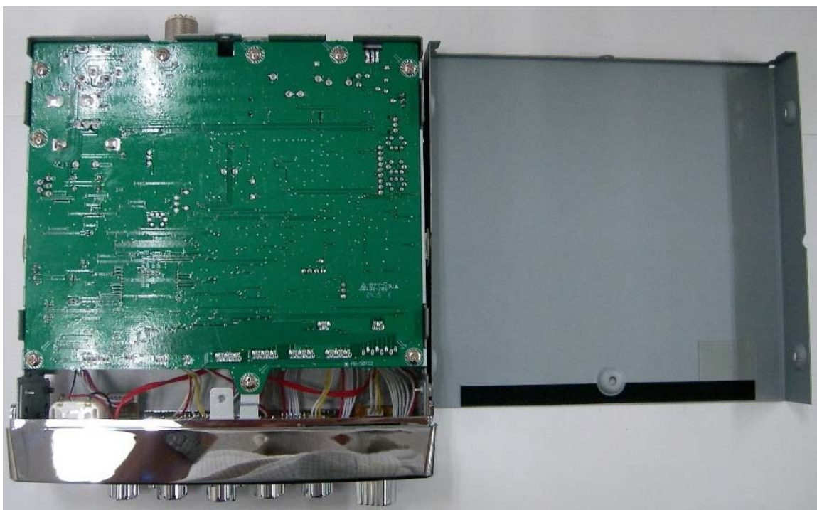
PC78LTD – Main Bottom View w/ Cover
