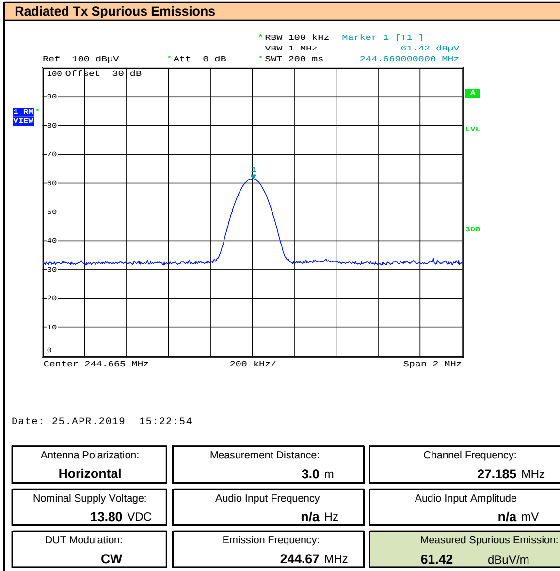
Plot 11.10 – Radiated Spurious Emissions OATS, 9 th Harmonic, Horizontal
