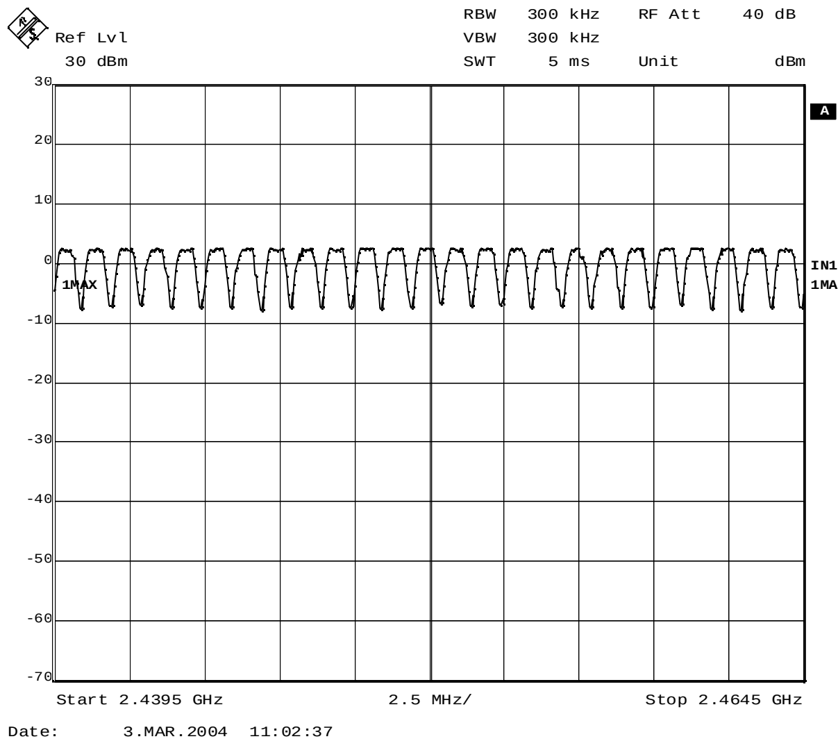
Plot 2-3. Number of Hopping Frequencies (range 3)
