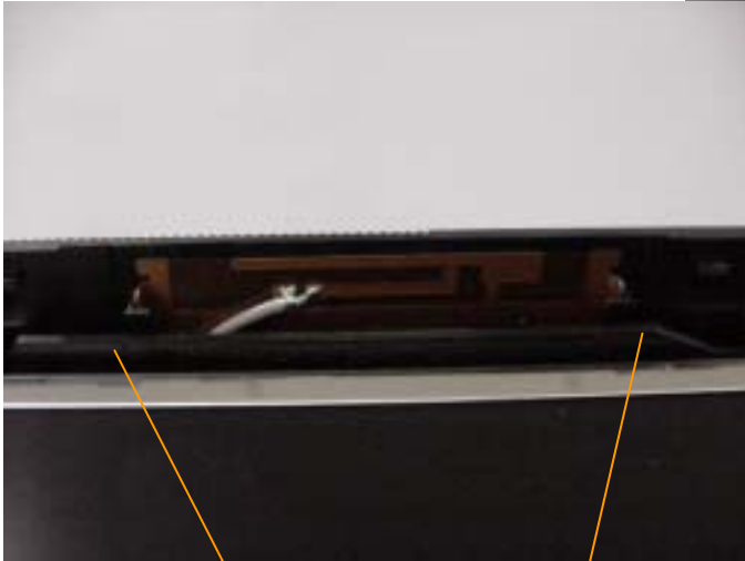
Main antenna Dual Band Inverted-F type
