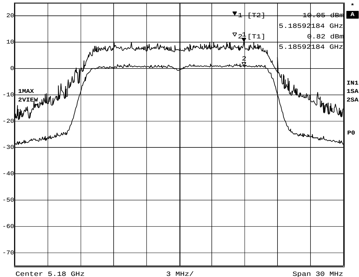
Plot 4-1 Peak Excursion Ratio at 5180MHz
