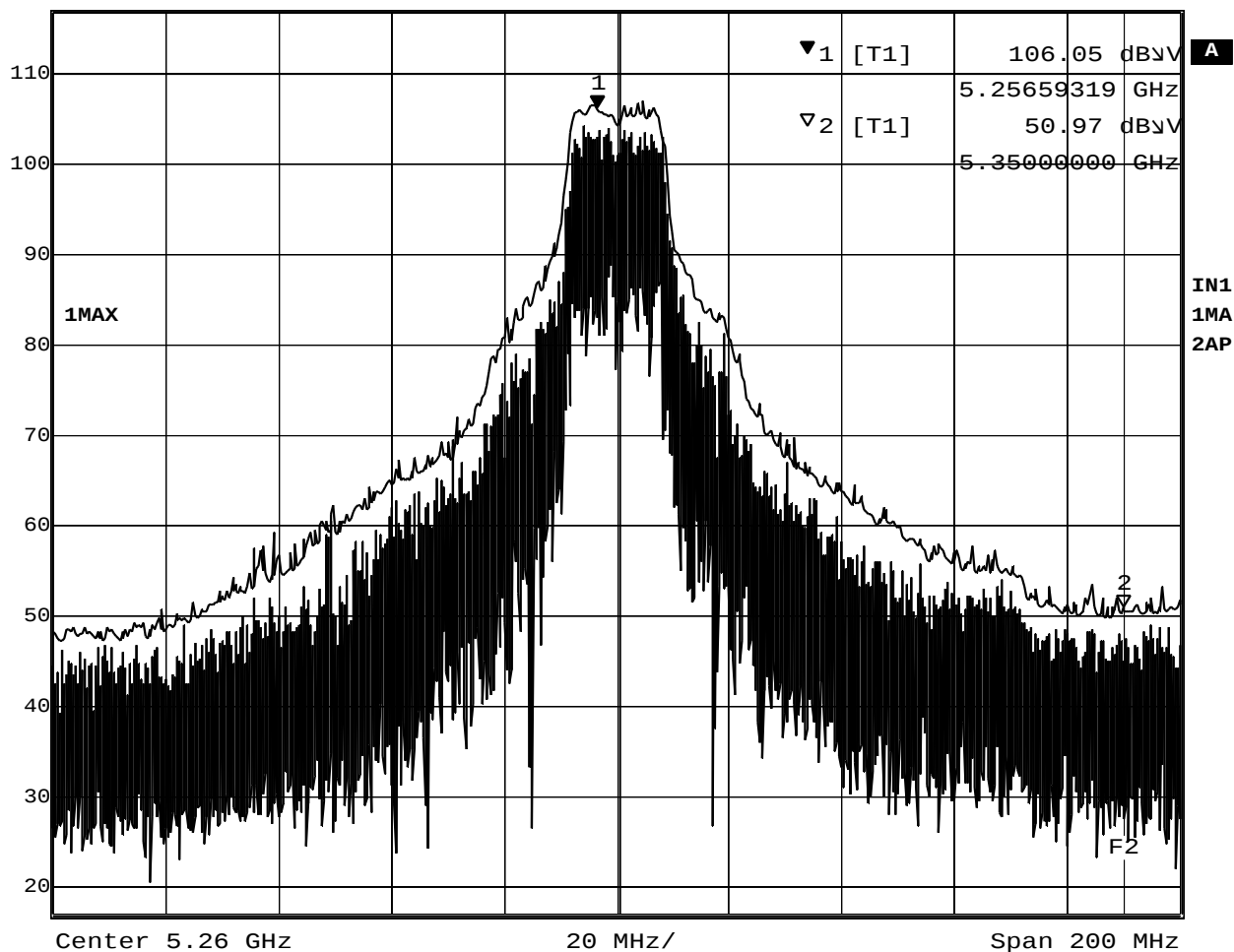
Plot 7-2-1 5260MHz TX mode (Peak)
