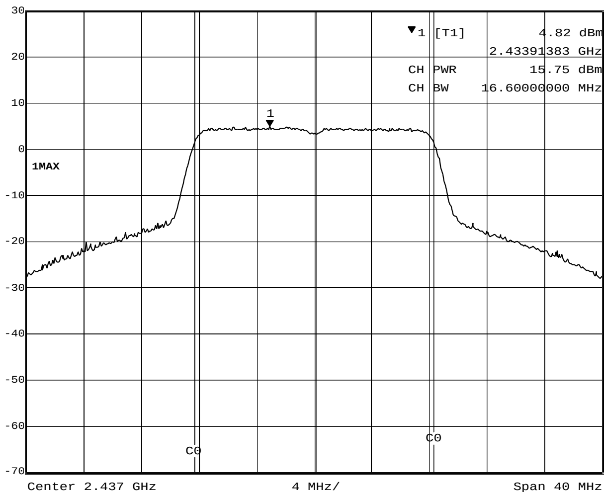
Plot 3-2. Conducted Peak Output Power of 2437MHz
