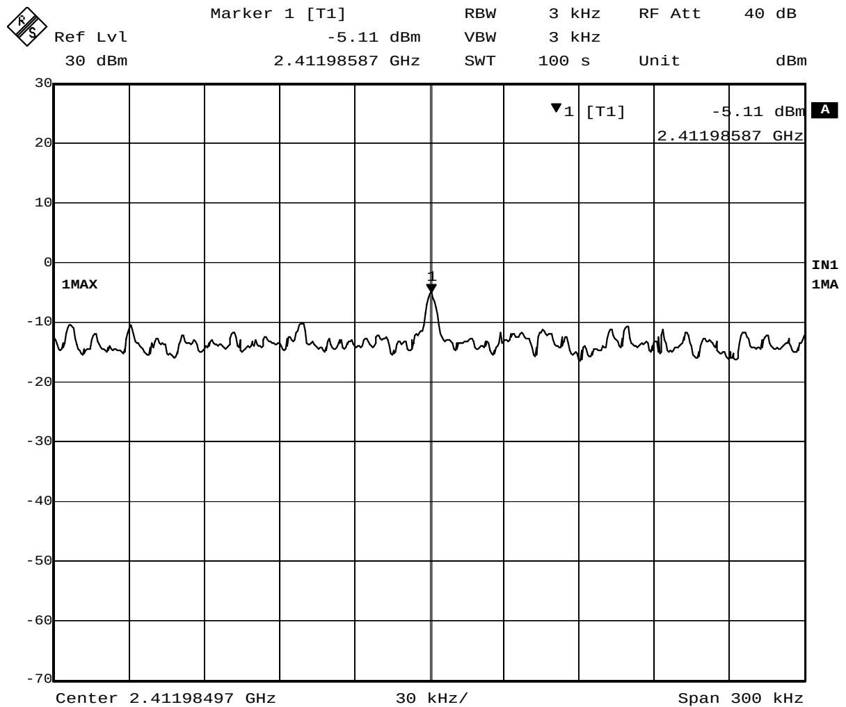
Plot 5-1. Peak Power Spectral Density of 2412MHz (DSSS, 11Mbps)
