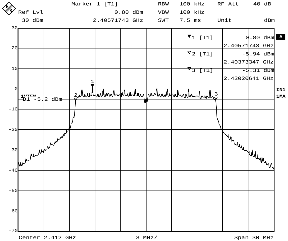
Plot 1-4. 6dB BW at 2412MHz (OFDM, 18Mbps)
