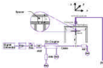
Figure A.0 Dipole Validation Test Setup
