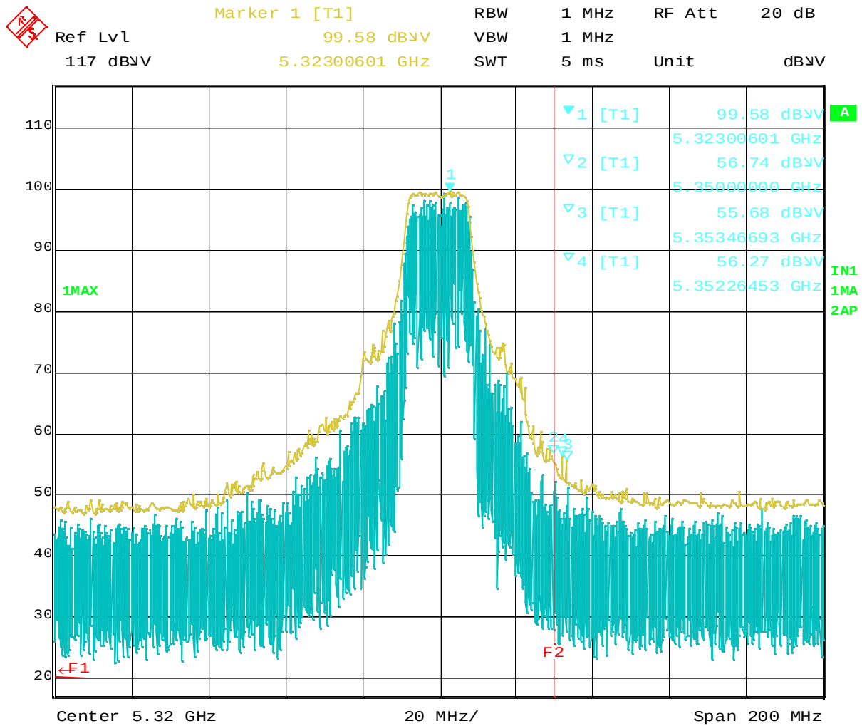
Plot 7-3 5320MHz TX, 6Mbps (Peak), X30 Series
