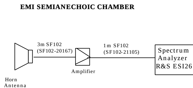
Figure 8-3. Cables for Radiated Emission Test (18 - 25GHz)
