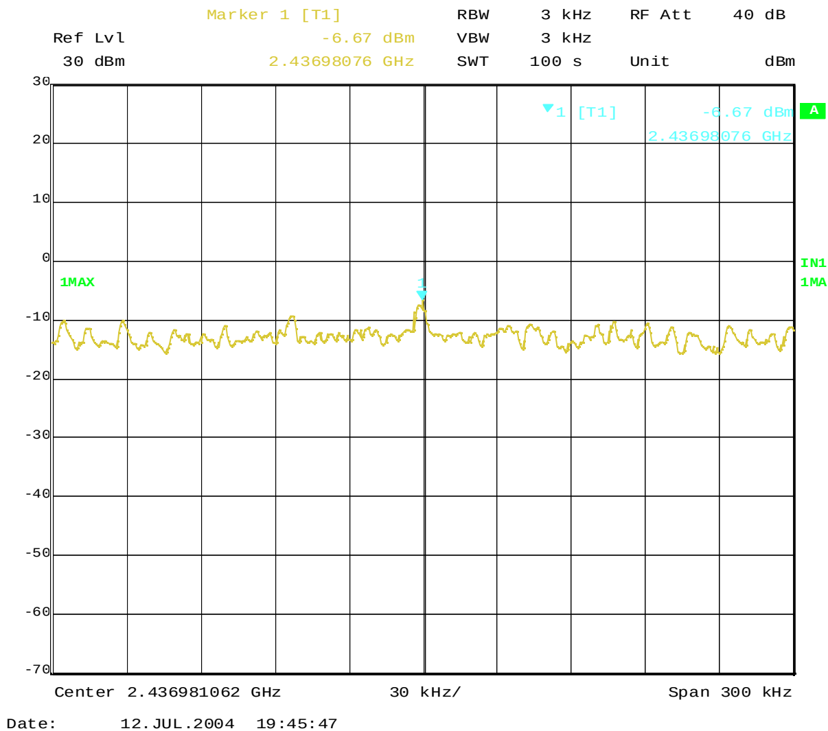
Plot 5-1. Peak Power Spectral Density of 2437MHz (DSSS, 11Mbps)
