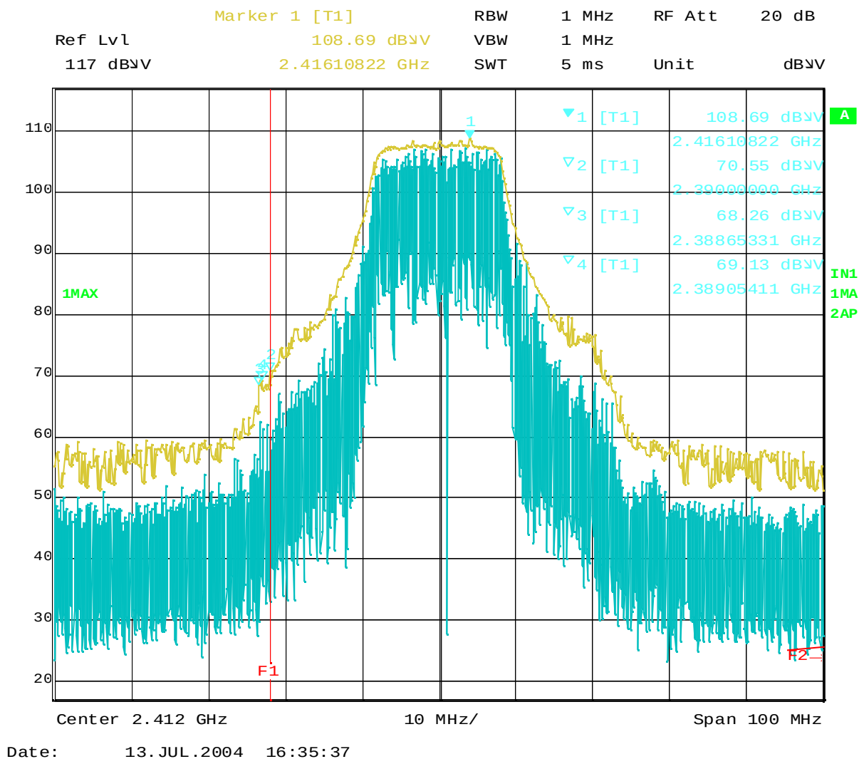
Plot 8-5 Ch.1 2412MHz TX, OFDM 6Mbps (Peak), 14" model
