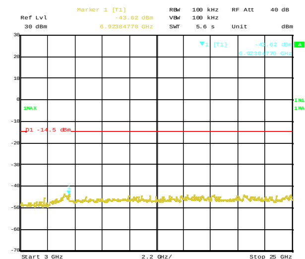
Plot 4-3. Out of band emissions around 2462MHz (DSSS, 11Mbps)
