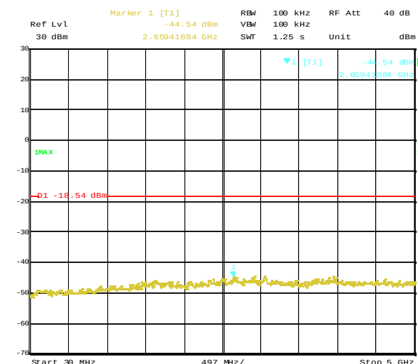
Plot 4-7. Out of band emissions around 5745MHz (OFDM, 6Mbps)
