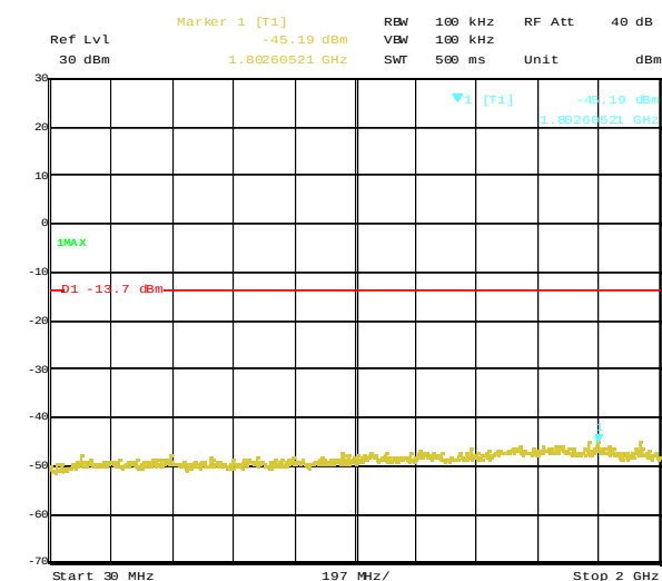
Plot 4-2. Out of band emissions around 2437MHz (DSSS, 11Mbps)
