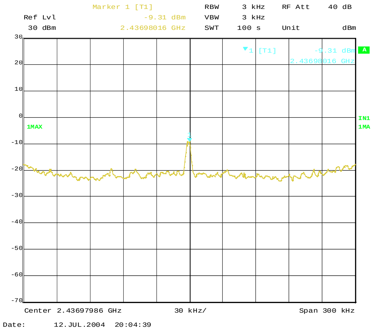
Plot 5-2. Peak Power Spectral Density of 2437MHz (OFDM, 6Mbps)
