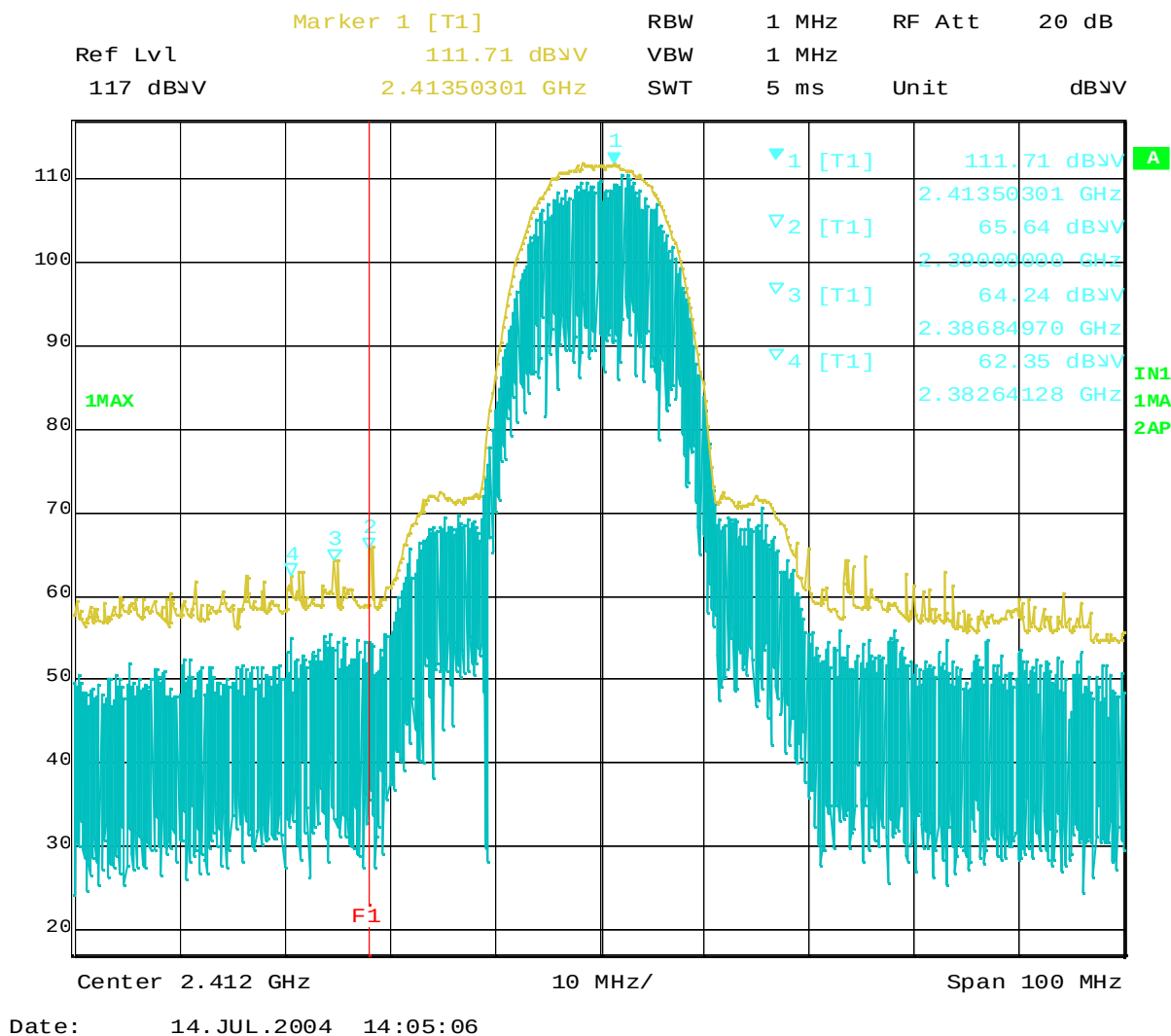
Plot 8-1 Ch.1 2412MHz TX, DSSS 11Mbps (Peak), 14" model
