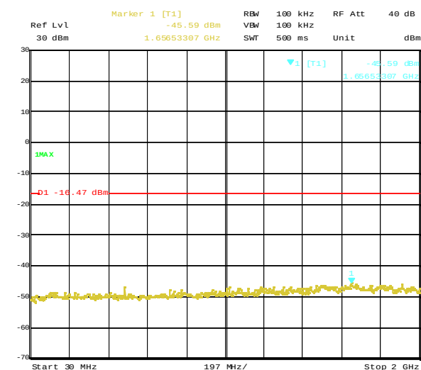
Plot 4-5. Out of band emissions around 2437MHz (OFDM, 6Mbps)
