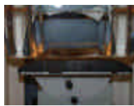
Figure A.10.1 Body SAR Test Setup -- Bystander Position, LCD Open -- (Main Antenna)
