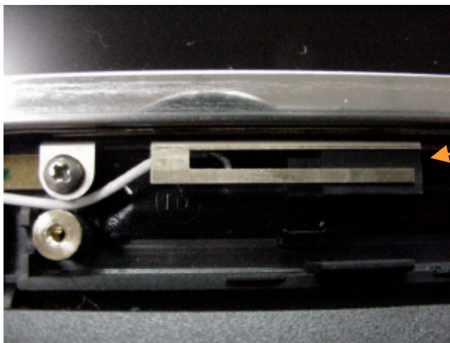
R50 14/15 inch Bluetooth Antenna (Meander Antenna) P/N: 91P6817
