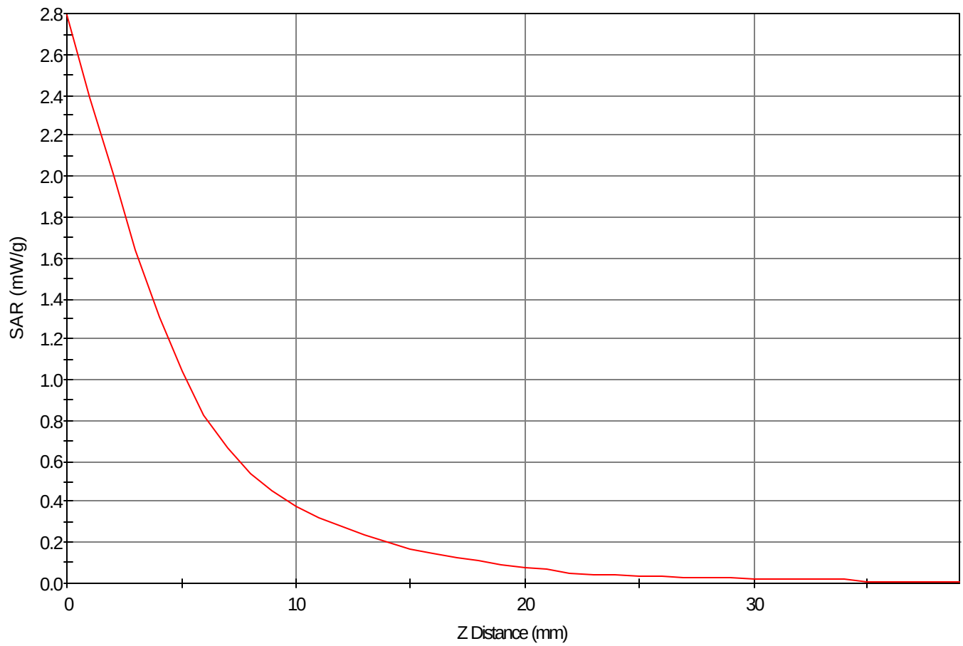
SAR - Z Axis at Hotspot x:-5.0 y:-35.0
