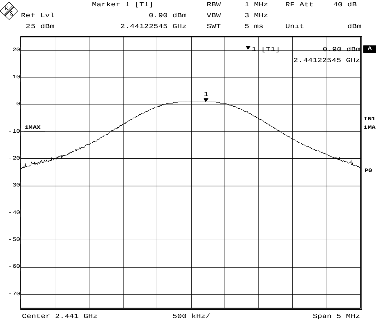
Peak Output Power (TX on 2441MHz)
