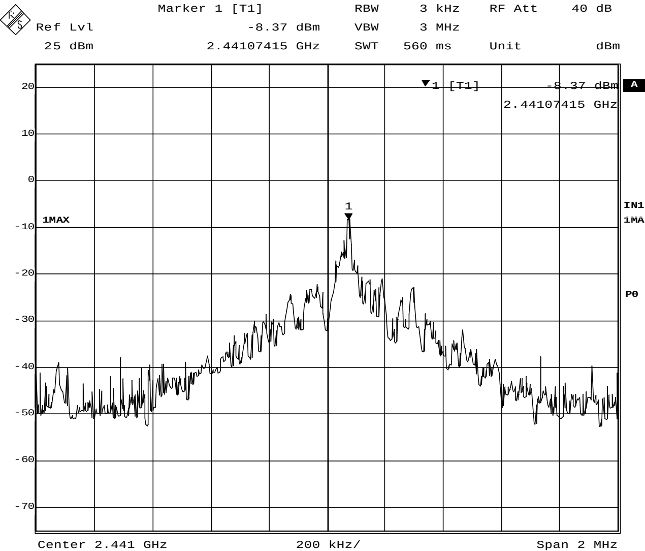
Transmitter Power Spectral Density (Inquiry)
