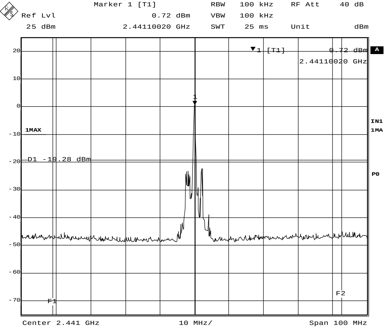
Out of Band Emissions (TX on 2441MHz)
