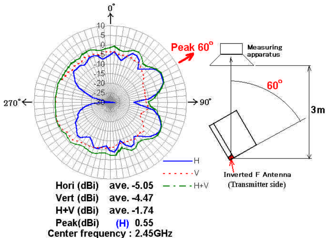
Main antenna
