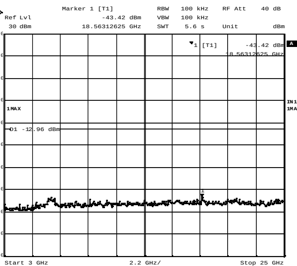
Plot 4-3. Out of band emissions around 2462MHz (11Mbps)
