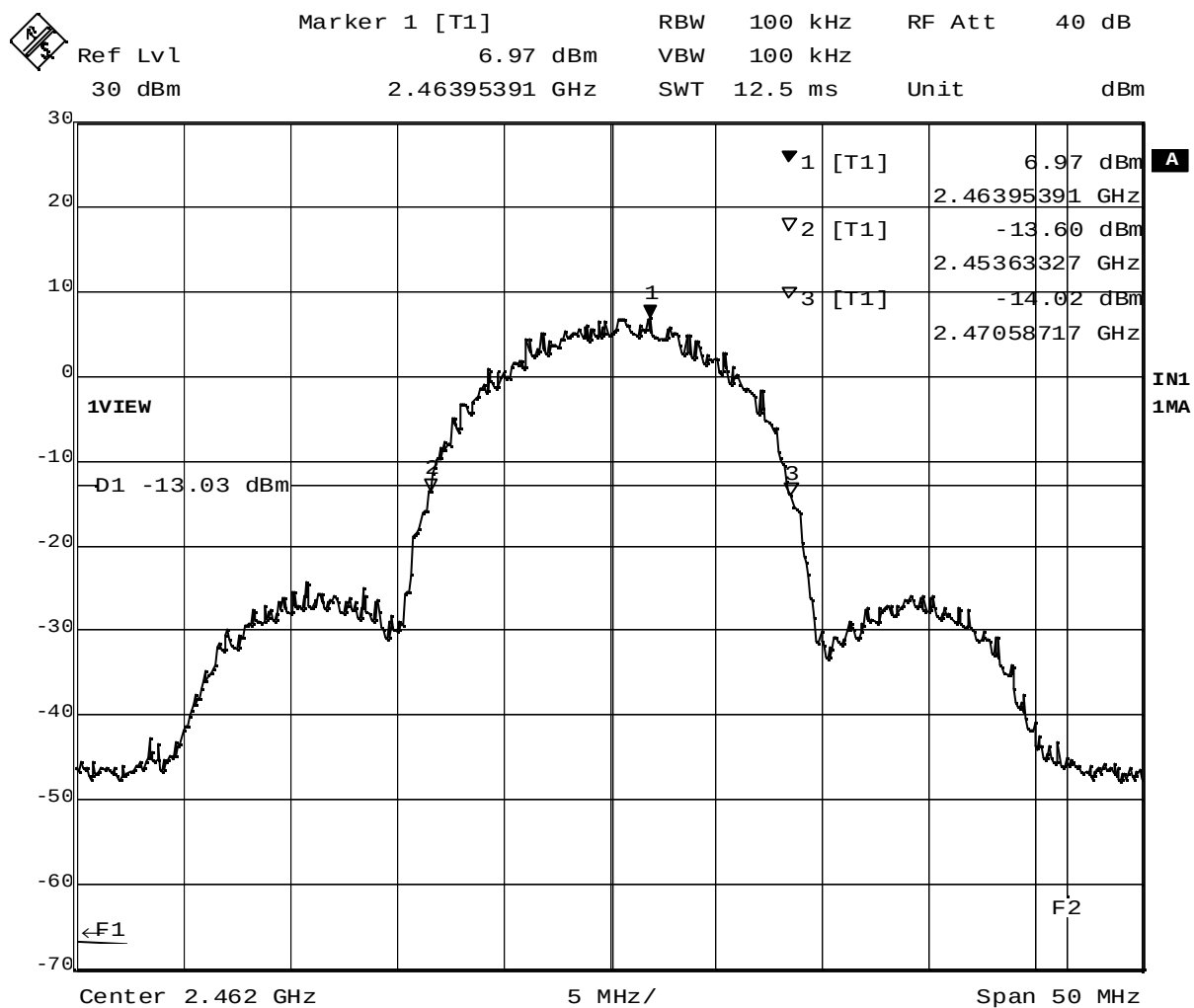
Plot 2-3. 20dB BW at 2462MHz (11Mbps)
