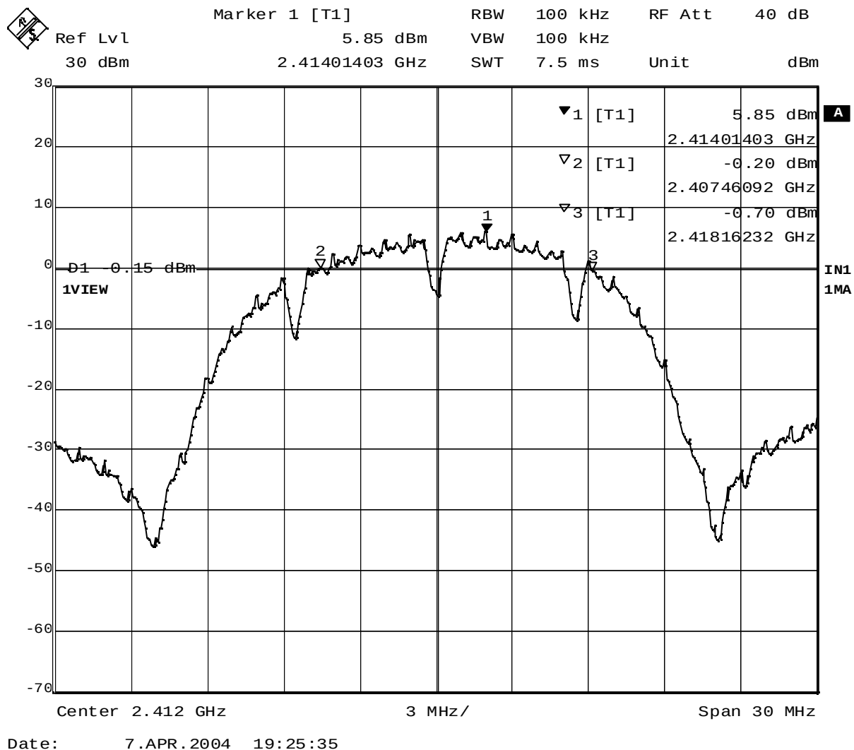
Plot 1-1. 6dB BW at 2412MHz. (1Mbps)
