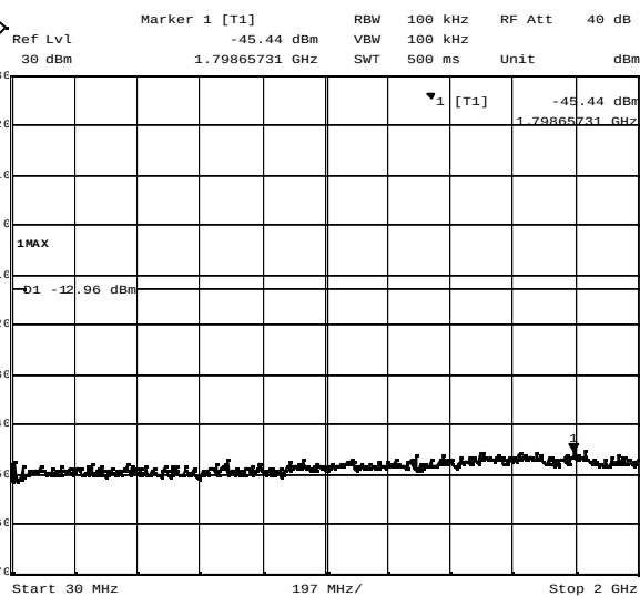
Plot 4-3. Out of band emissions around 2462MHz (11Mbps)
