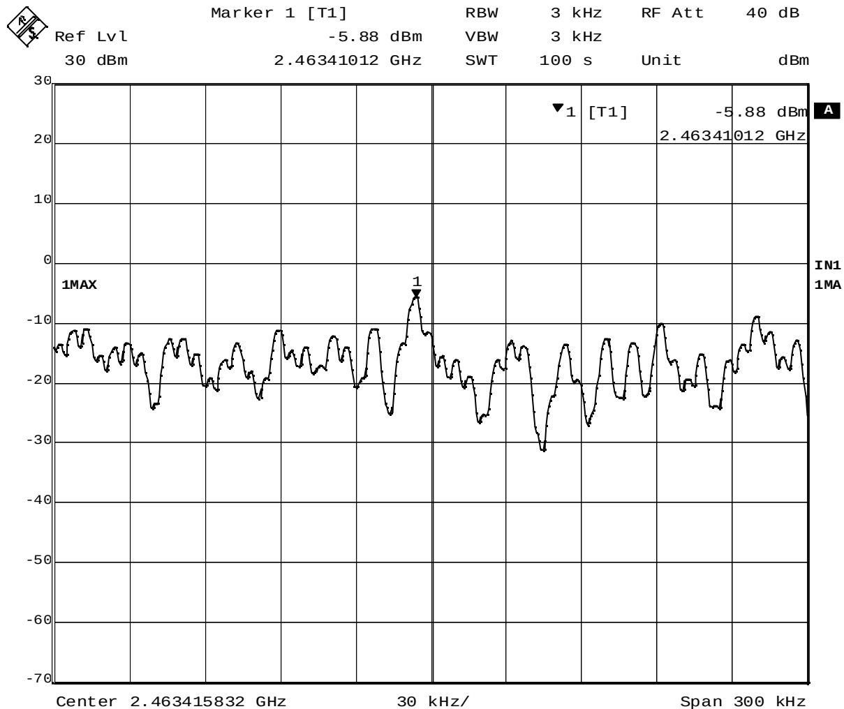
Plot 5-3. Peak Power Spectral Density of 2462MHz (11Mbps)
