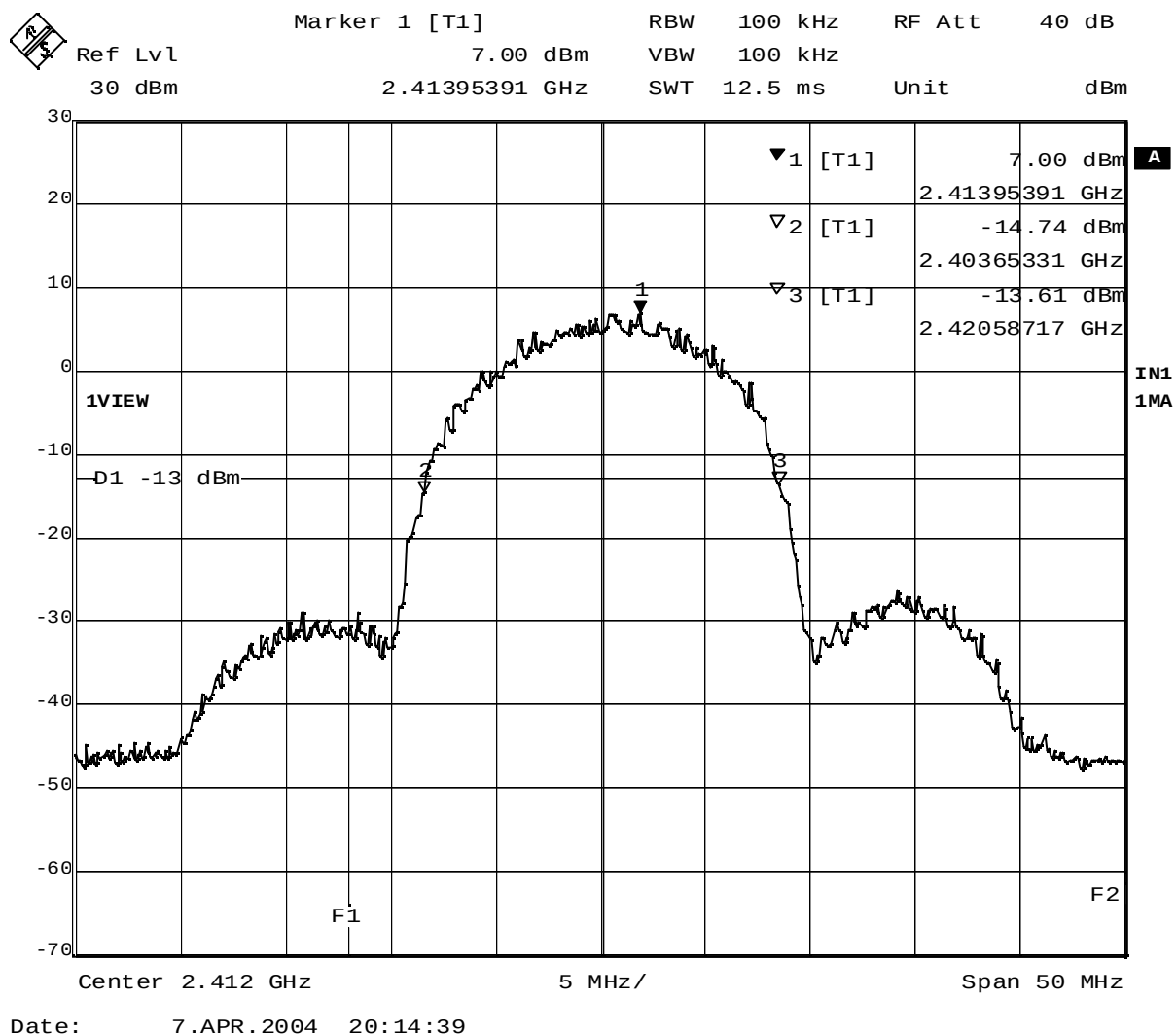
Plot 2-1. 20dB BW at 2412MHz (11Mbps)
