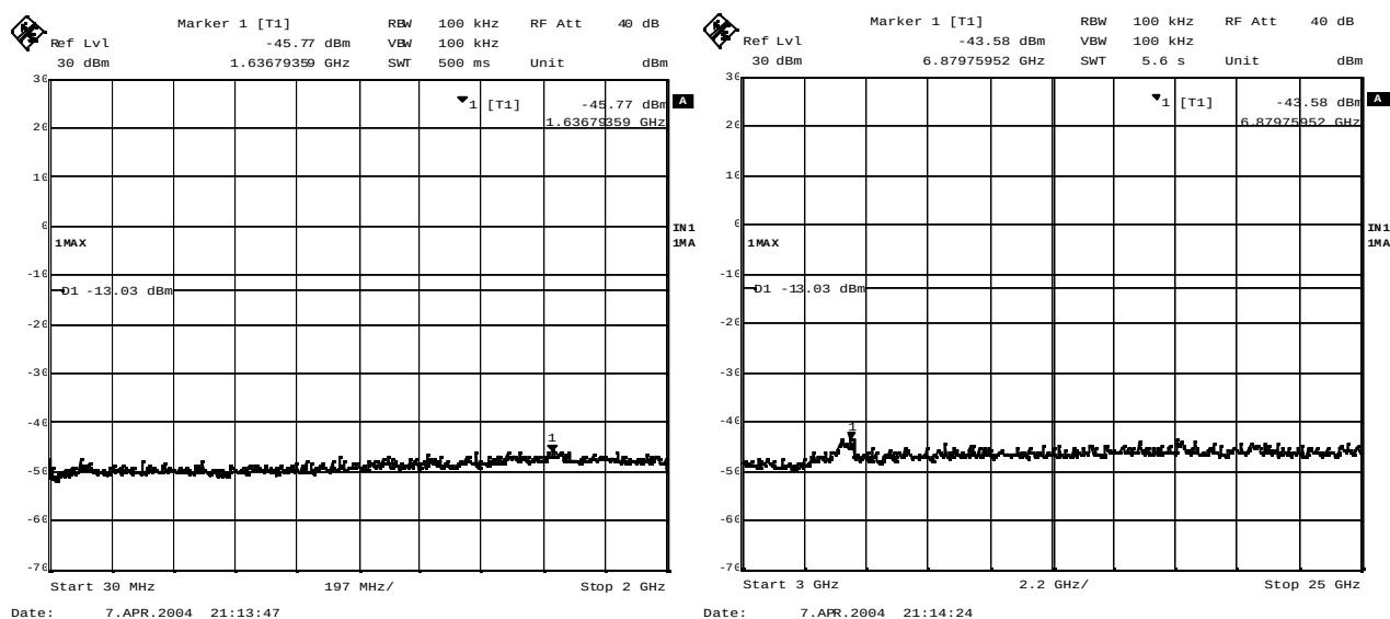
Plot 4-1. Out of band emissions around 2412MHz (11Mbps)
