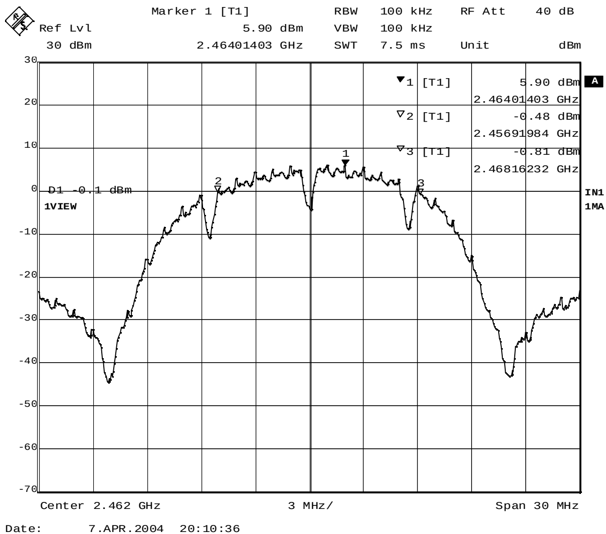
Plot 1-3. 6dB BW at 2462MHz (1Mbps)
