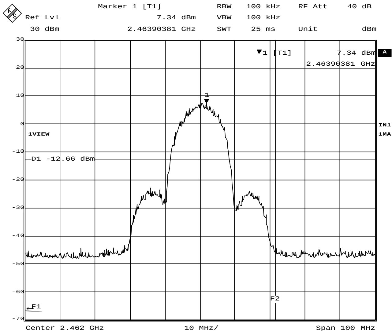
Plot 2-6. Out of band emissions around 2462MHz
