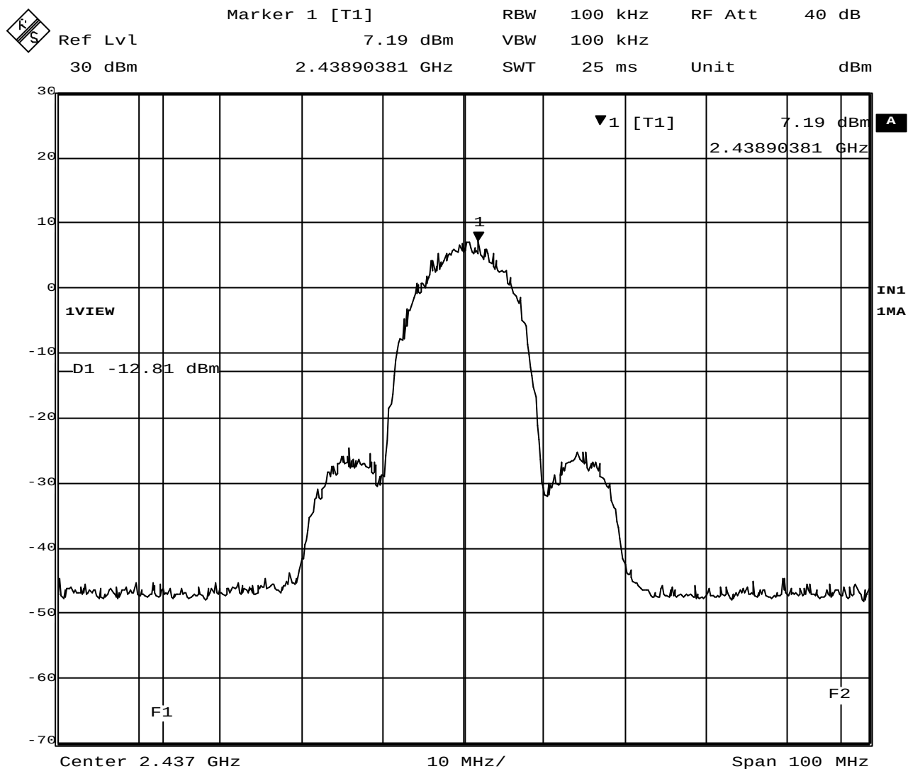
Plot 2-5. Out of band emissions around 2437MHz
