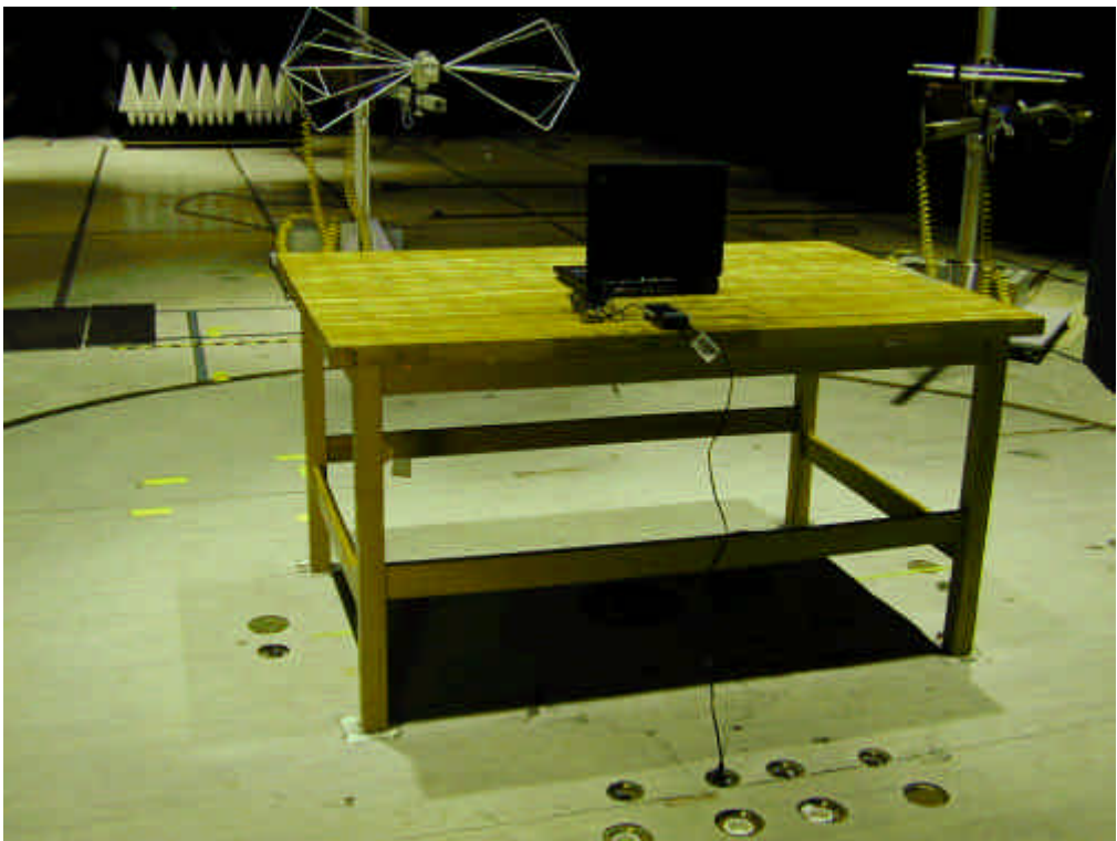
Semi-anechoic Chamber #1
