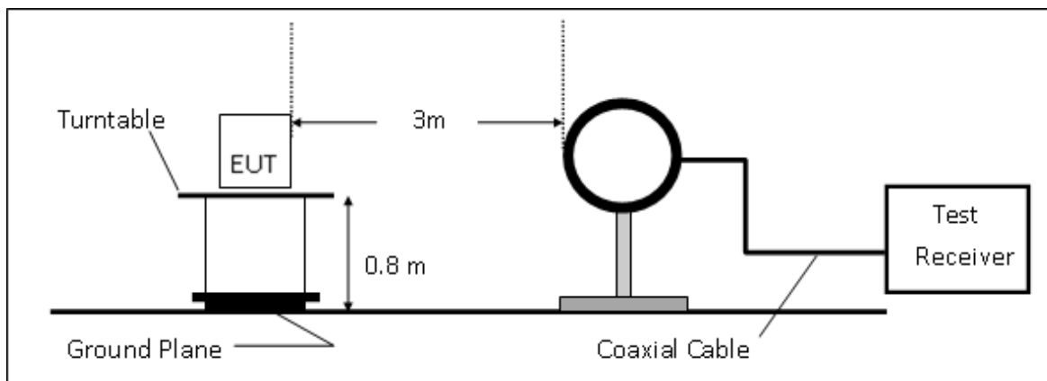
(B) Radiated Emission Test Set-UP, Frequency form 30MHz to 1000MHz
