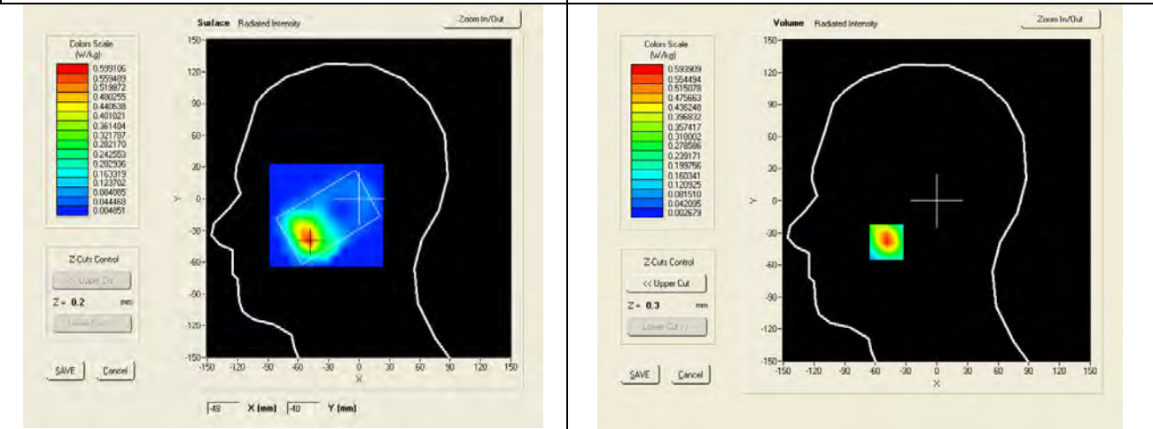
SAR, Z Axis Scan (X = -49, Y = -39)
