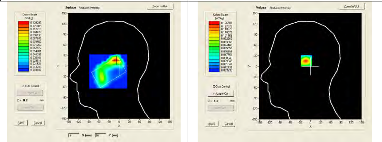
SAR, Z Axis Scan (X = -10, Y = 17)
