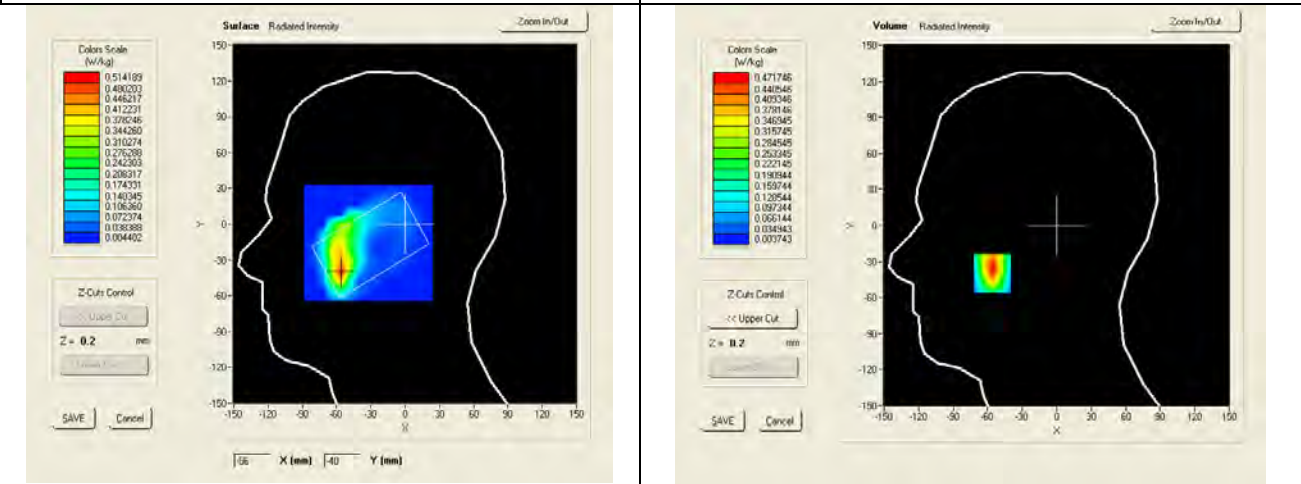
SAR, Z Axis Scan (X = -56, Y = -40)
