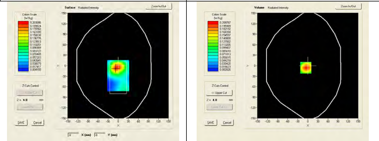
SAR, Z Axis Scan (X = -6, Y = -6)
