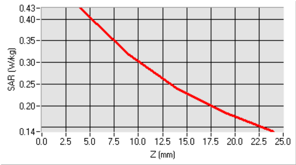
SAR, Z Axis Scan (X = -32, Y = -23)
