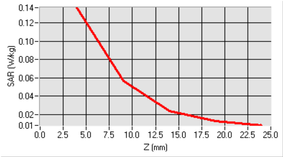
SAR, Z Axis Scan (X = -10, Y = 17)
