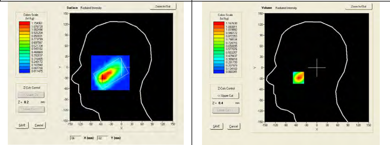
SAR, Z Axis Scan (X = -53, Y = -28)
