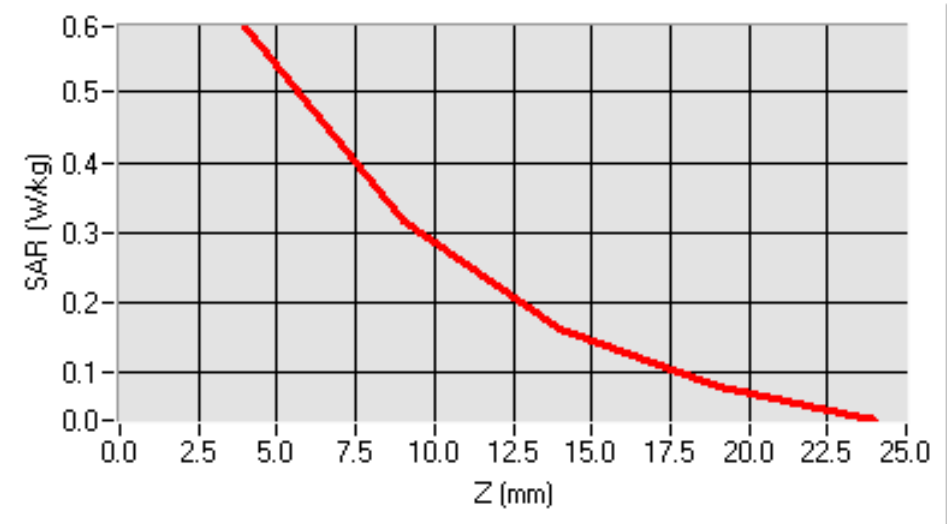
SAR, Z Axis Scan (X = -49, Y = -39)
