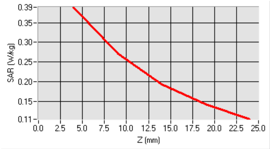
SAR, Z Axis Scan (X = 0, Y = -41)
