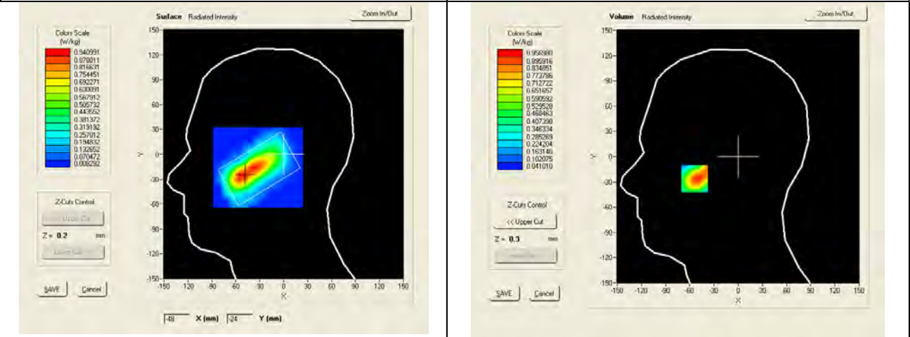
SAR, Z Axis Scan (X = -54, Y = -26)
