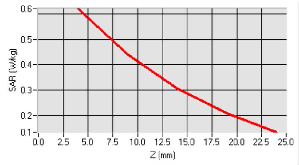
SAR, Z Axis Scan (X = 5, Y = -15)
