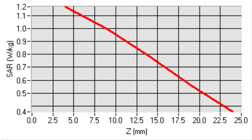
SAR, Z Axis Scan (X = -53, Y = -28)
