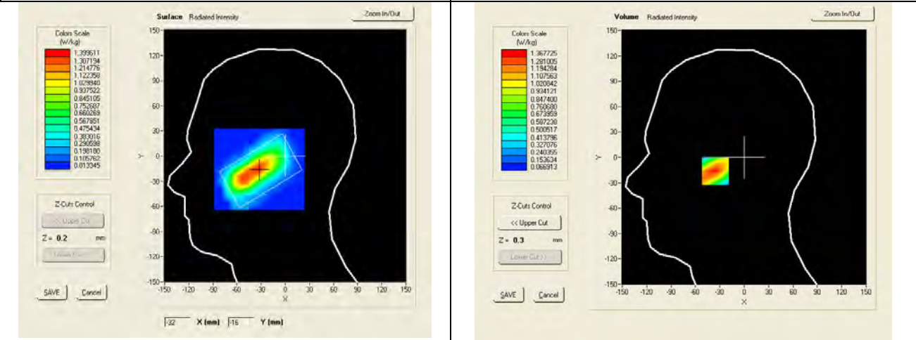
SAR, Z Axis Scan (X = -33, Y = -16)
