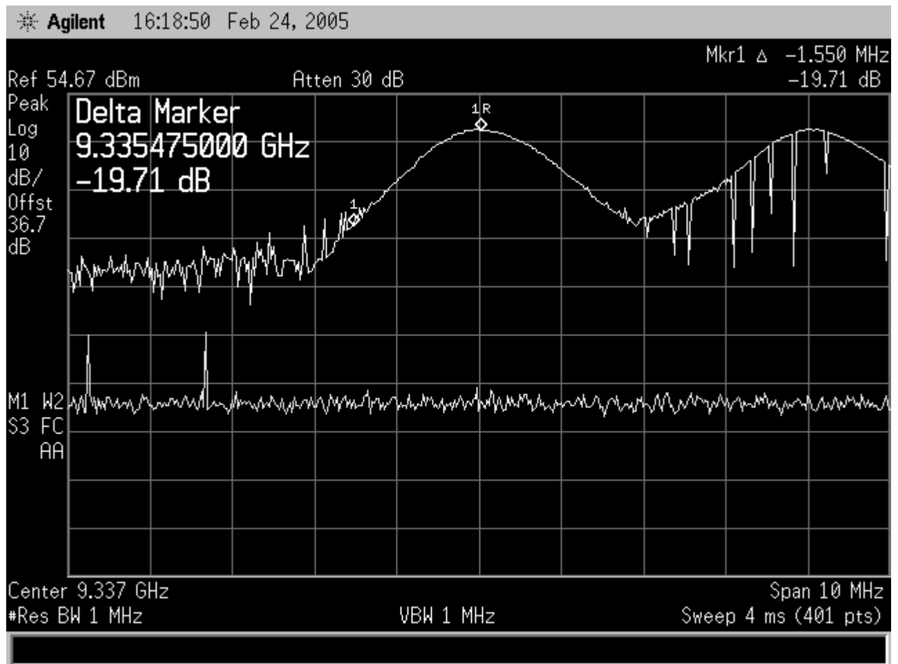
Figure 11-30 Frequency Stability, Lower Edge @ 0C
