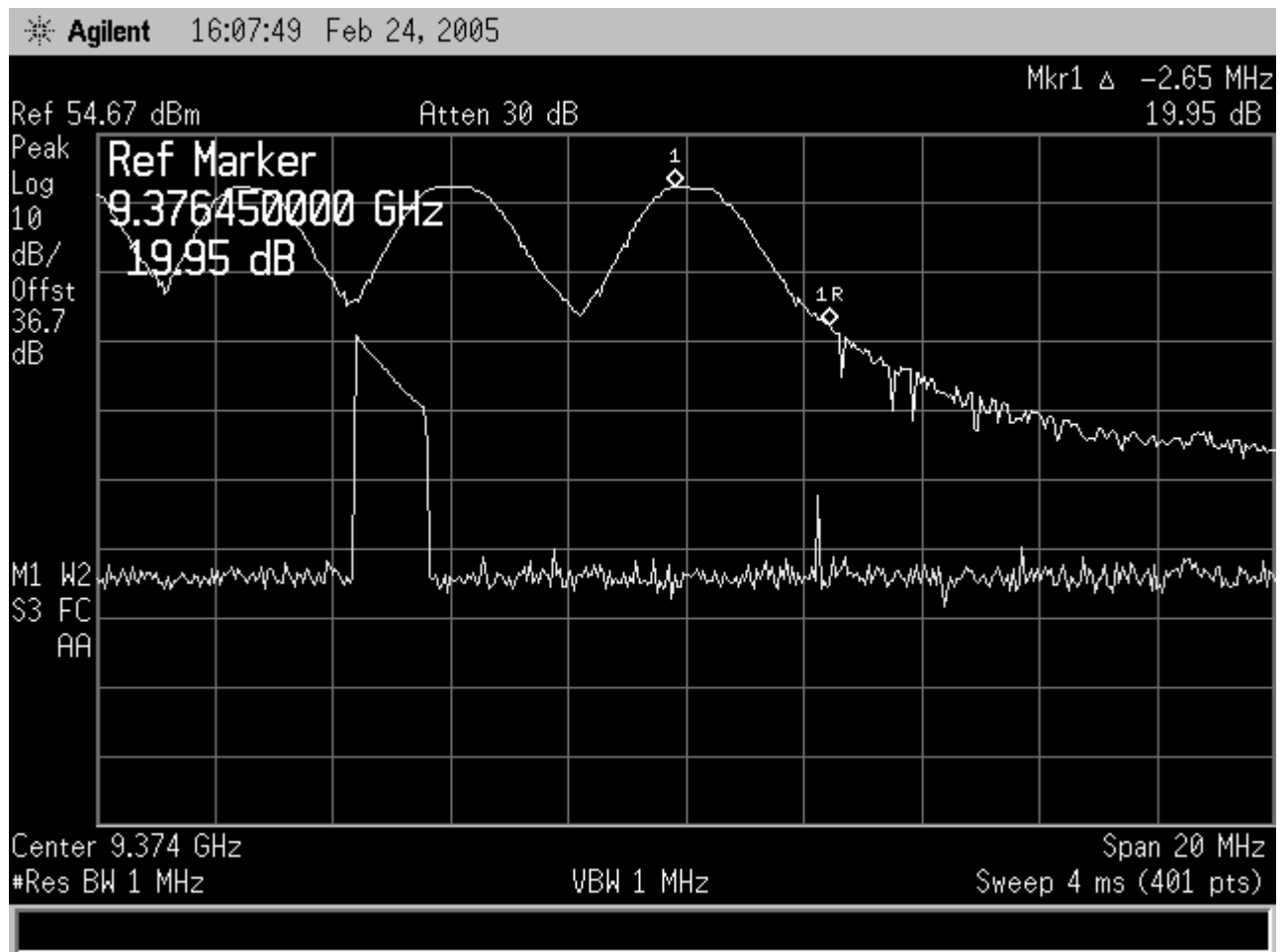
Figure 11-85 Frequency Stability, 230 Vdc Upper Edge @ 0C
