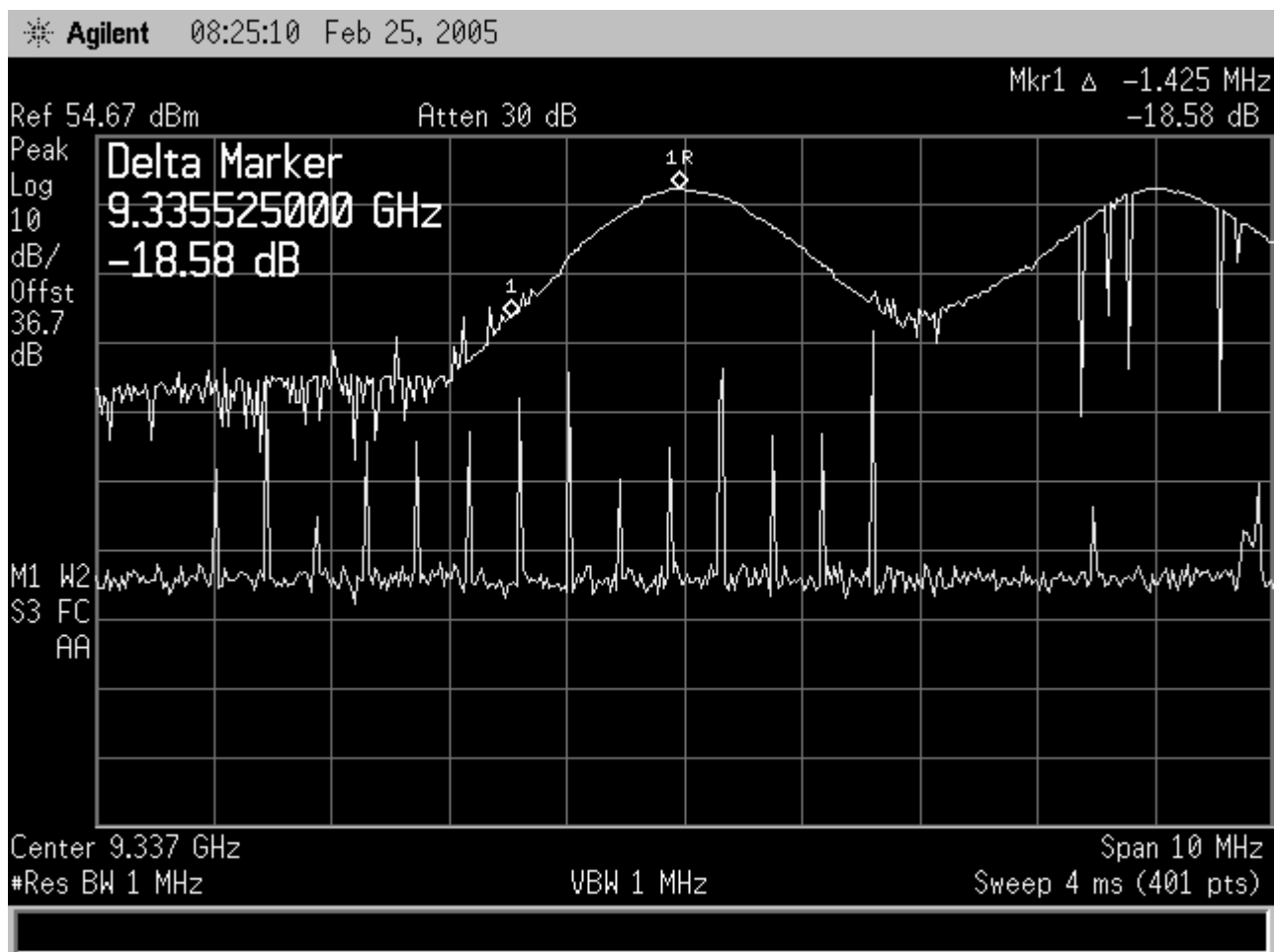
Figure 11-75 Frequency Stability, 230 Vdc Lower Edge @ 10C
