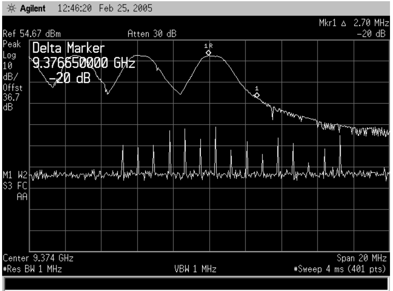
Figure 11-69 Frequency Stability, 170 Vdc Upper Edge @ +60C
