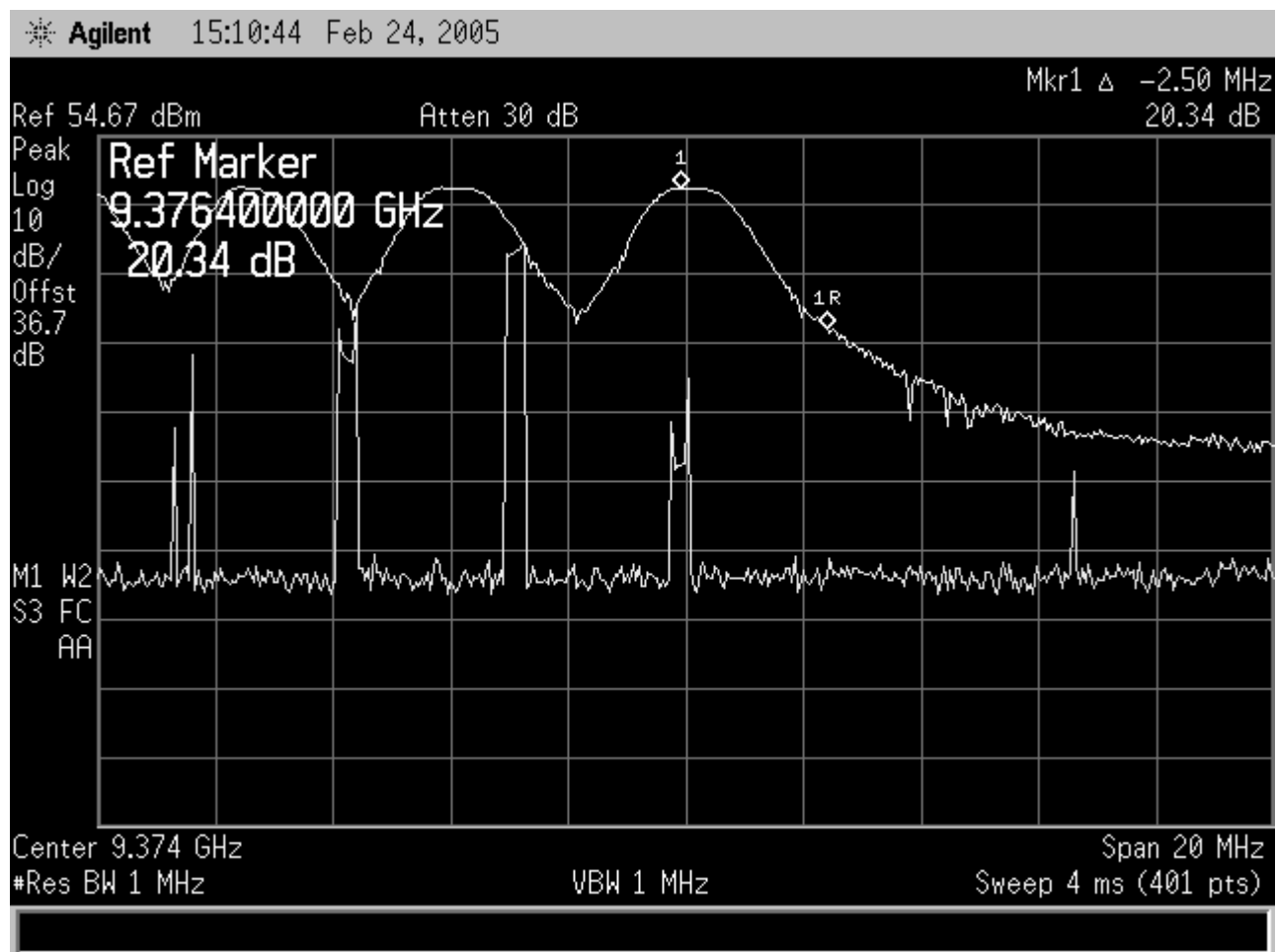
Figure 11-84 Frequency Stability, 230 Vdc Upper Edge @ -10C
