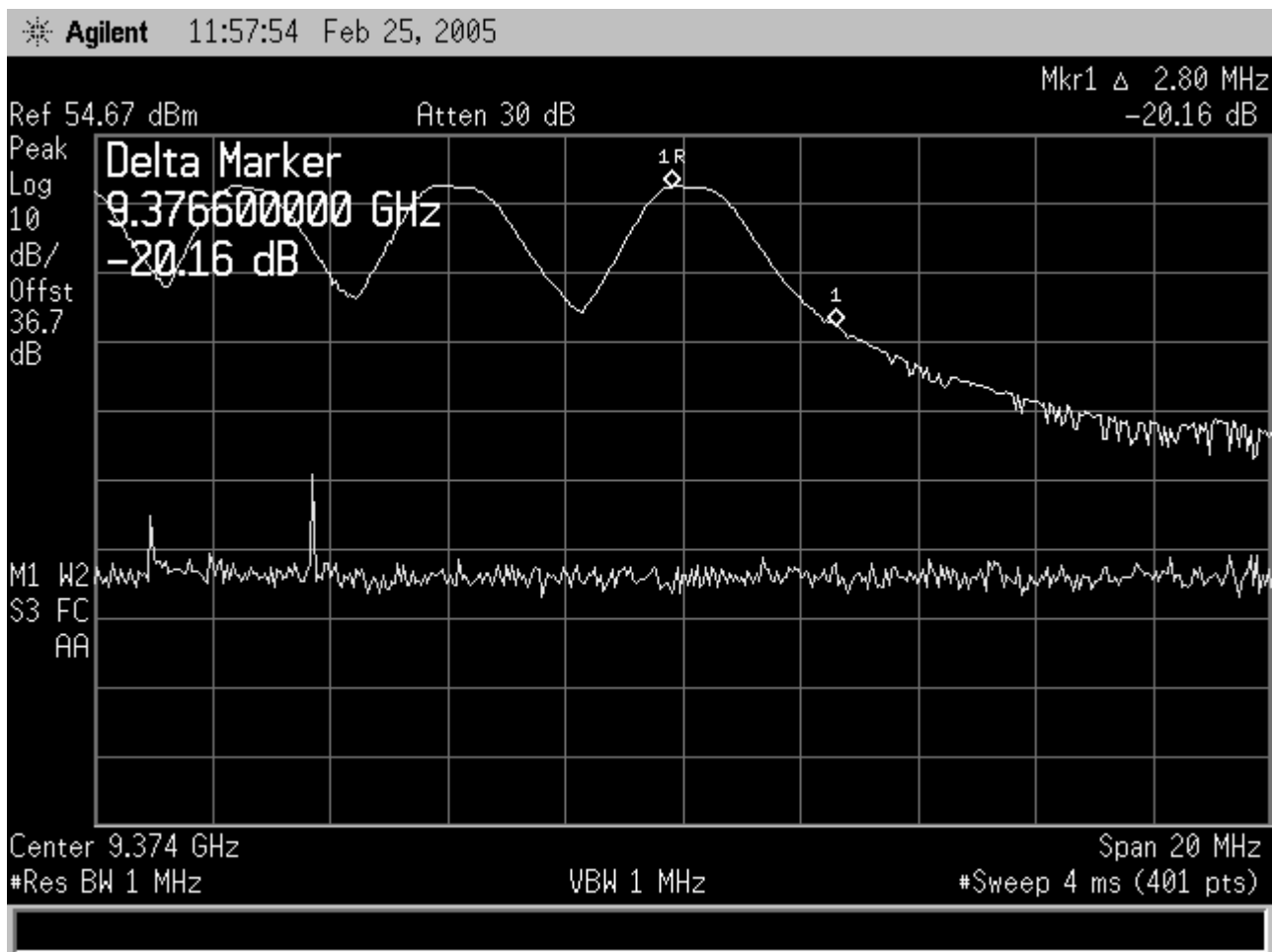
Figure 11-68 Frequency Stability, 170 Vdc Upper Edge @ +50C
