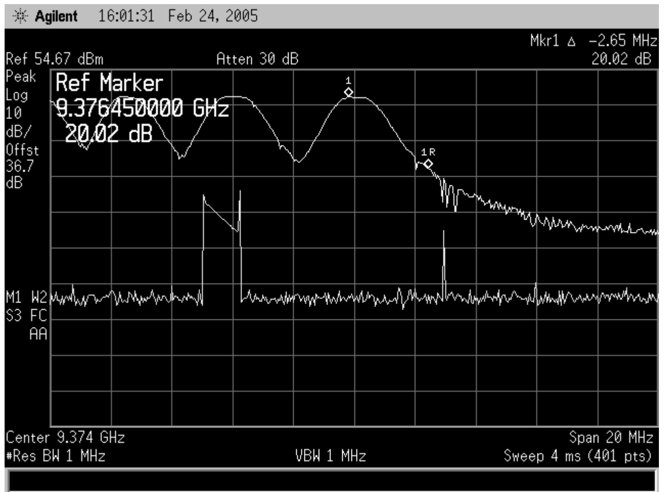
Figure 11-63 Frequency Stability, 170 Vdc Upper Edge @ 0C
