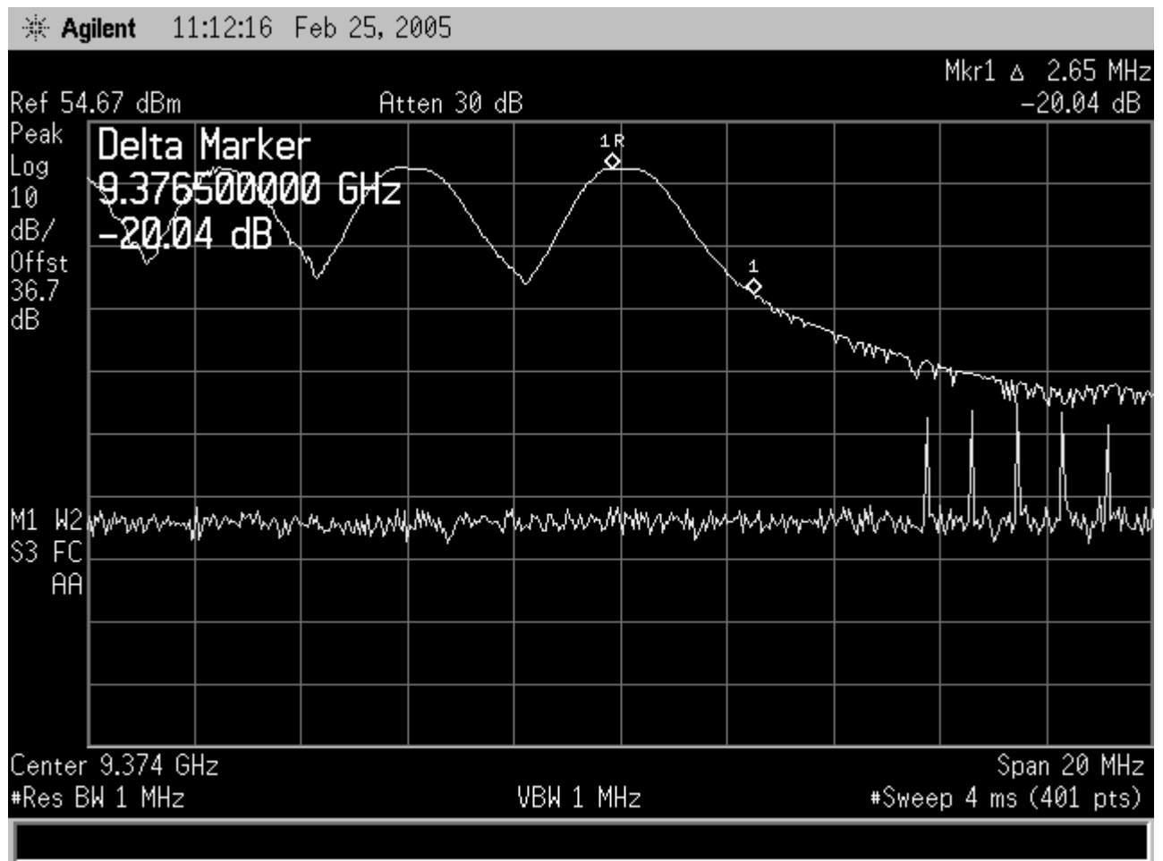
Figure 11-89 Frequency Stability, 230 Vdc Upper Edge @ +40C
