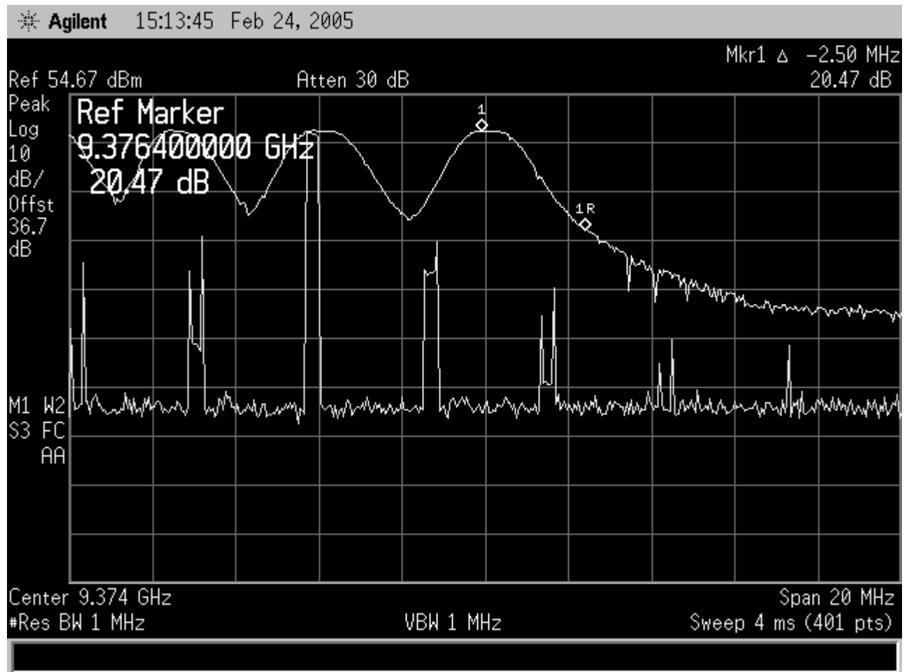
Figure 11-40 Frequency Stability, Upper Edge @ -10C
