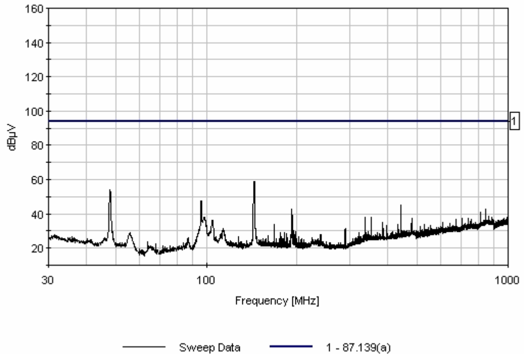
Figure 11-18 Spurious Emissions, Field Strength 30 MHz to 1 GHz Horizontal
