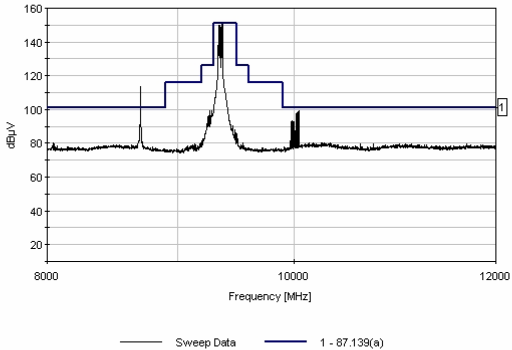
Figure 11-16 Spurious Emissions at Antenna Port (Fundamental)
