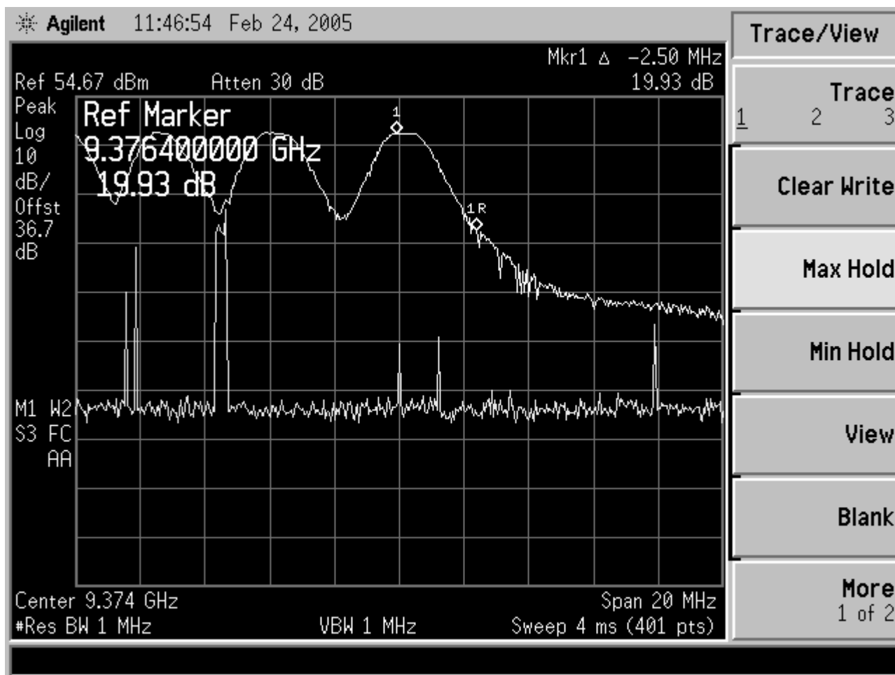
Figure 11-59 Frequency Stability, 170 Vdc Upper Edge @ -40C
