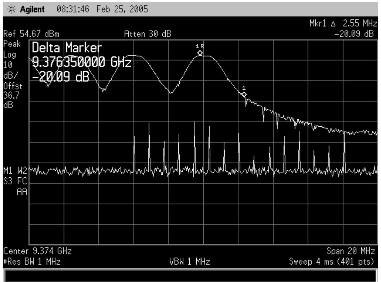
Figure 11-64 Frequency Stability, 170 Vdc Upper Edge @ +10C
