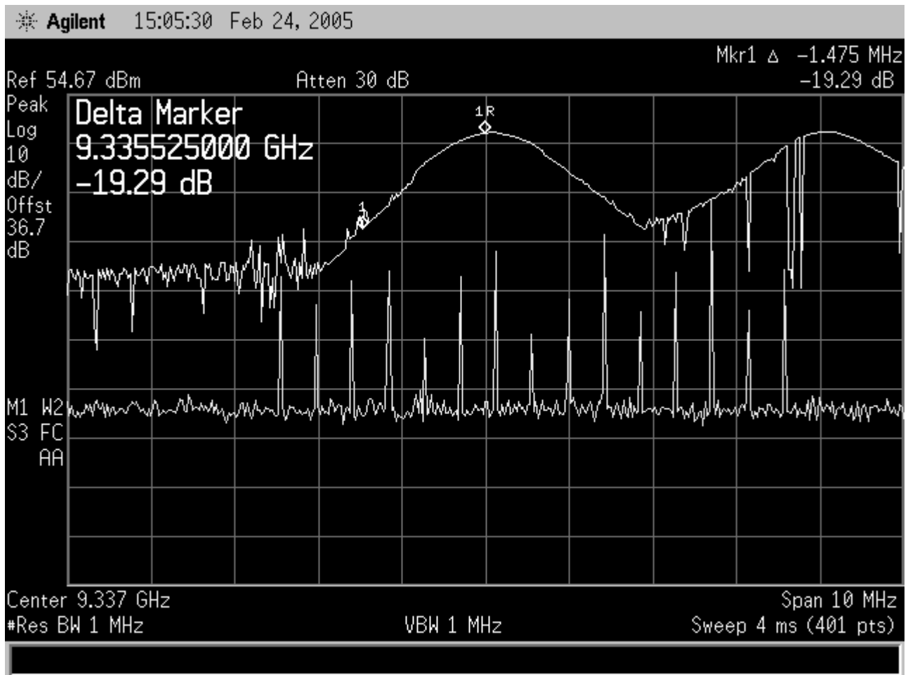
Figure 11-51 Frequency Stability, 170 Vdc Lower Edge @ -10C
