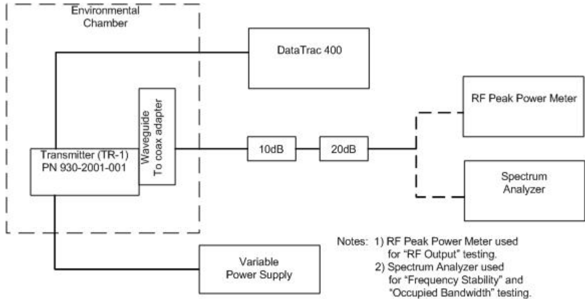
Figure 11-1 Configuration Setup
