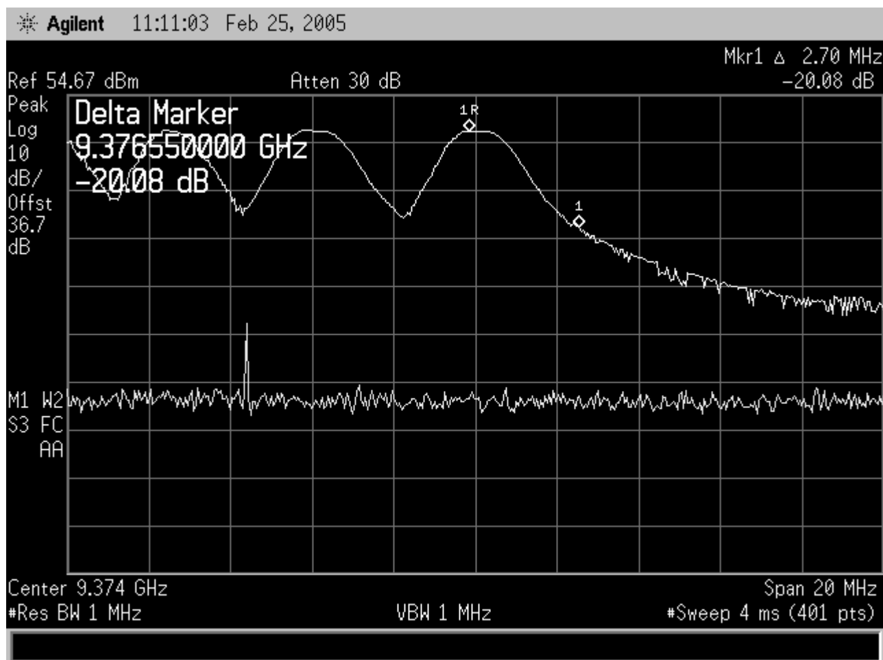
Figure 11-45 Frequency Stability, Upper Edge @ +40C
