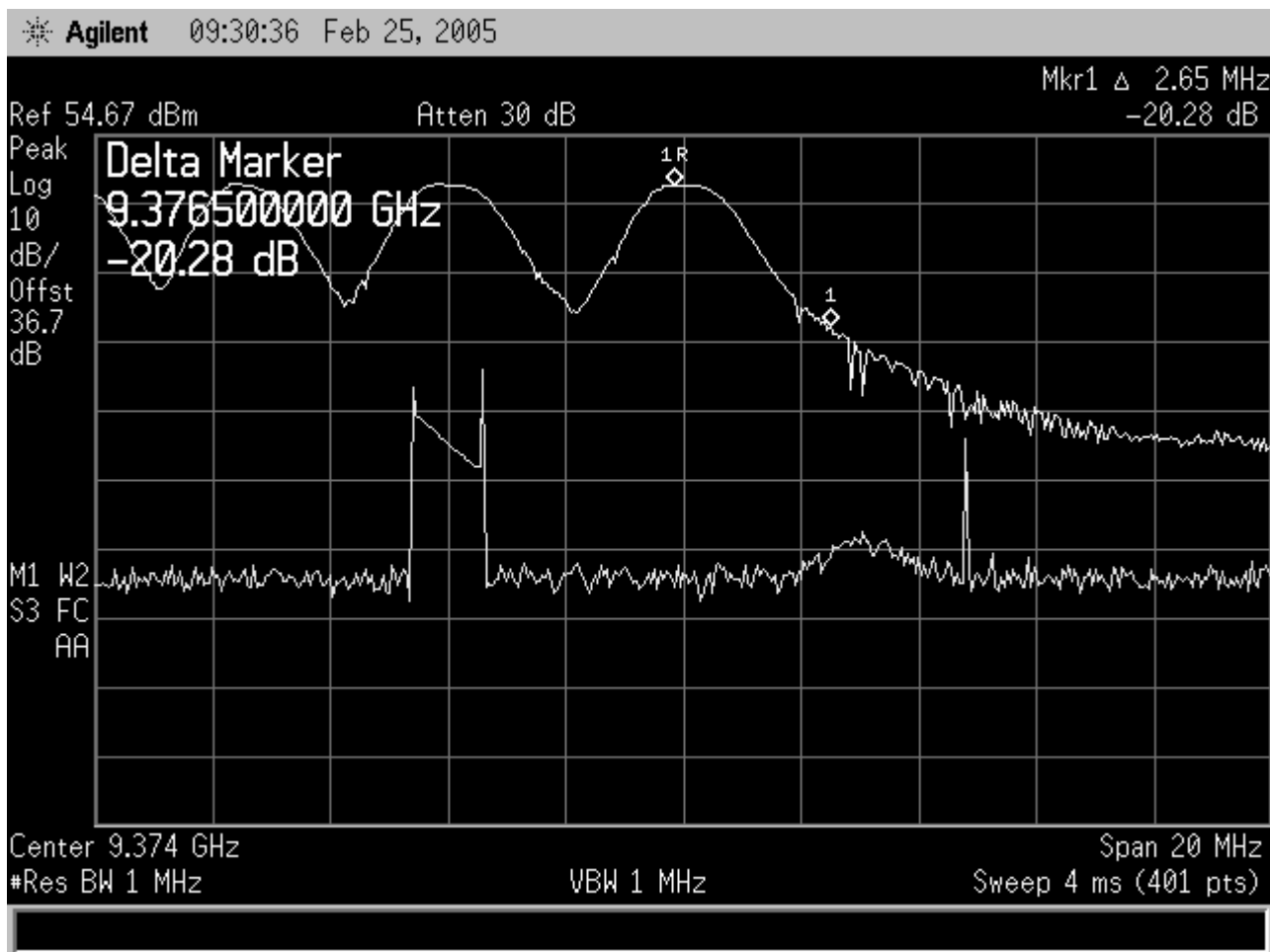
Figure 11-43 Frequency Stability, Upper Edge @ +20C
