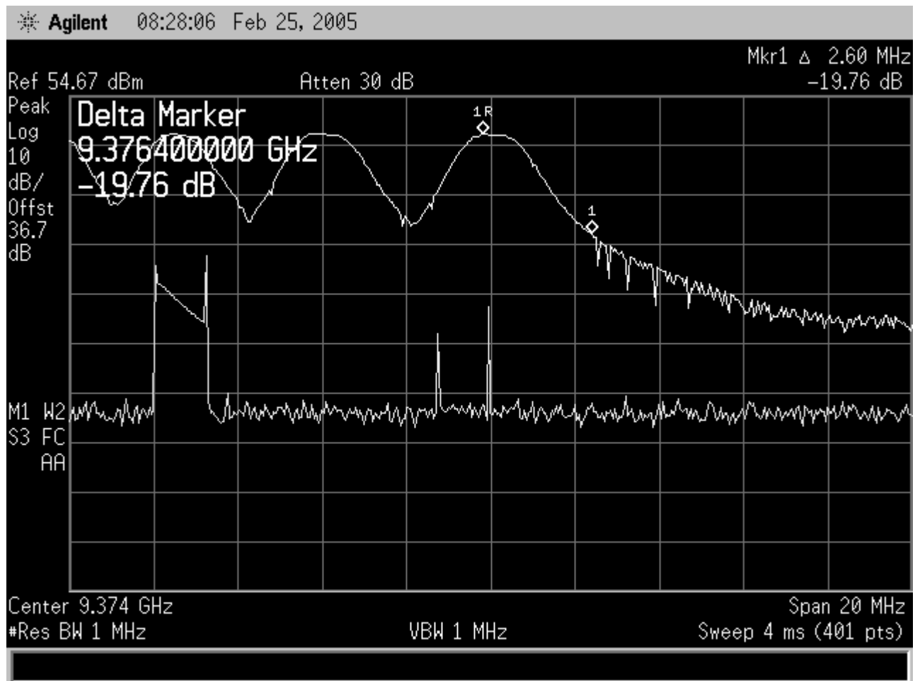
Figure 11-86 Frequency Stability, 230 Vdc Upper Edge @ +10C
