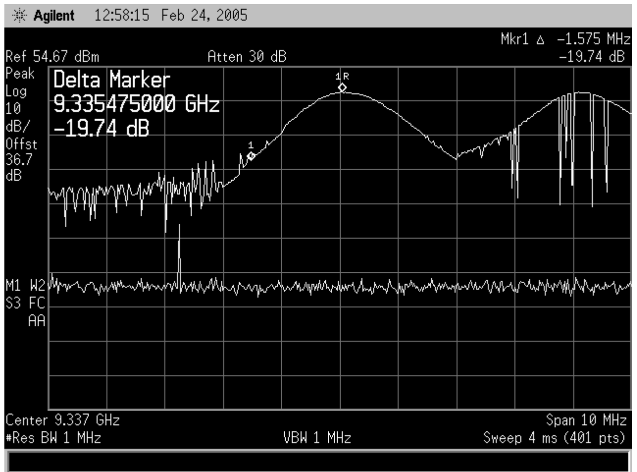
Figure 11-49 Frequency Stability, 170 Vdc Lower Edge @ -30C
