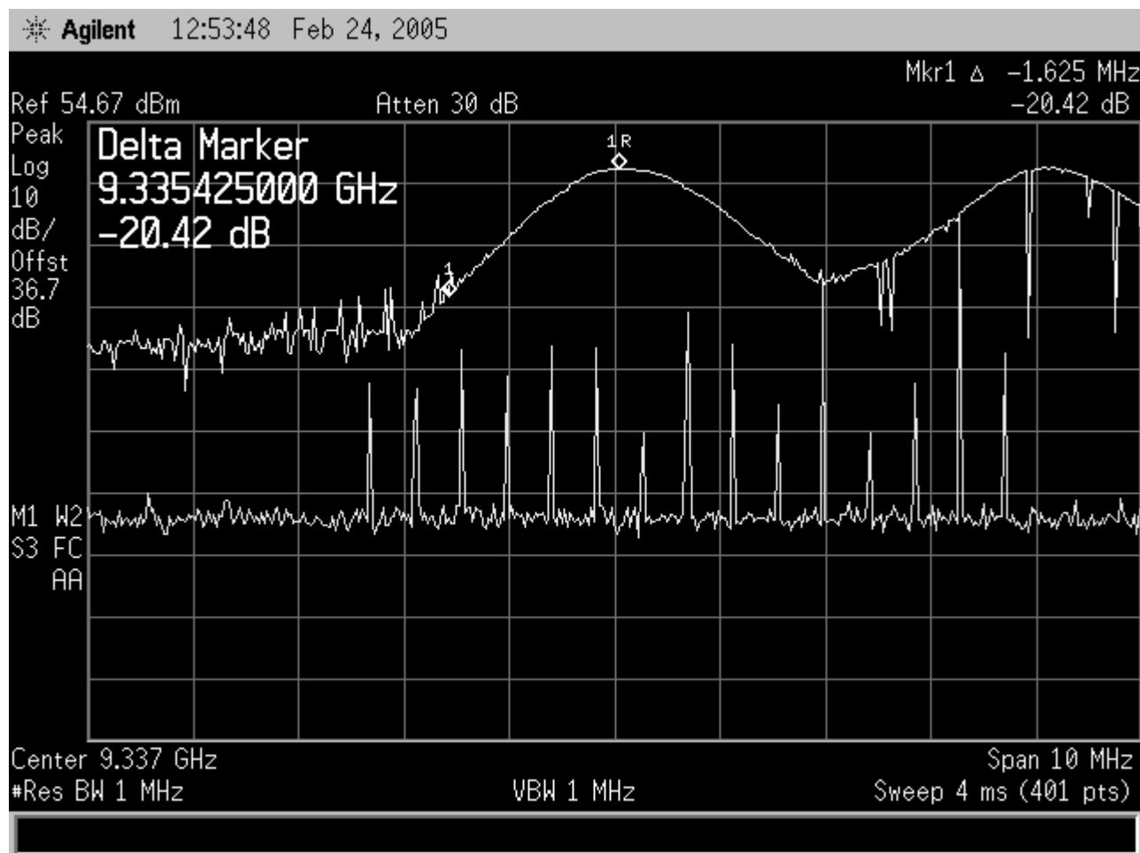
Figure 11-71 Frequency Stability, 230 Vdc Lower Edge @ -30C
