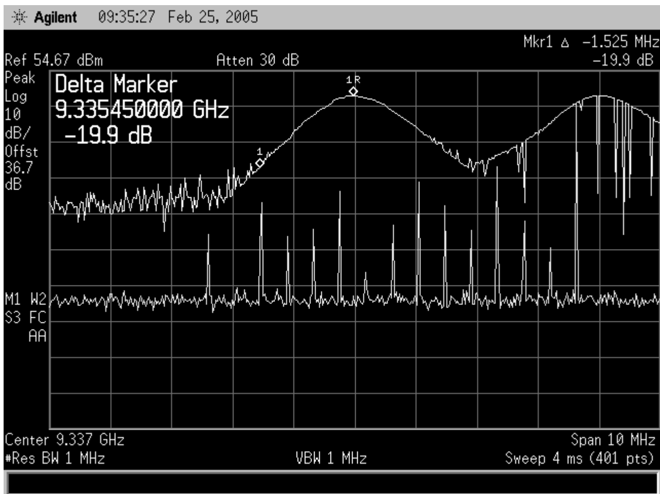
Figure 11-32 Frequency Stability, Lower Edge @ +20C
