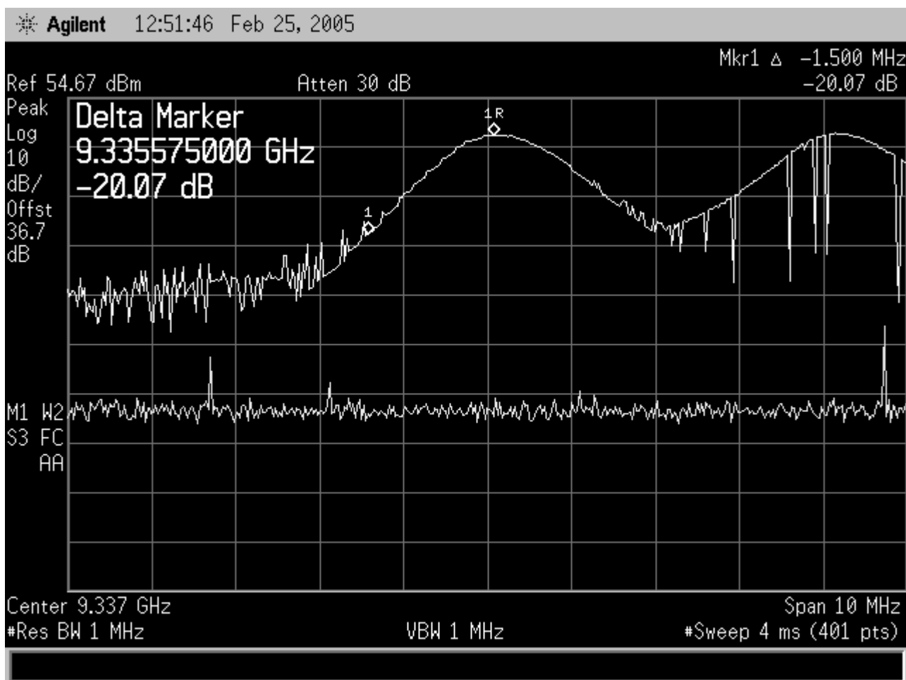
Figure 11-36 Frequency Stability, Lower Edge @ +60C
