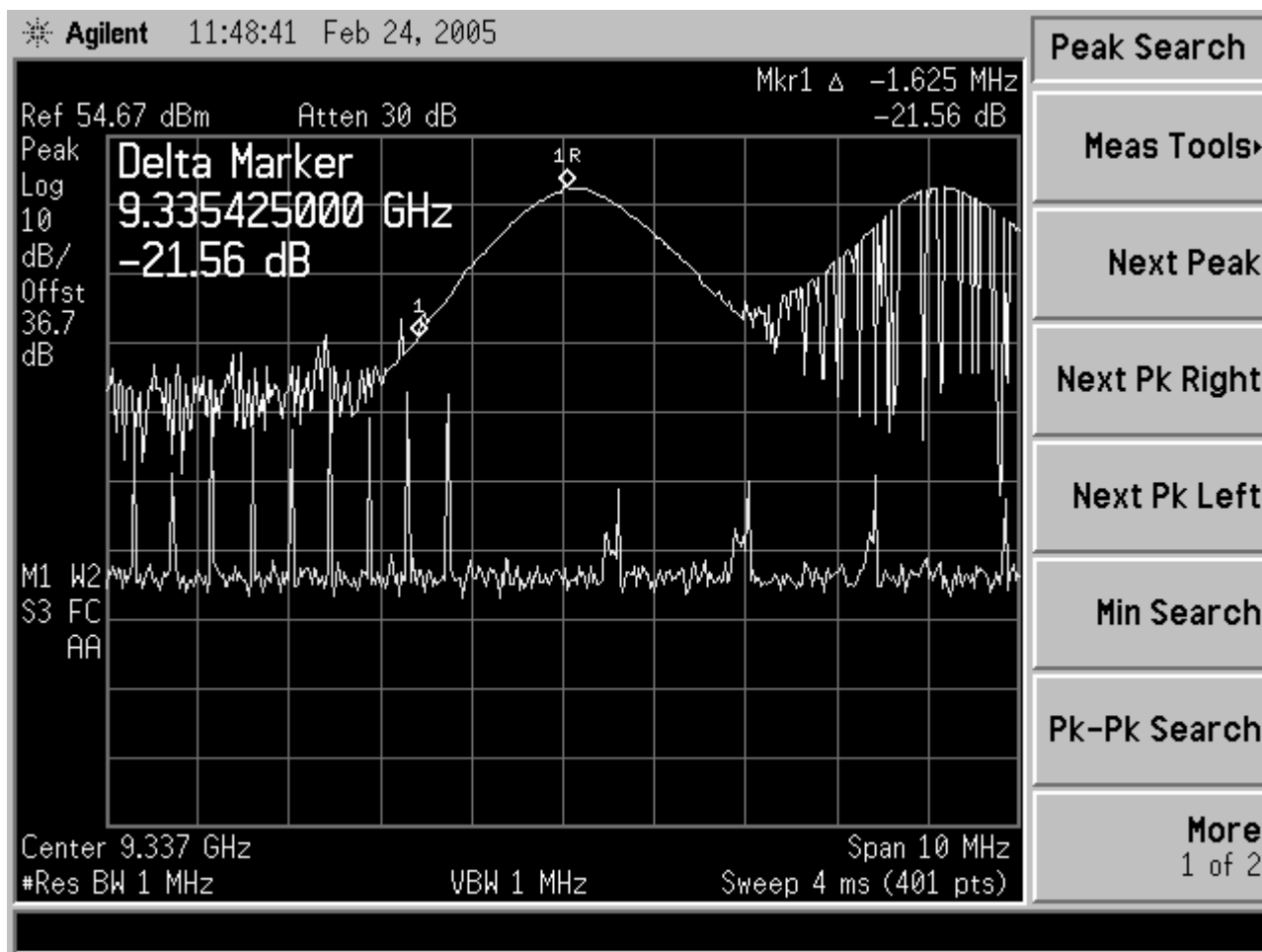
Figure 11-48 Frequency Stability, 170 Vdc Lower Edge @ -40C
