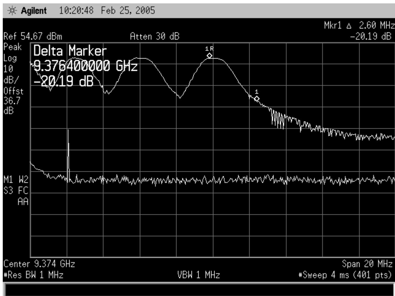
Figure 11-66 Frequency Stability, 170 Vdc Upper Edge @ +30C
