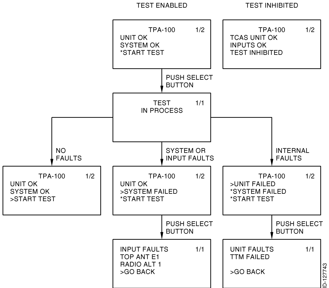
Start Test/Test Inhibited Sample Flow Diagram Figure 1004
