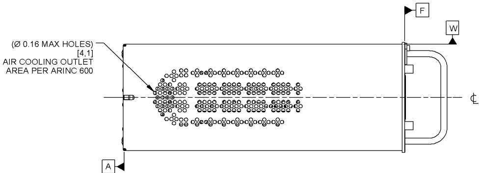
TPA-100A TCAS Processor Outline Drawing Figure 2006 (Sheet 1 of 2)
