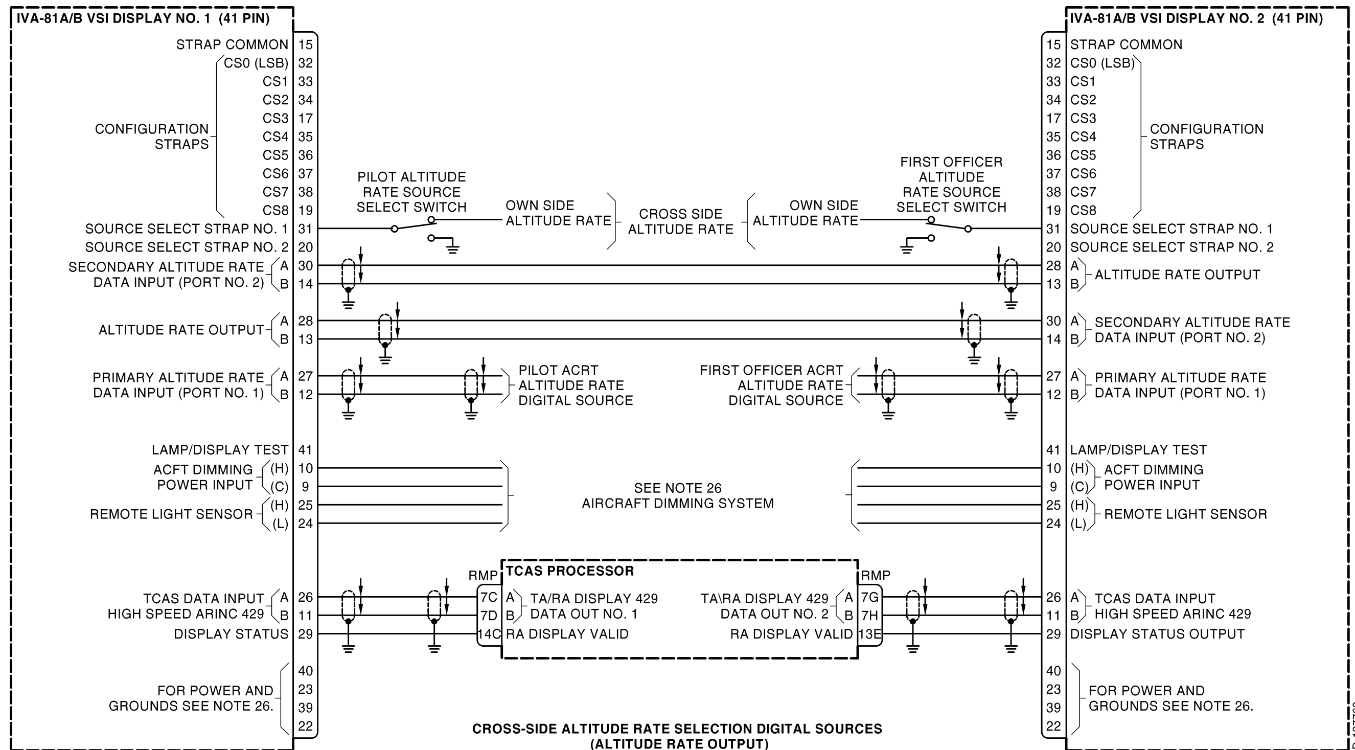
CAS-100 Interwiring Diagram Figure 2015 (Sheet 8 of 16)
