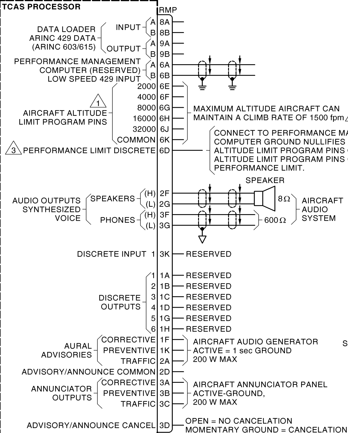
CAS-100 Interwiring Diagram Figure 2015 (Sheet 3 of 16)
