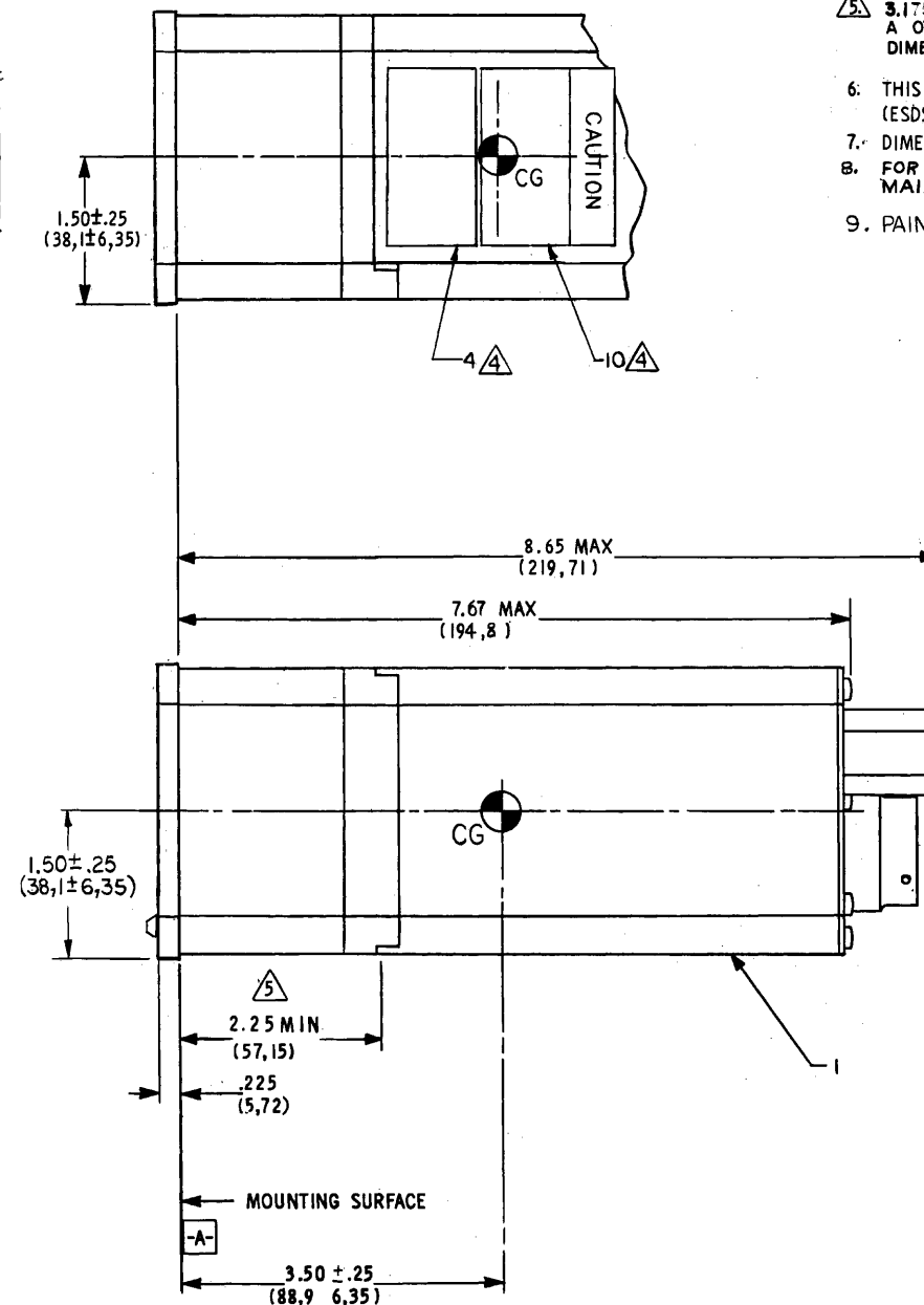
IVA-81B Resolution Advisory/Vertical Speed Indicator (RA/VS) Outline Drawing Figure 1012
