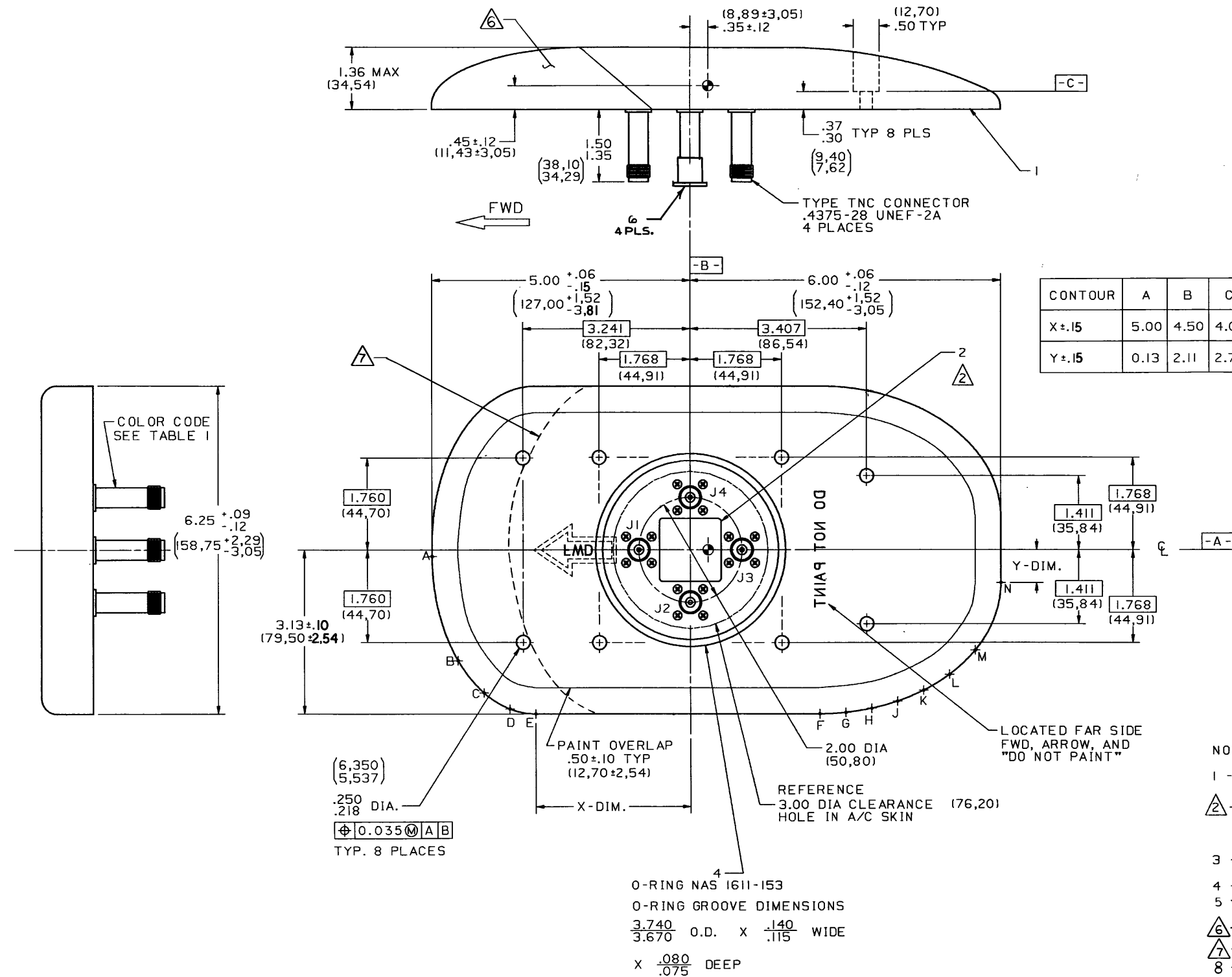
ANT-81A Directional Antenna (Four-Element Array, Flat Base, Four Mounting Screws) Outline Drawing Figure 2008
