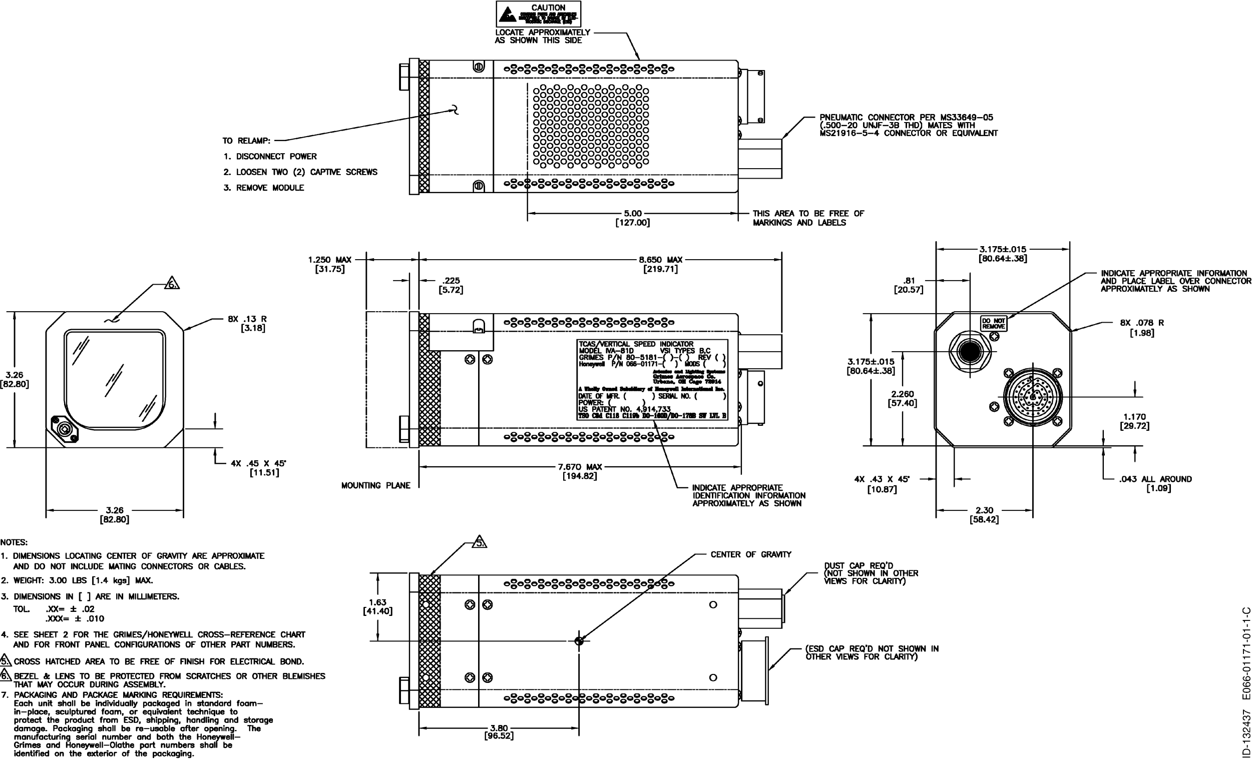
IVA-81D Traffic Advisory/Vertical Speed Indicator (TA/VS) Outline Drawing Figure 1013 (Sheet 1 of 2)
