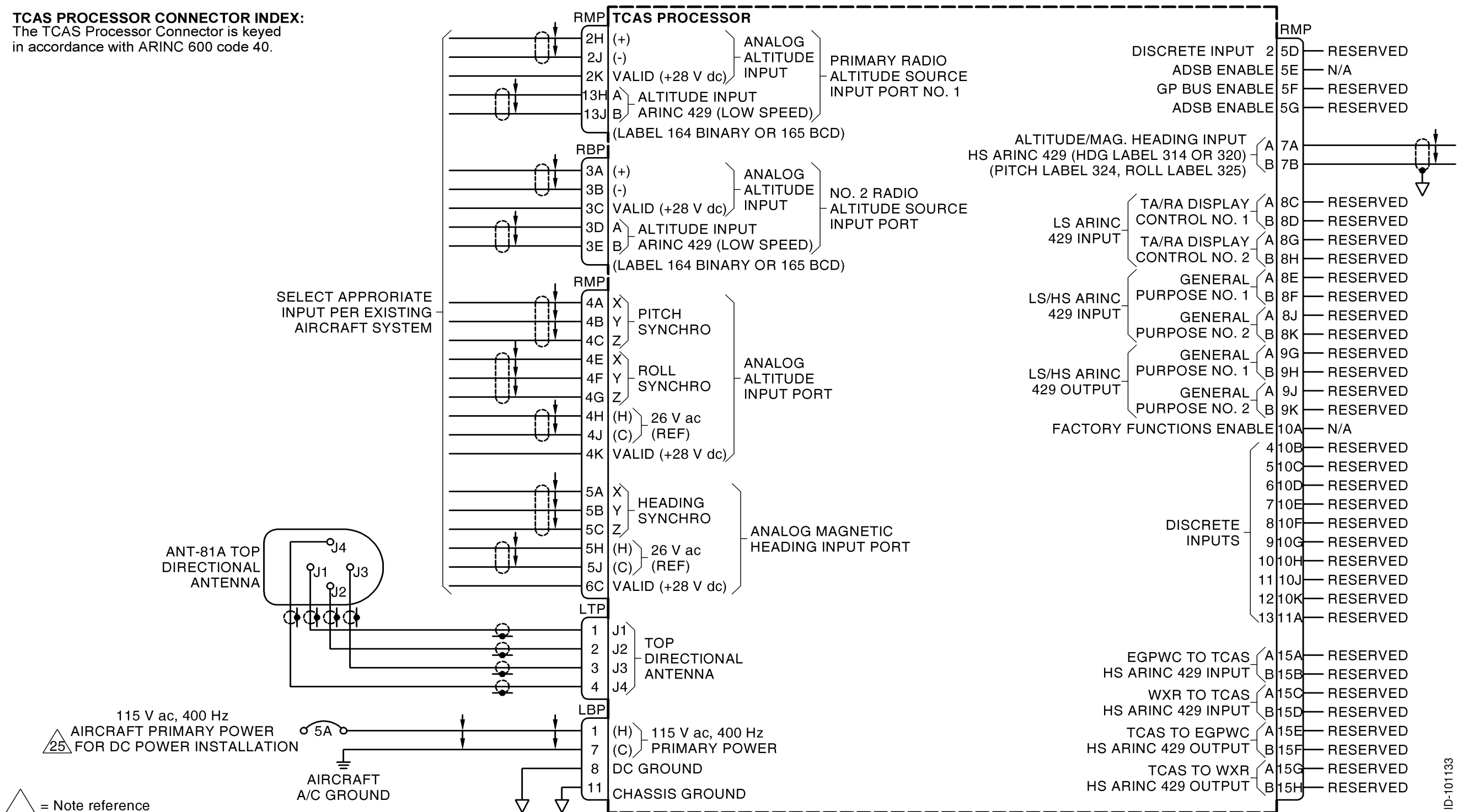
CAS-100 Interwiring Diagram Figure 2015 (Sheet 1 of 16)
