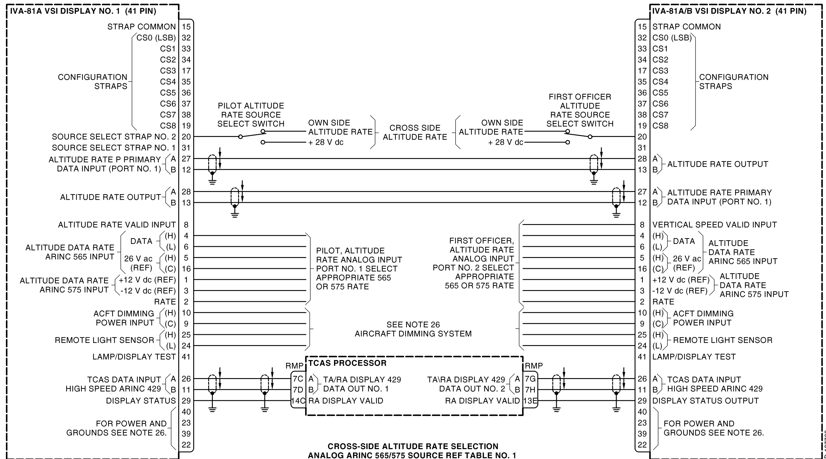
CAS-100 Interwiring Diagram Figure 2015 (Sheet 7 of 16)
