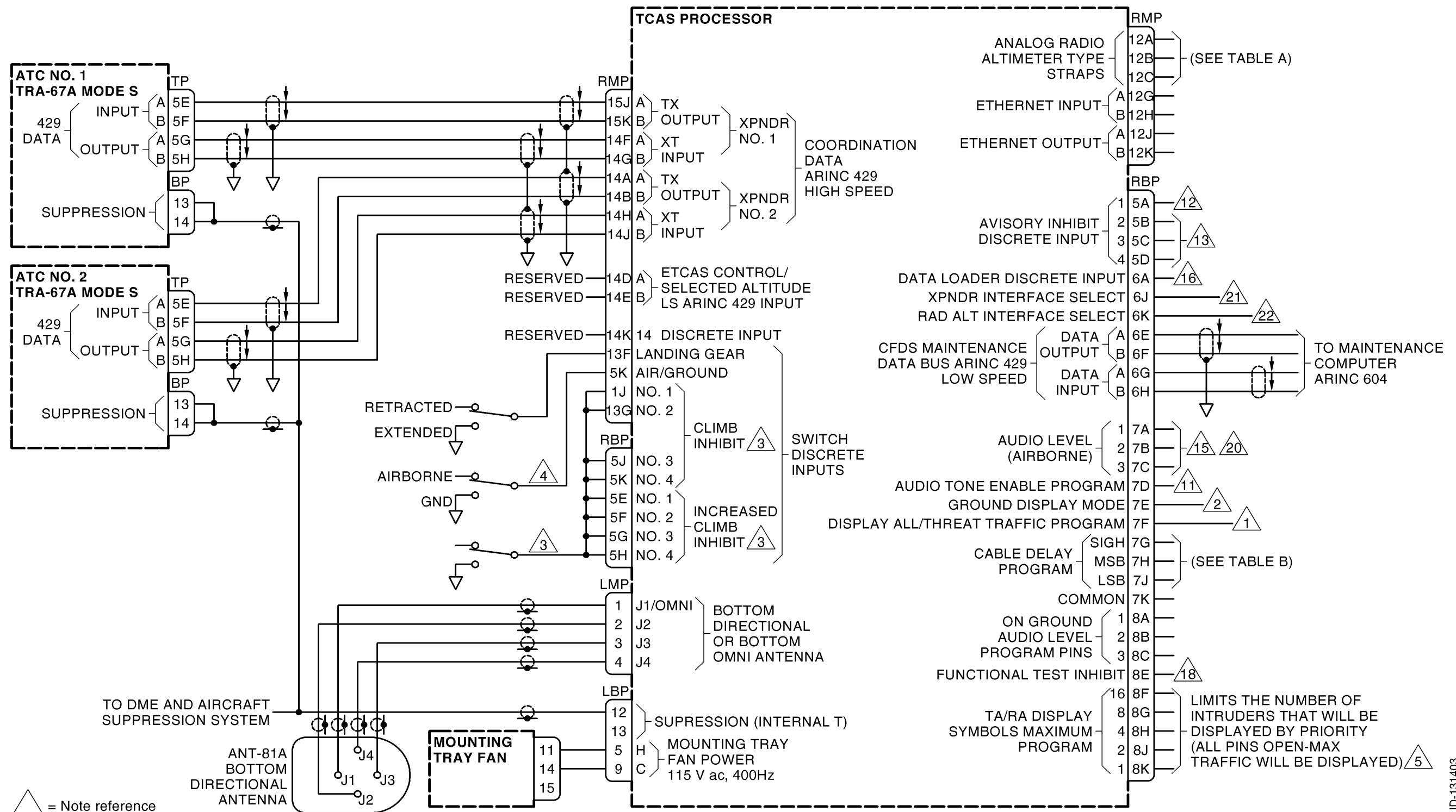
CAS-100 Interwiring Diagram Figure 2015 (Sheet 2 of 16)
