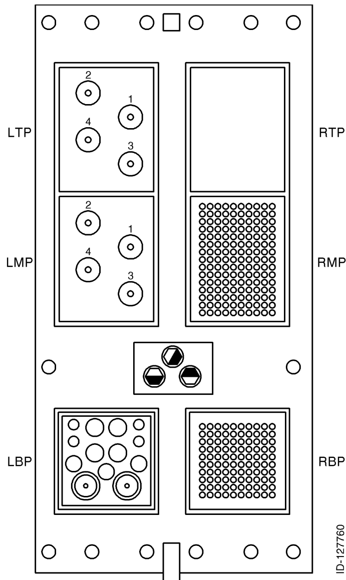
TPA-100A TCAS Processor Aft Connector Figure 2001 (Sheet 1 of 2)
