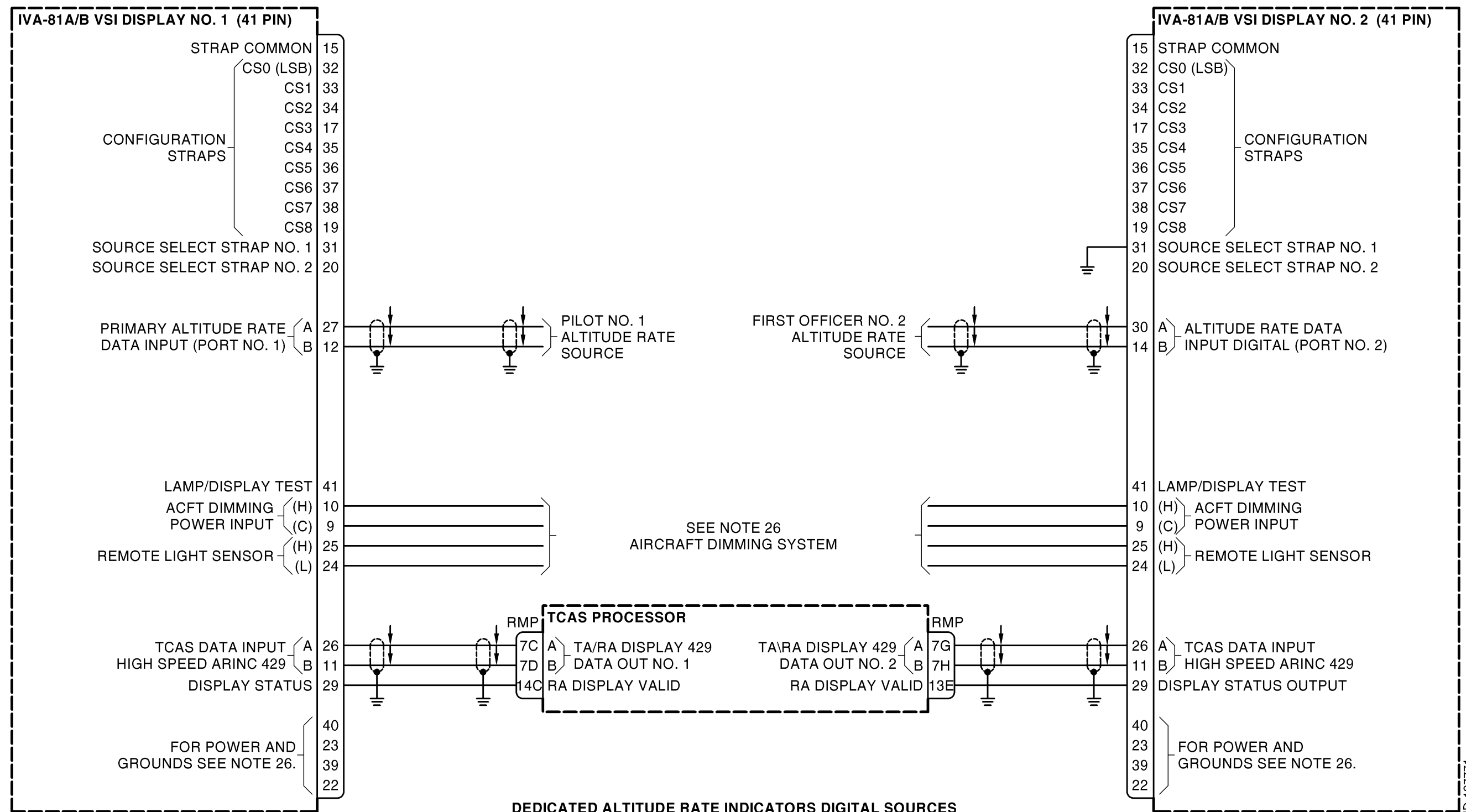
CAS-100 Interwiring Diagram Figure 2015 (Sheet 10 of 16)
