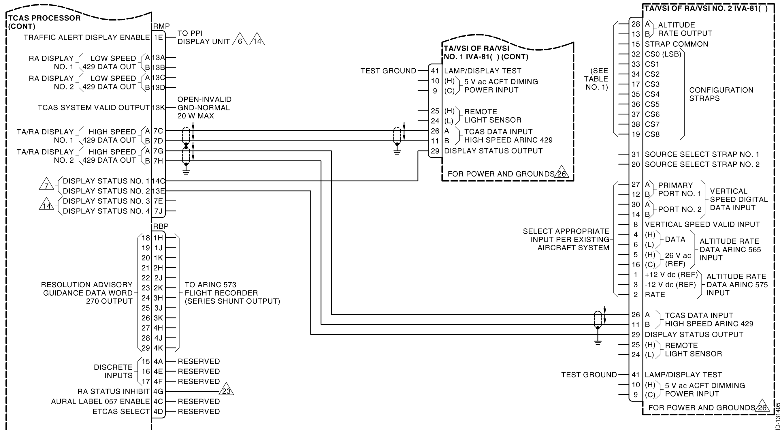
CAS-100 Interwiring Diagram Figure 2015 (Sheet 4 of 16)
