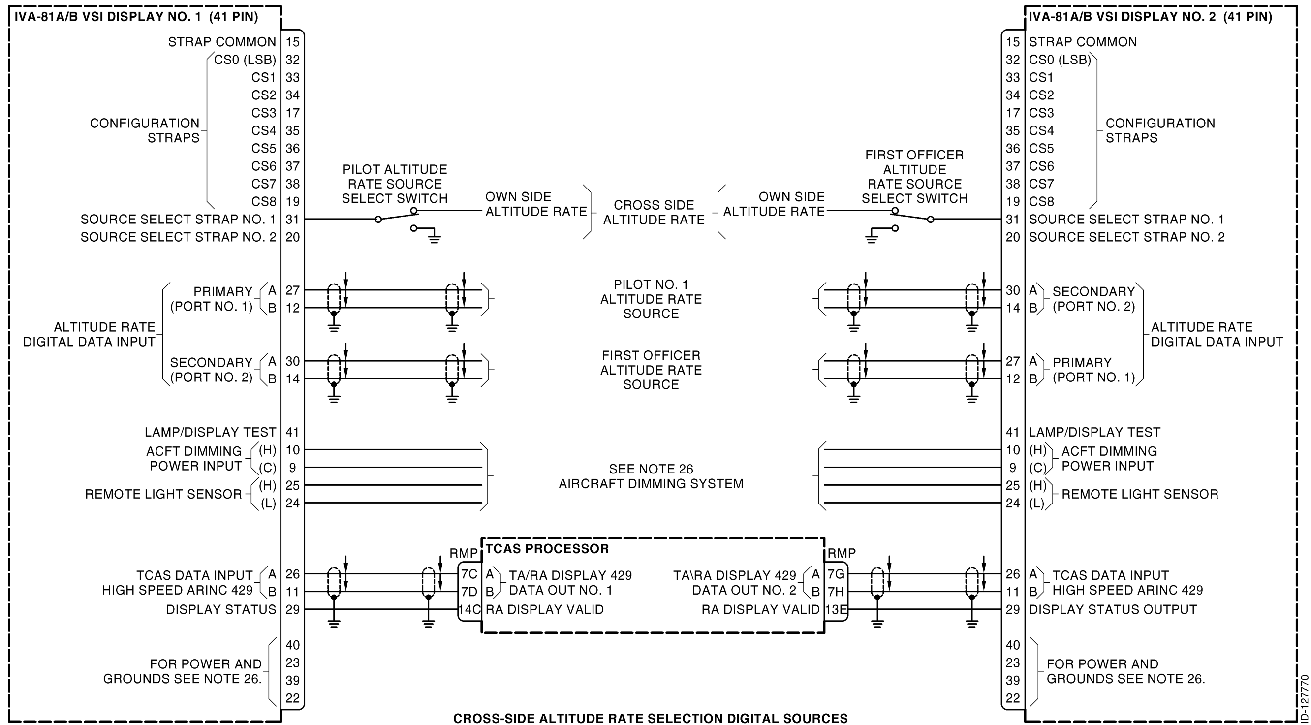
CAS-100 Interwiring Diagram Figure 2015 (Sheet 9 of 16)
