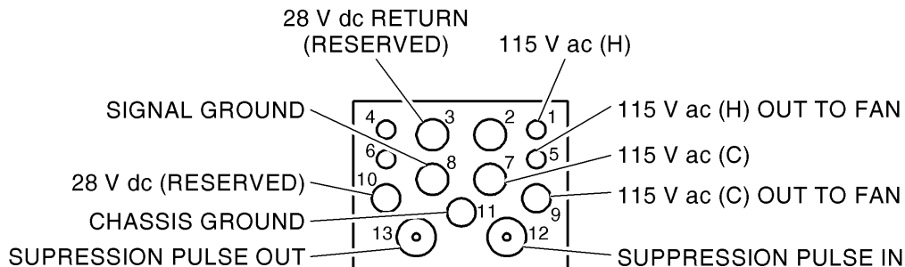
LEFT BOTTOM INSERT (LBP) CONNECTOR INSERT LAYOUT
