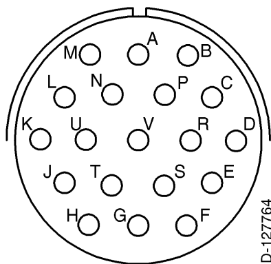
ITA-81A Aft Connector Figure 2004
