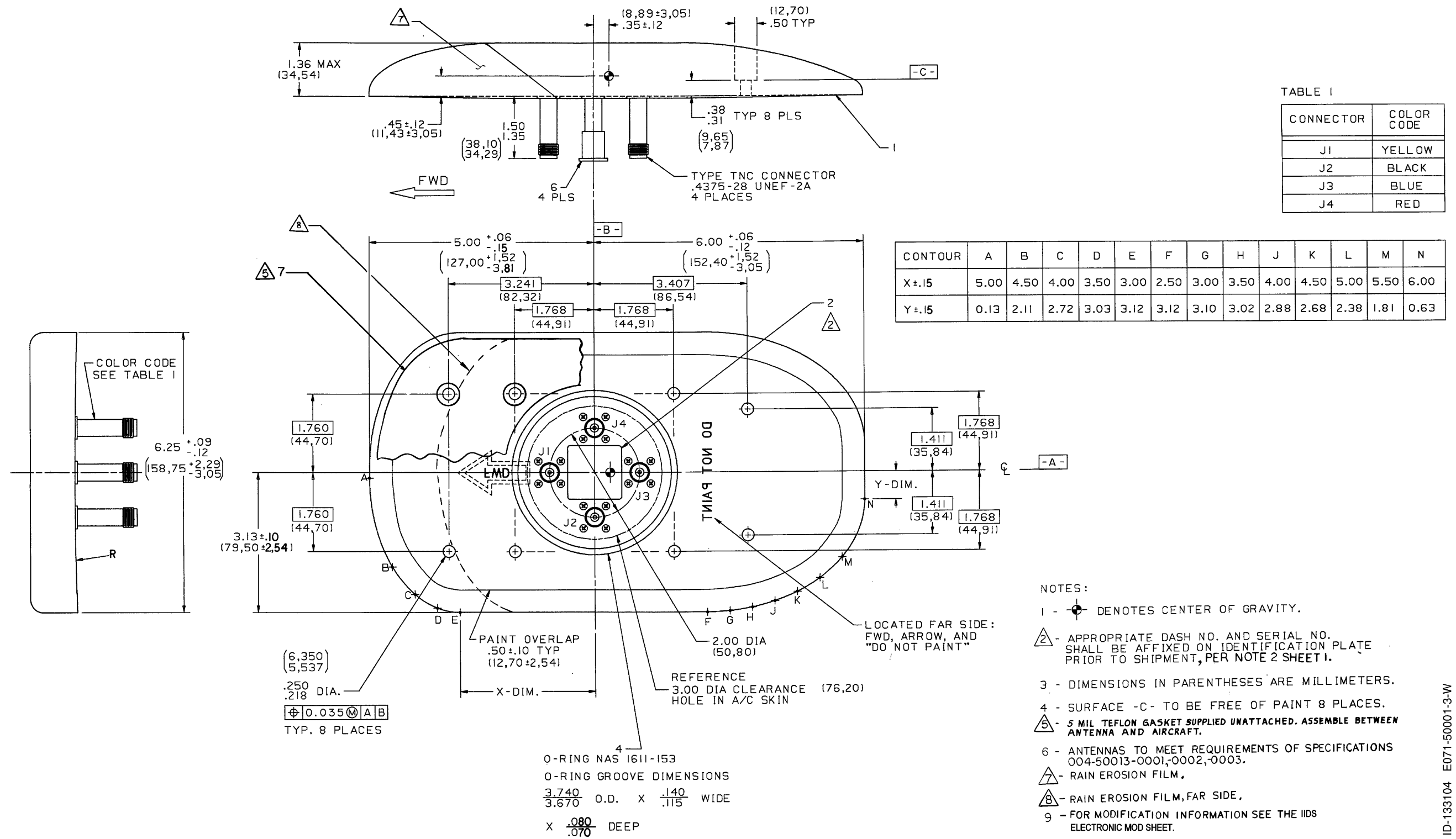
ANT-81A Directional Antenna (Four-Element Array, Flat Base, Eight Mounting Screws) Outline Drawing Figure 2009
