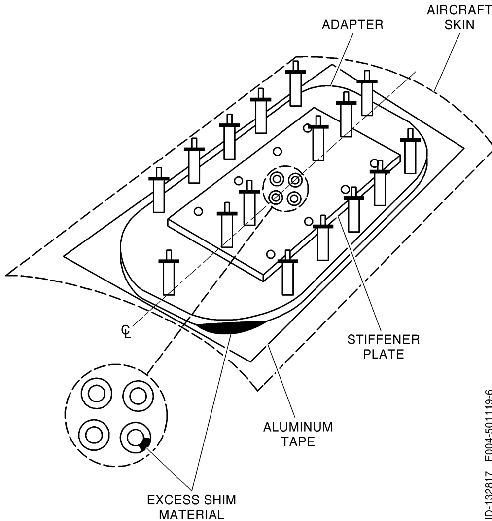
Adapter and Moldable Shim Assembled on the Airframe Figure 2005
