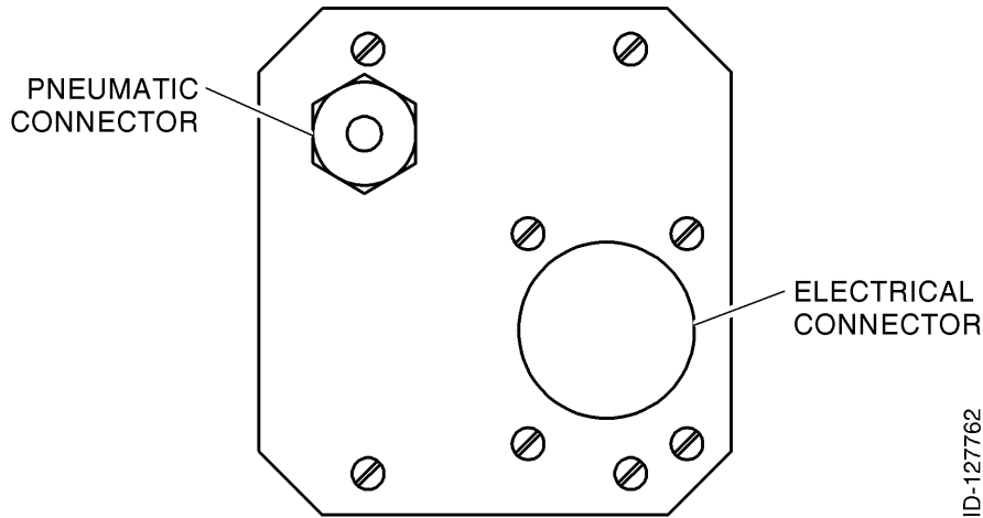
IVA-81A/D, TA/VSI and IVA-81B, RA/VSI Aft Connector Locations Figure 2002
