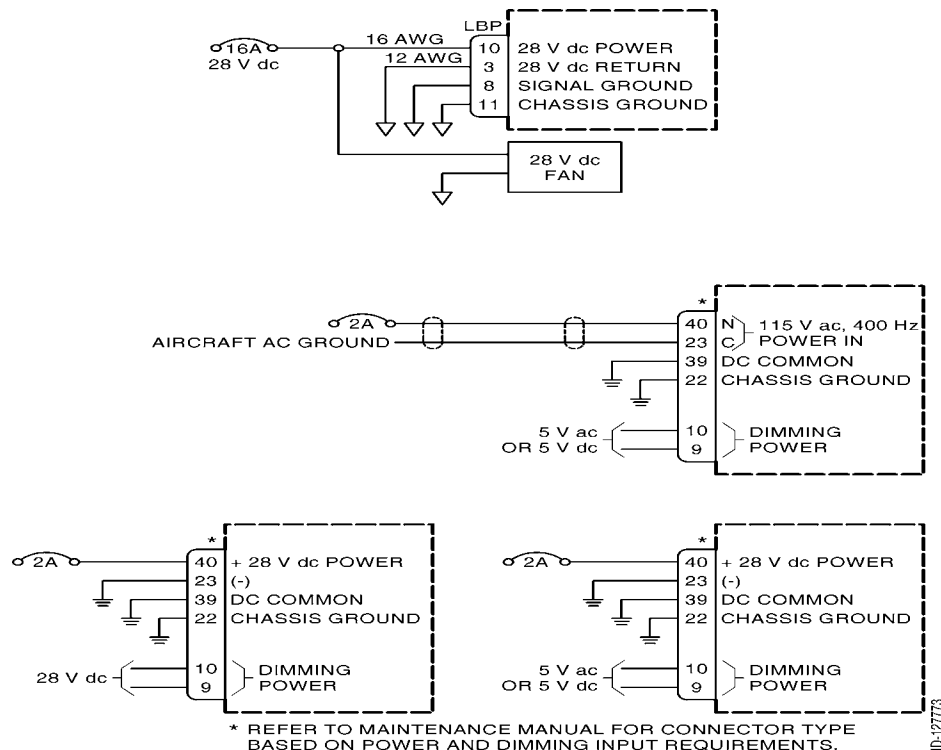
CAS-100 Interwiring Diagram Figure 2015 (Sheet 15 of 16)
