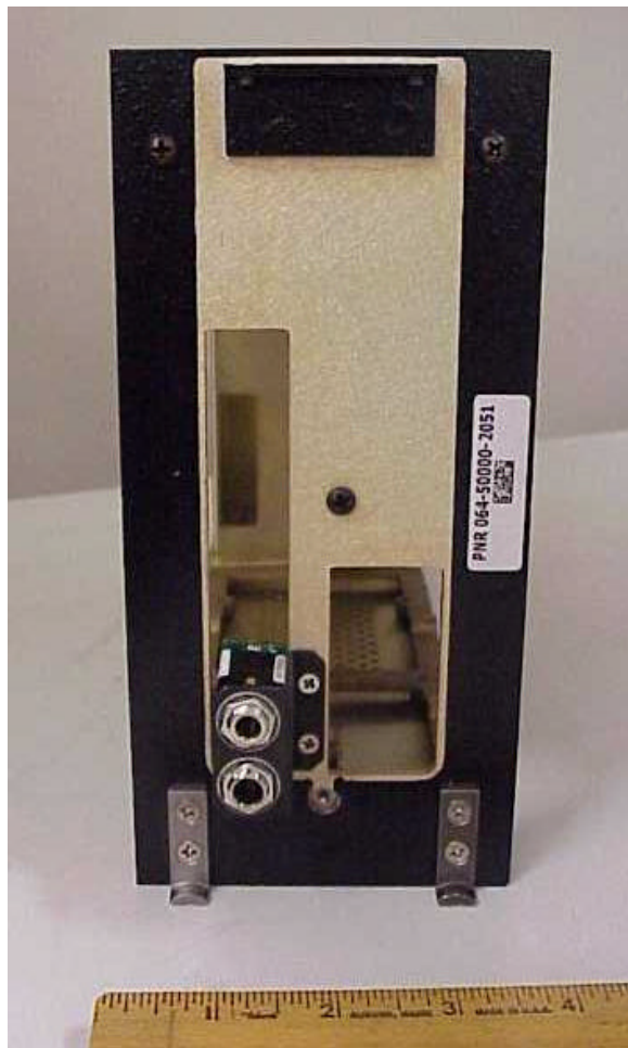
Front Panel Assembly with PCMCI card slot and RS232 covers removed, and then the Front panel assembly removed from LRU chassis.
