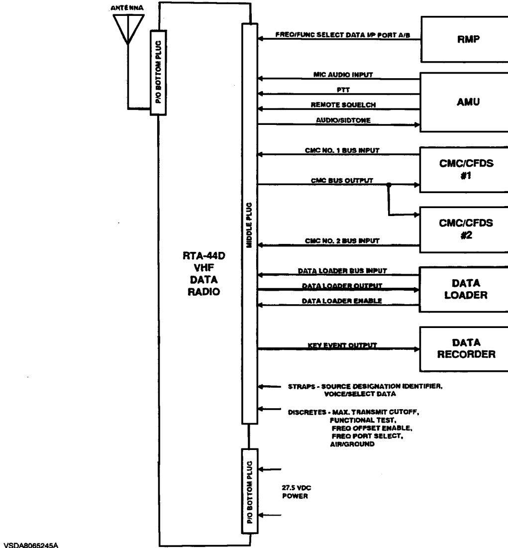
VHF Communications for Voice Operation Figure 10
