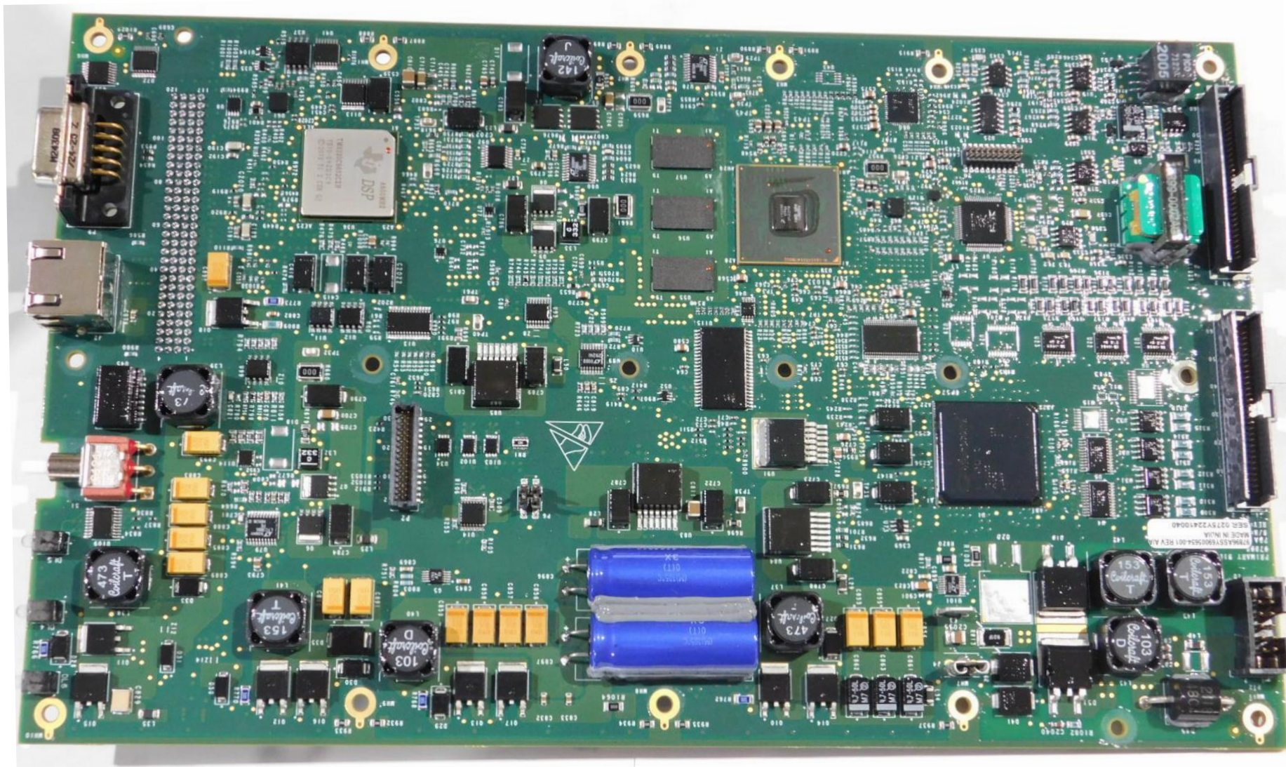
Processor PBA Side A
