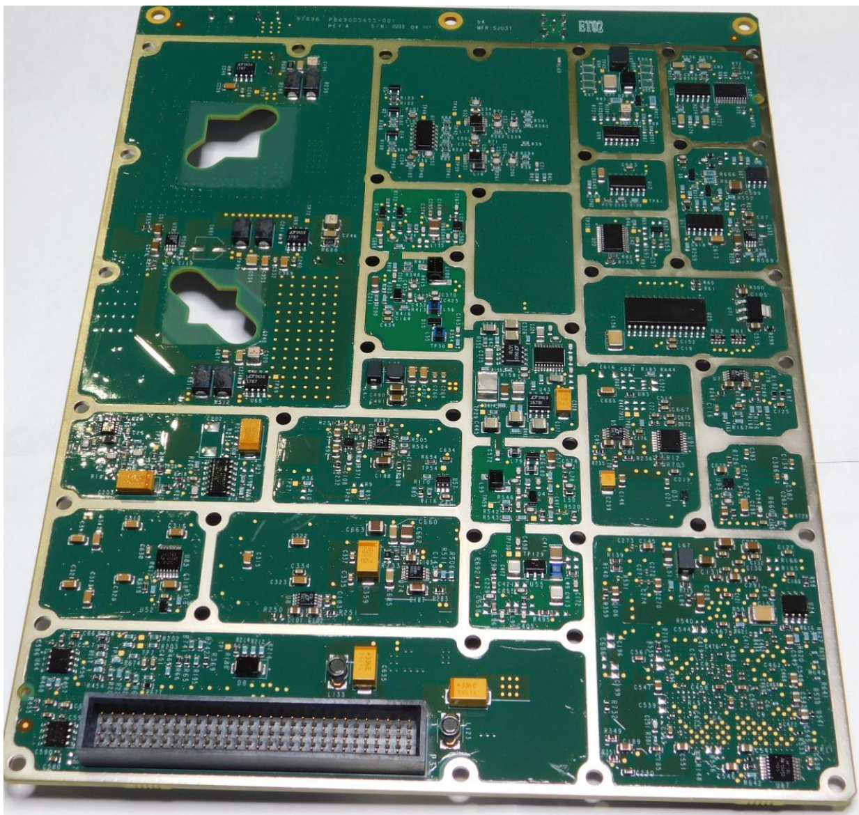
RF PBA Side B
