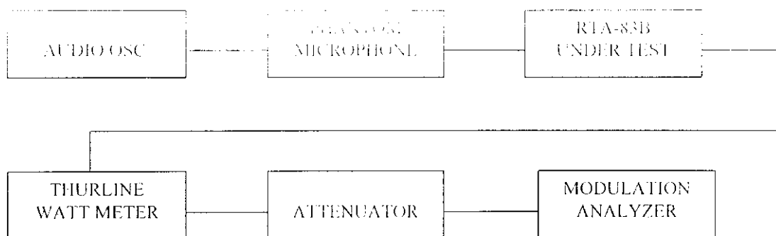
AM Modulation Characteristics Test Set-Up Figure 6
