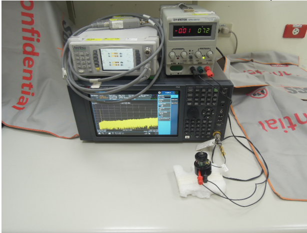
FCC 15 247_SRD_Radiated_RC-K3X-001HJ_Setup
