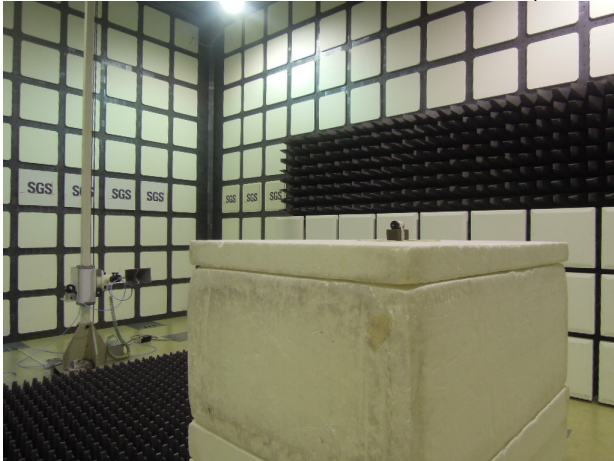
FCC 15 247_SRD_Radiated_RC-K3X-001HJ_Setup
