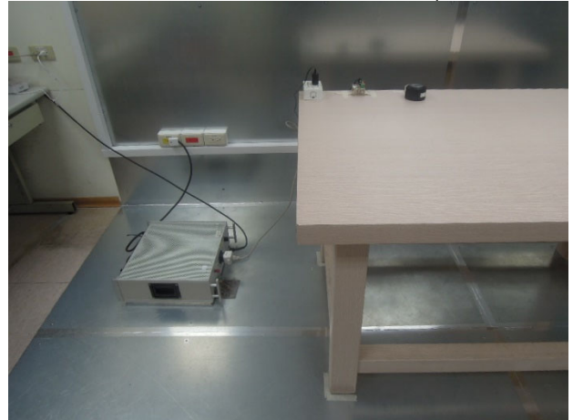
FCC_LP0002_SRD_Conduction_Setup
