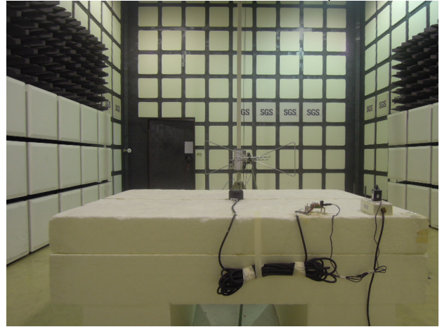
FCC_15_247_SRD_Radiated_Setup
