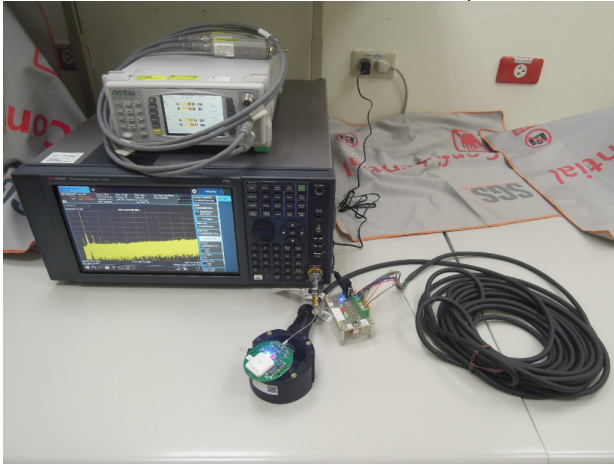
FCC_15_247_SRD_Radiated_Setup
