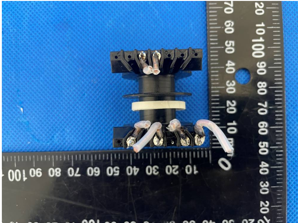
Figure 27. Transformer T901 view 5
