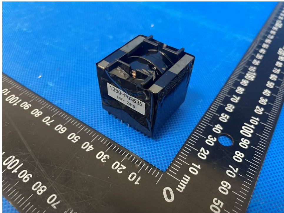
Figure 23. Transformer T901 view 1
