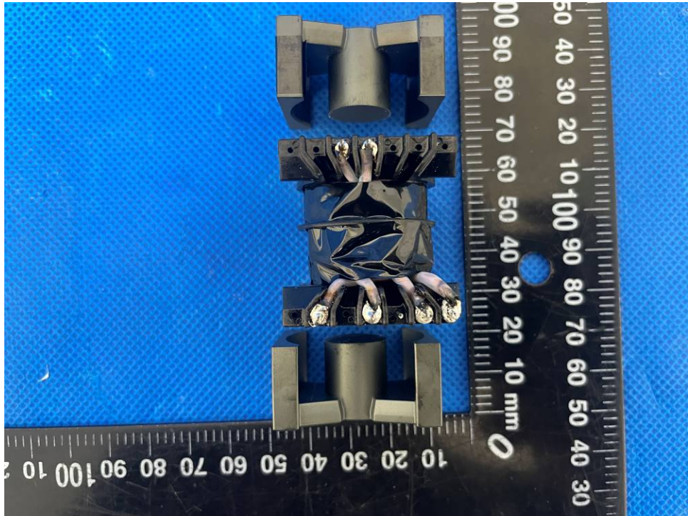
Figure 25. Transformer T901 view 3
