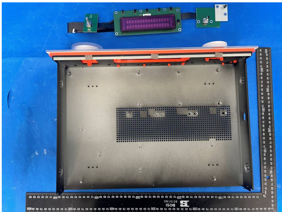
Figure 6. Internal view 6
