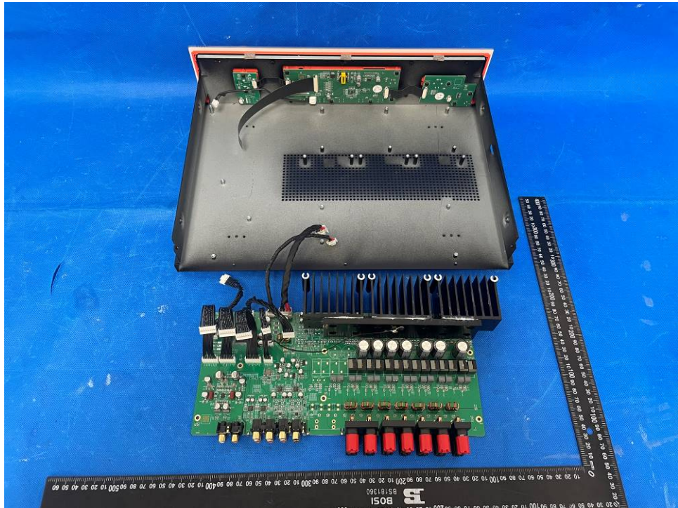
Figure 5. Internal view 5
