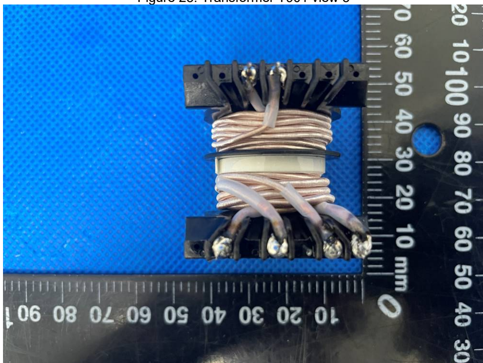
Figure 26. Transformer T901 view 4
