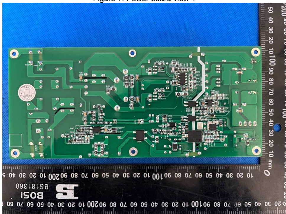
Figure 8. Power board view 2
