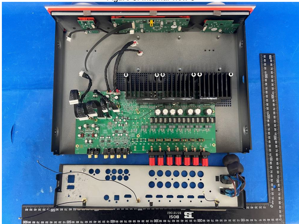
Figure 4. Internal view 4
