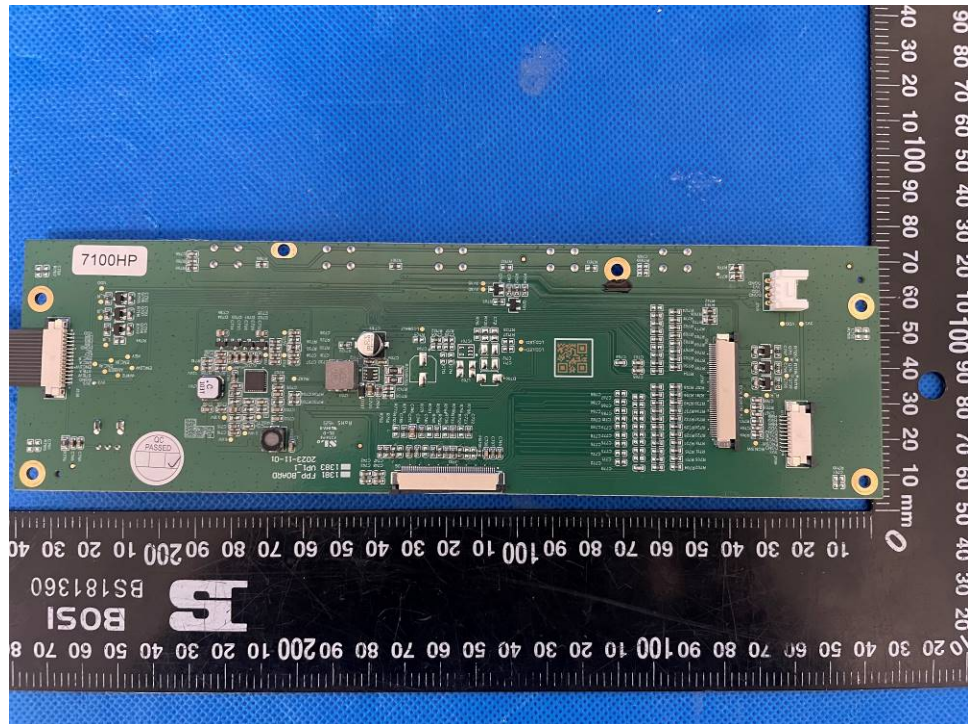
Figure 17. FPP board view 1
