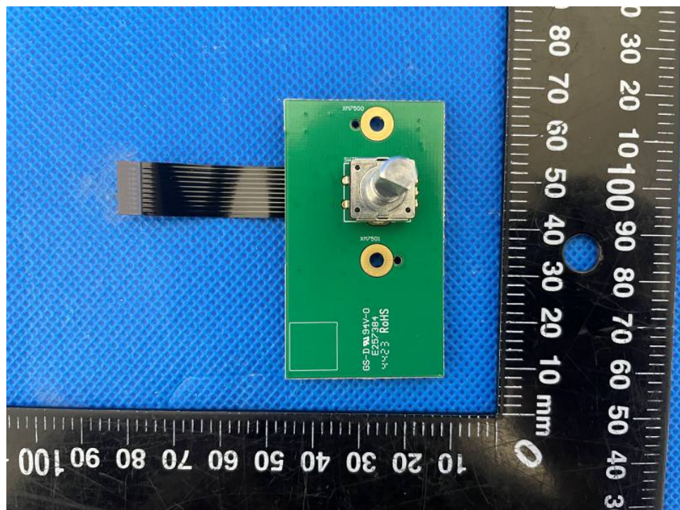
Figure 22. R EN board view 2
