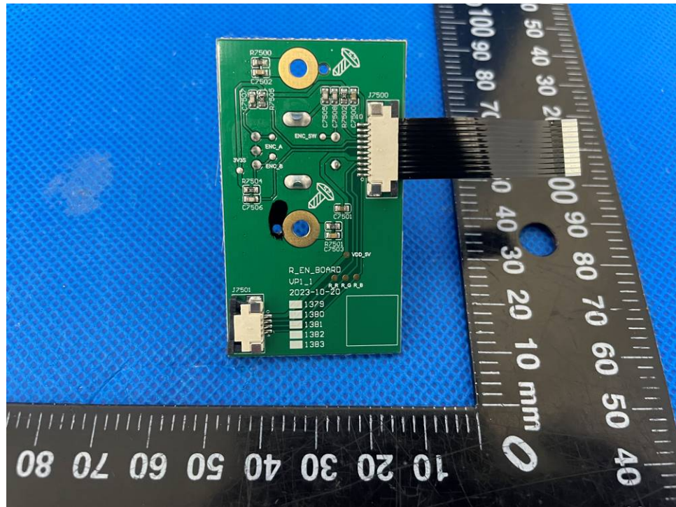
Figure 21. R EN board view 1
