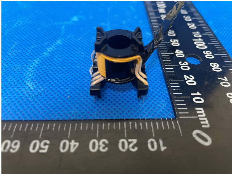
Figure 37. Transformer T901 view 9
