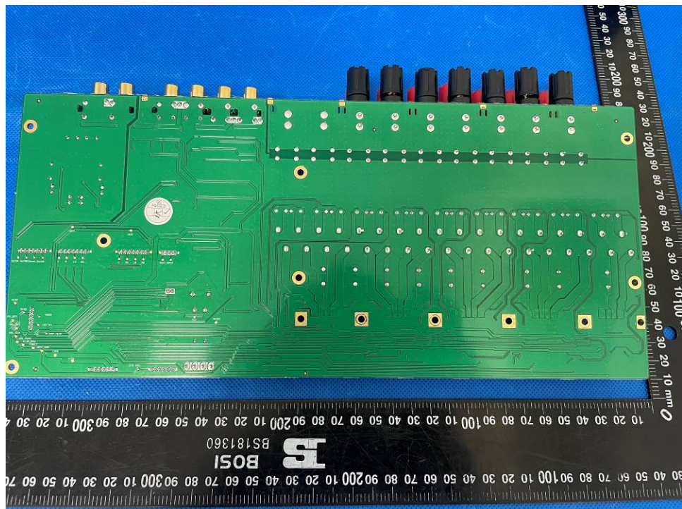
Figure 14. AMP board view 3
