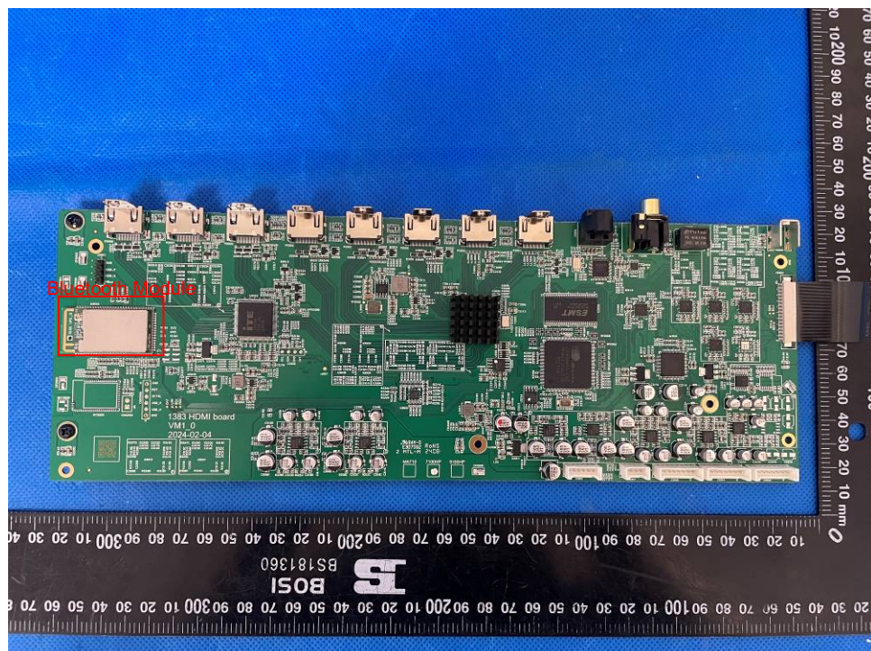
Figure 10 HDMI board view 1
