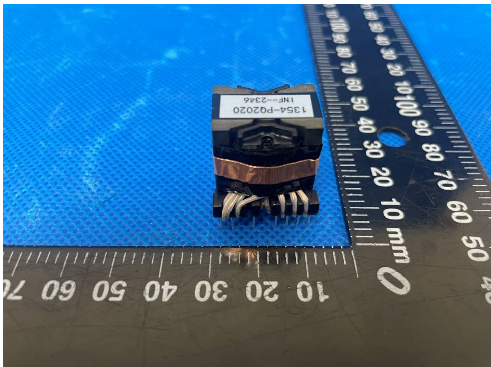
Figure 32. Transformer T901 view 4
