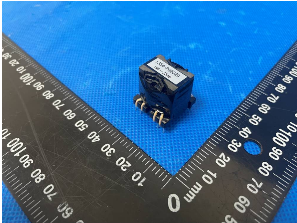
Figure 29. Transformer T901 view 1
