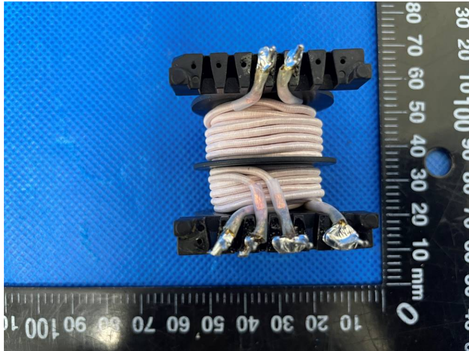
Figure 27. Transformer T900 view 4
