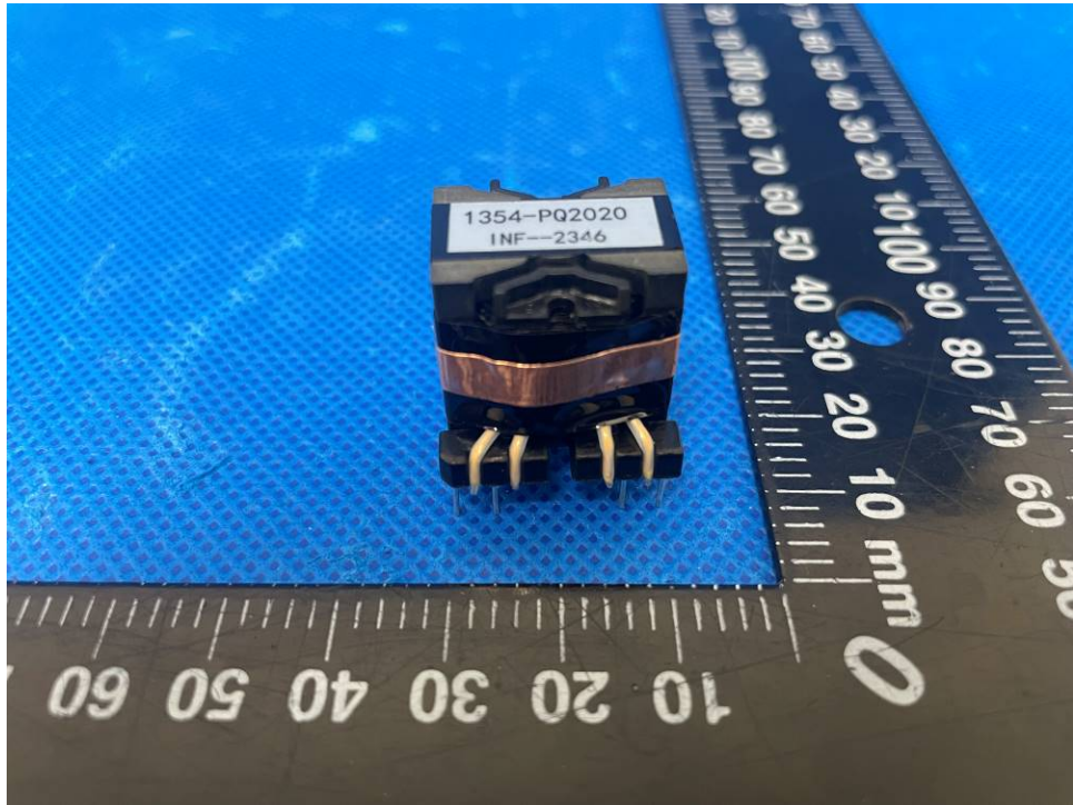
Figure 31. Transformer T901 view 3
