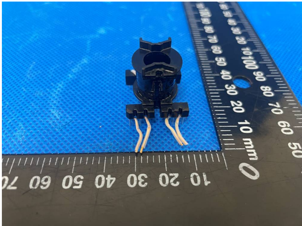
Figure 40. Transformer T901 view 12
