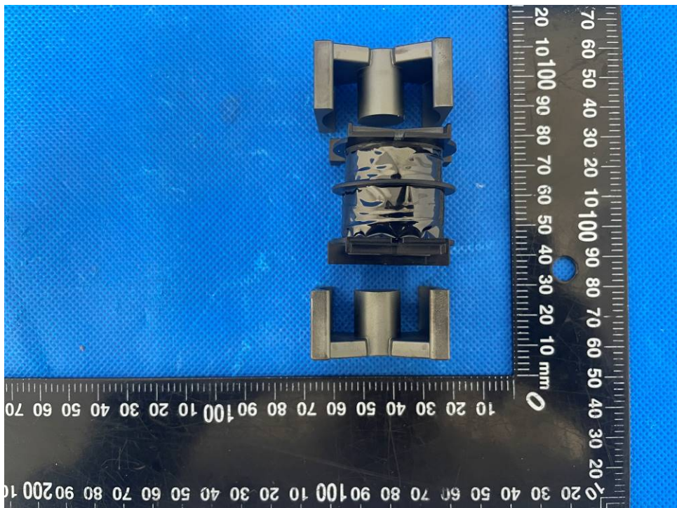
Figure 26. Transformer T900 view 3
